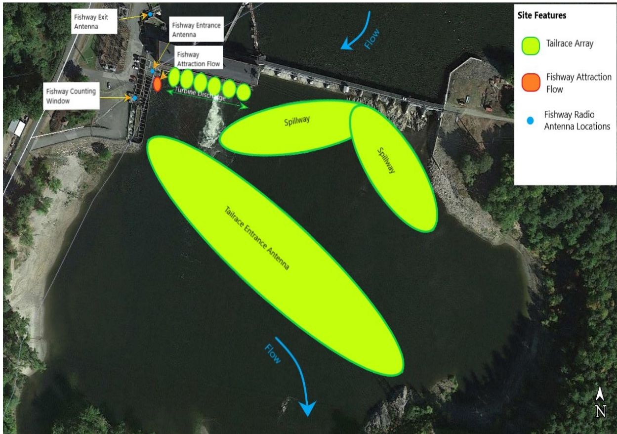
AIR 4, Figure 2. Detection zones for the Vernon tailrace array (tailrace entrance, spillway and turbine discharge antennas) and fishway monitoring stations used in 2015 as part of ILP Study 21 (American Shad Telemetry) and used in this assessment of FirstLight tagged sea lamprey movement at Vernon.
