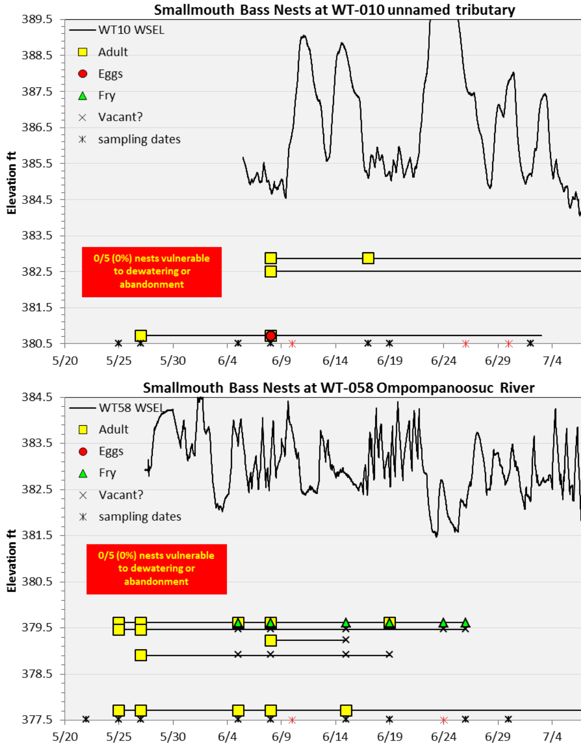
Figure 5.3-12. Smallmouth Bass (SB) nest elevations and backwater WSELs. Yellow squares represent nests with adults present; red circles represent eggs, green triangles represent fry, and "X's" are dates with no life-stages observed. Red dashed lines are vulnerable nests within 1.0 ft of WSE. Asterisks on x-axis are sampling dates, red asterisks are days with visibility <2ft.
