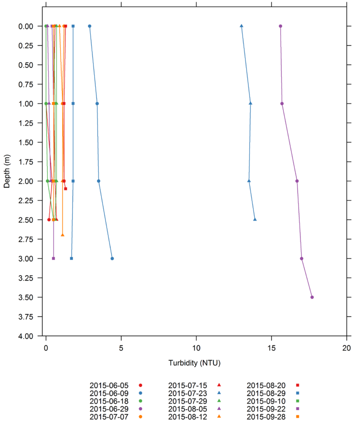
Figure H-42. Vertical profiles of NTU (NTU) collected at the Bellows Falls upper impoundment 06-BF-03 water quality monitoring station.
