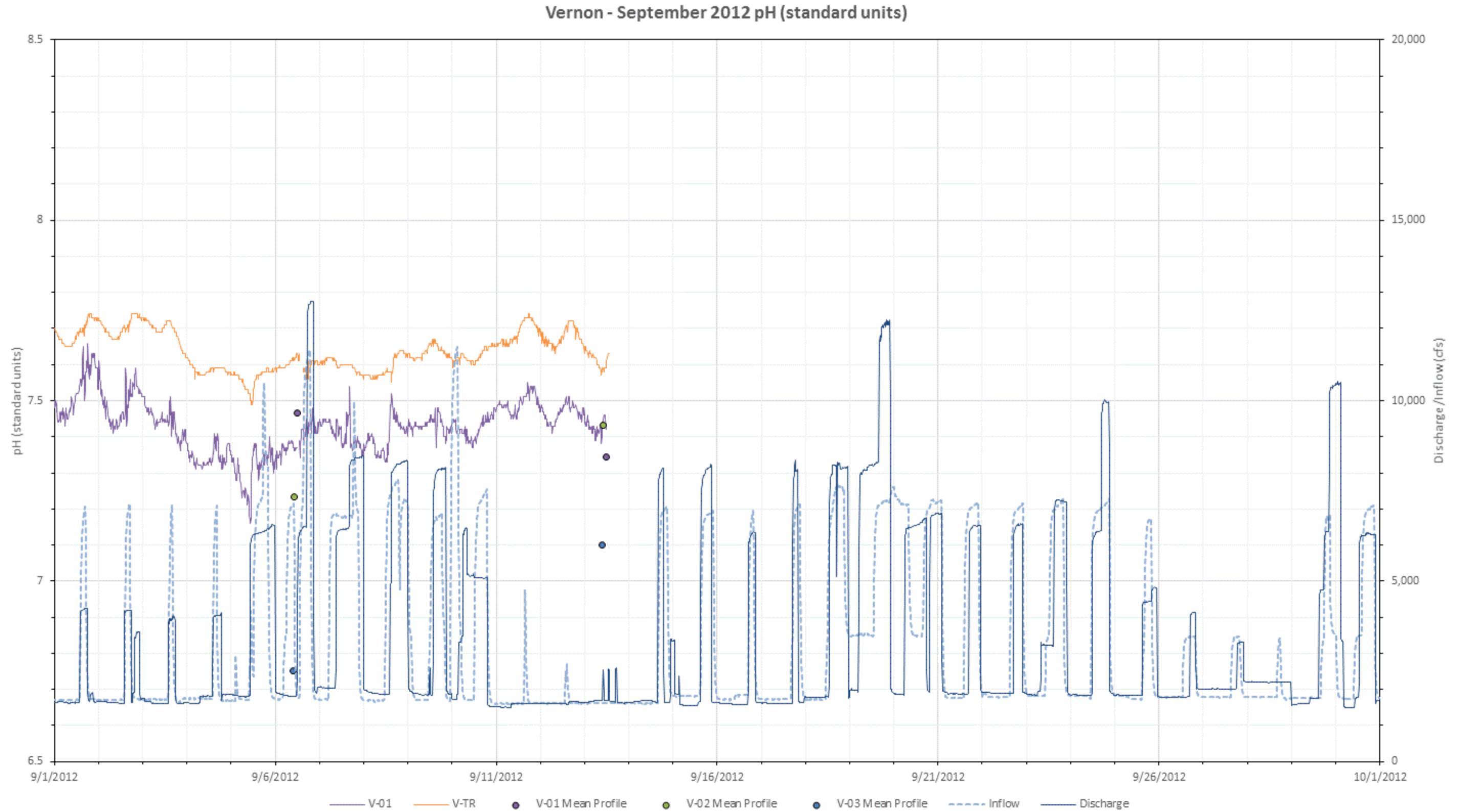
Figure L-48. 2012 September pH (standard units) at all mainstem Vernon stations with inflow (USGS Gage No. 01154500) and Vernon project discharge.
