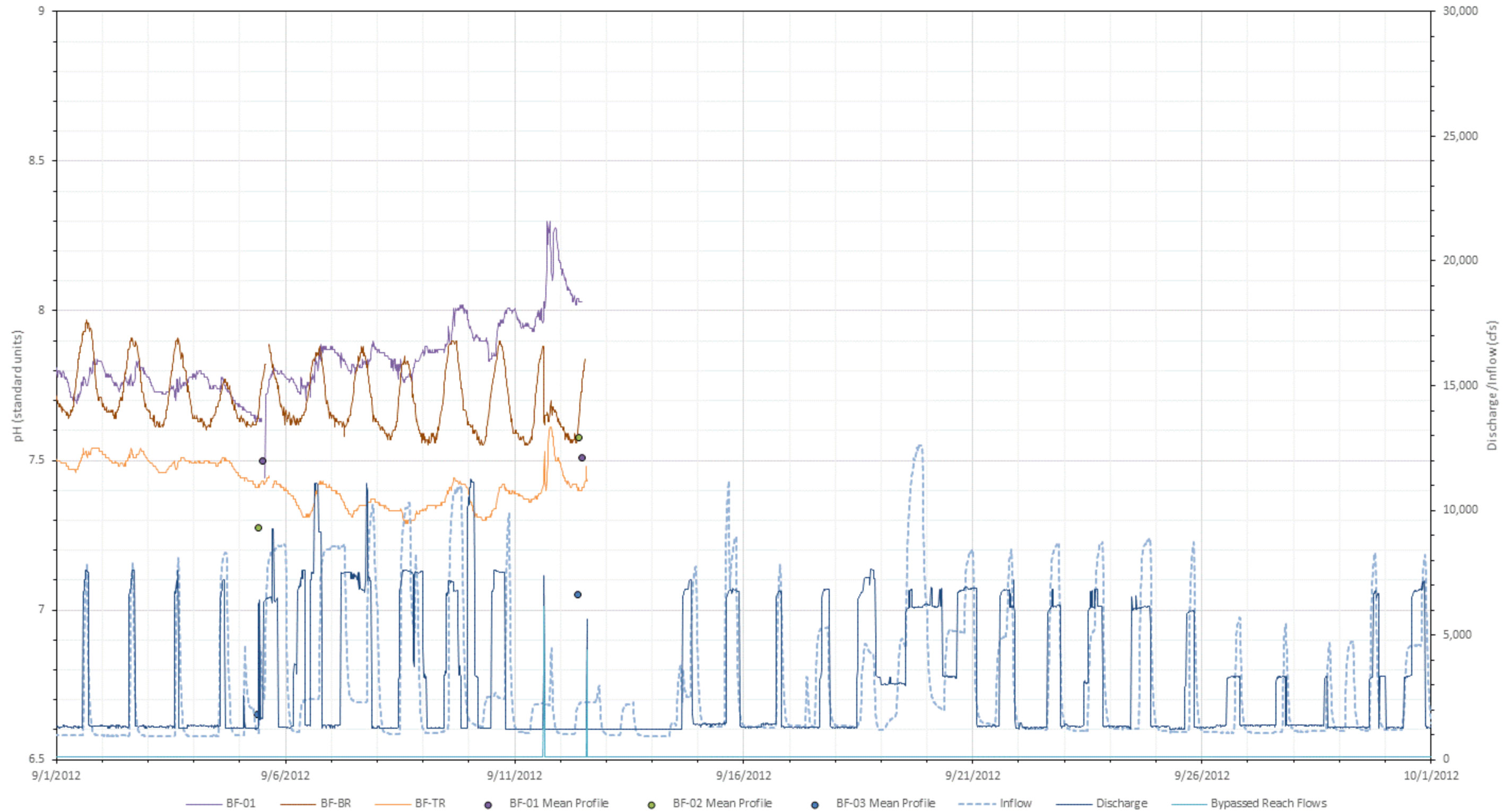
Figure L-44. 2012 September pH (standard units) at all Bellows Falls stations with inflow (USGS Gage No. 01144500), bypassed reach flow, and Bellows Falls project discharge.
