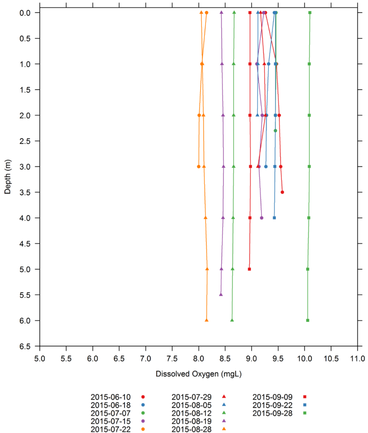
Figure H-56. Vertical profiles of dissolved oxygen (mg/L) collected at the Bellows Falls tailrace 06-BF-TR water quality monitoring station.
