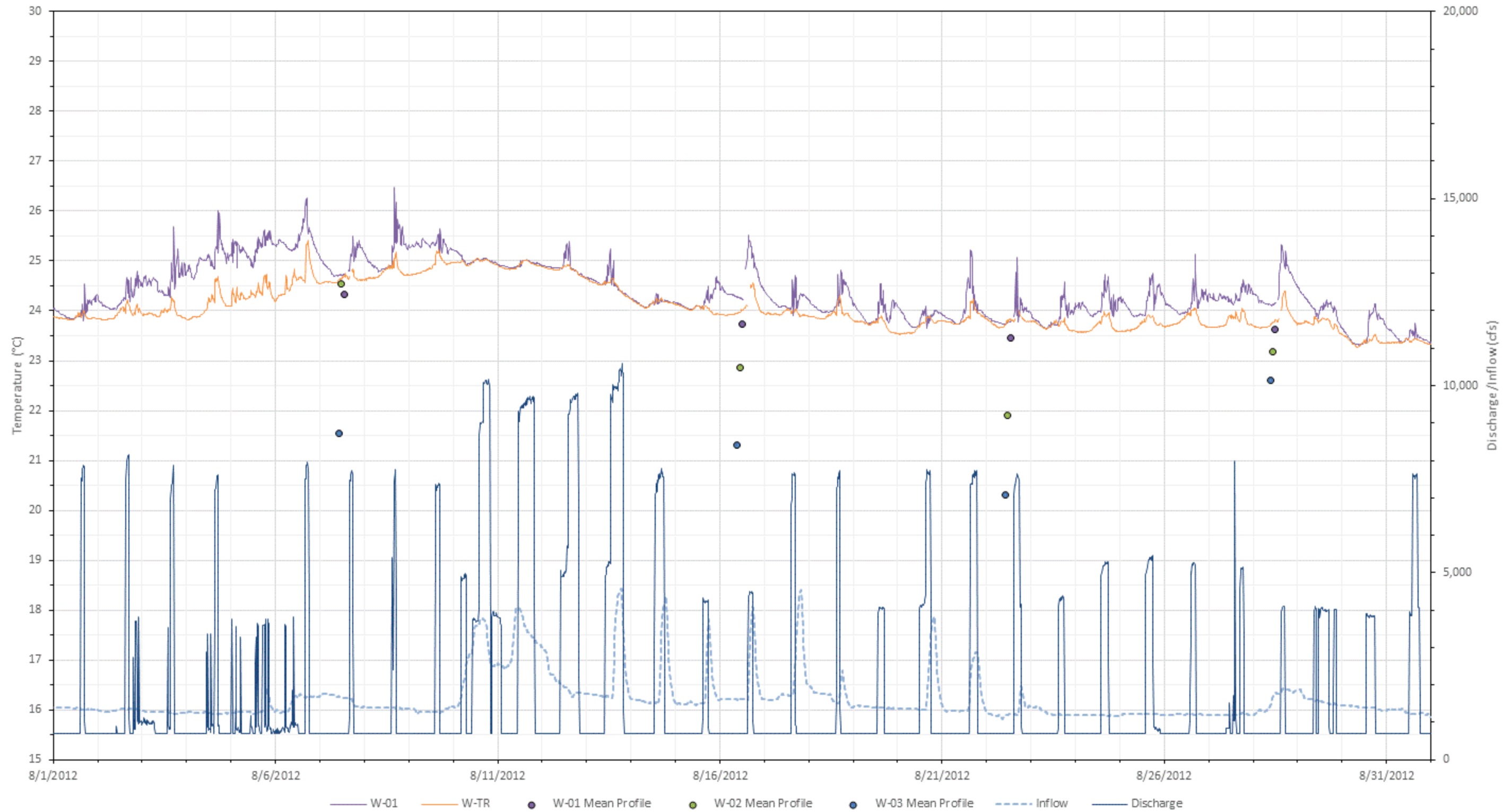
Figure L-3. 2012 August water temperatures at all Wilder stations with inflow (USGS Gage No. 01138500) and Wilder project discharge.
