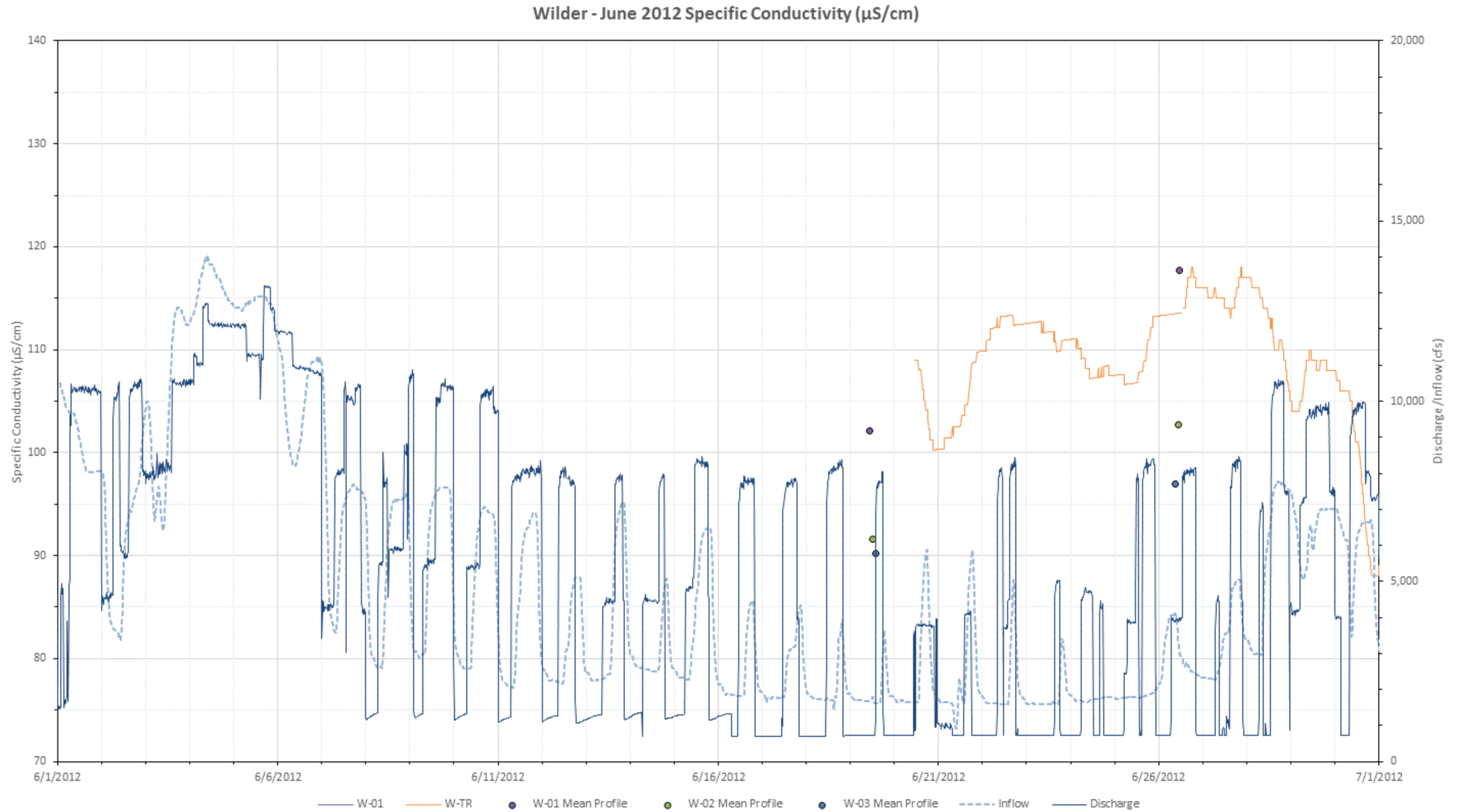
Figure L-49. 2012 June specific conductivity ( \mu\text{S}/\text{cm} ) at all Wilder mainstem stations with inflow (USGS Gage No. 0113850 Connecticut River at Wells River, VT) and Wilder project discharge.
