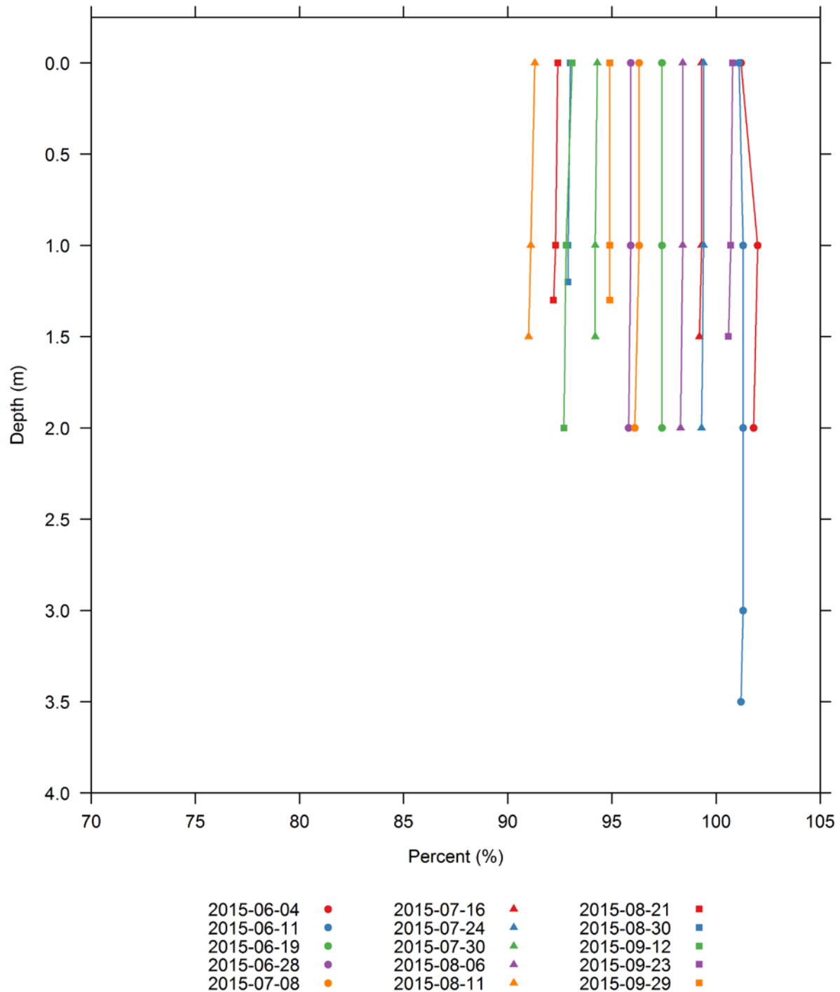
Figure H-9. Vertical profiles of dissolved oxygen (percent saturation) collected at the Wilder upper impoundment 06-W-03 water quality monitoring station.
