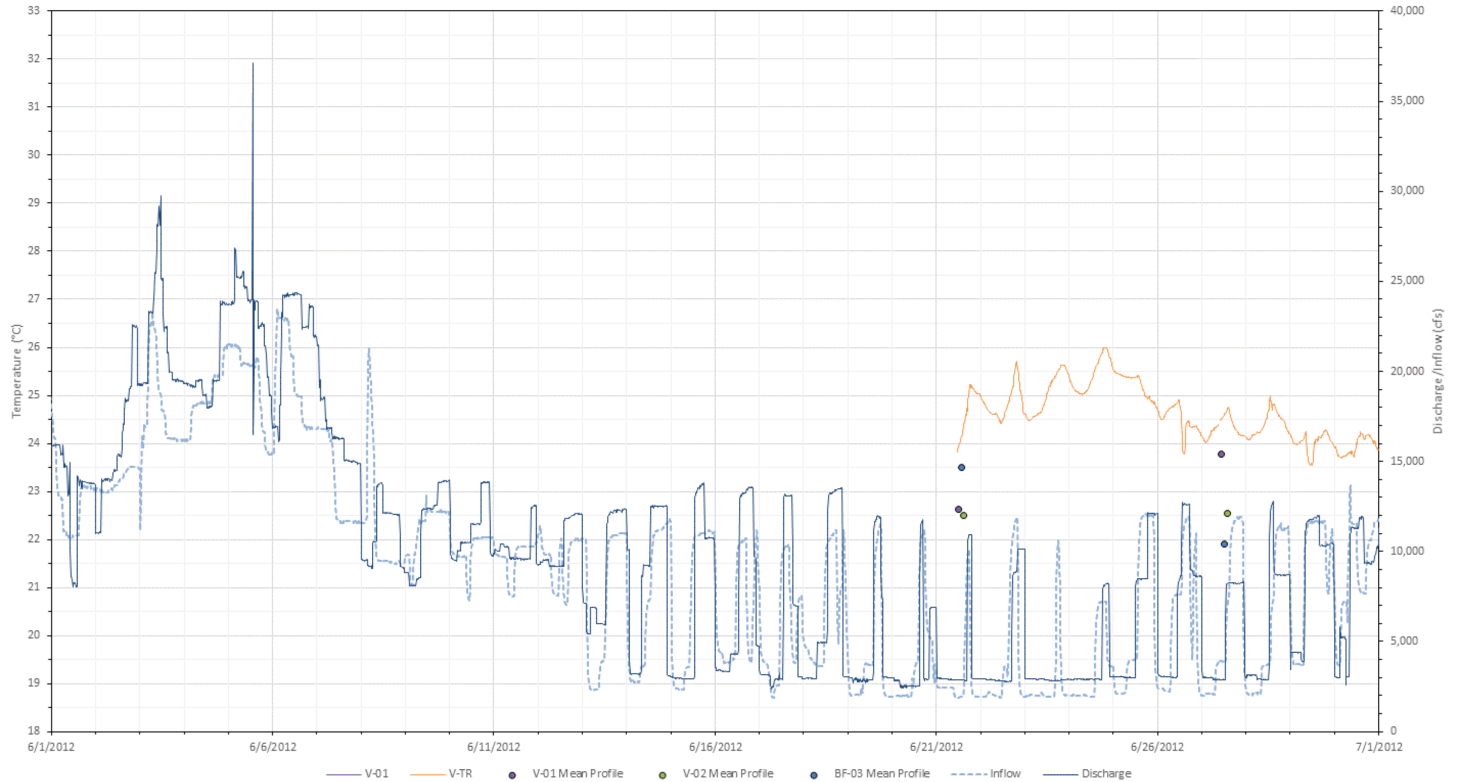
Figure L-9. 2012 June water temperatures at all mainstem Vernon stations with inflow (USGS Gage No. 01154500) and Vernon project discharge.
