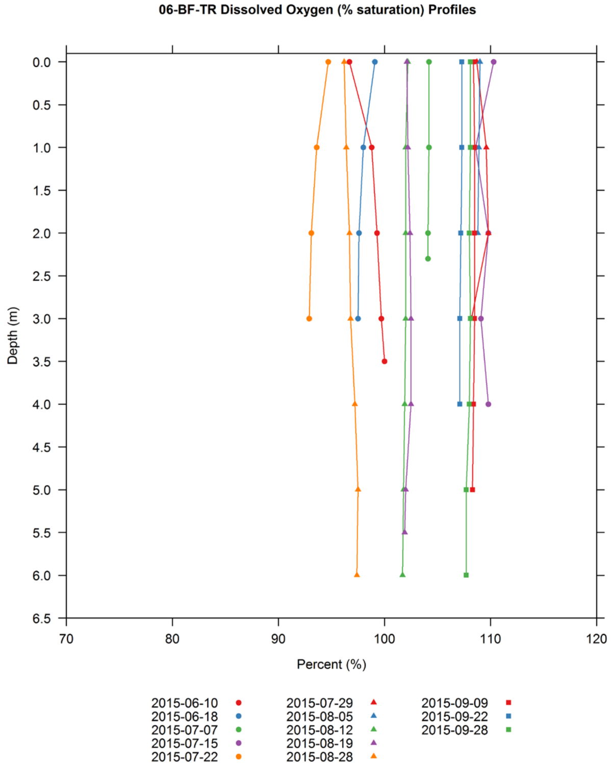
Figure H-57. Vertical profiles of dissolved oxygen (percent saturation) collected at the Bellows Falls tailrace O6-BF-TR water quality monitoring station.
