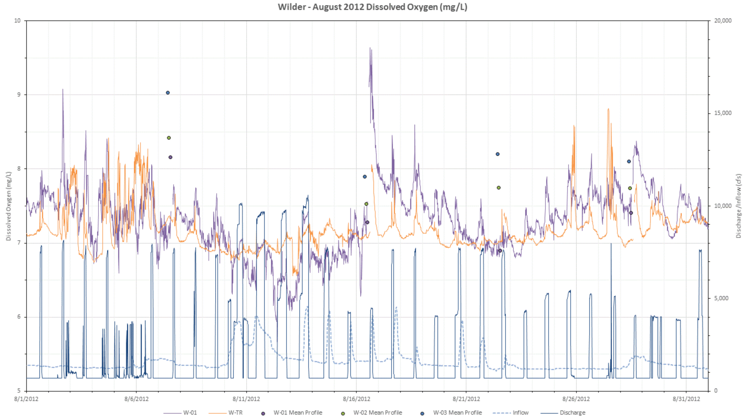
Figure L-15. 2012 August dissolved oxygen (mg/L) at all Wilder mainstem stations with inflow (USGS Gage No. 01138500) and Wilder project discharge.
