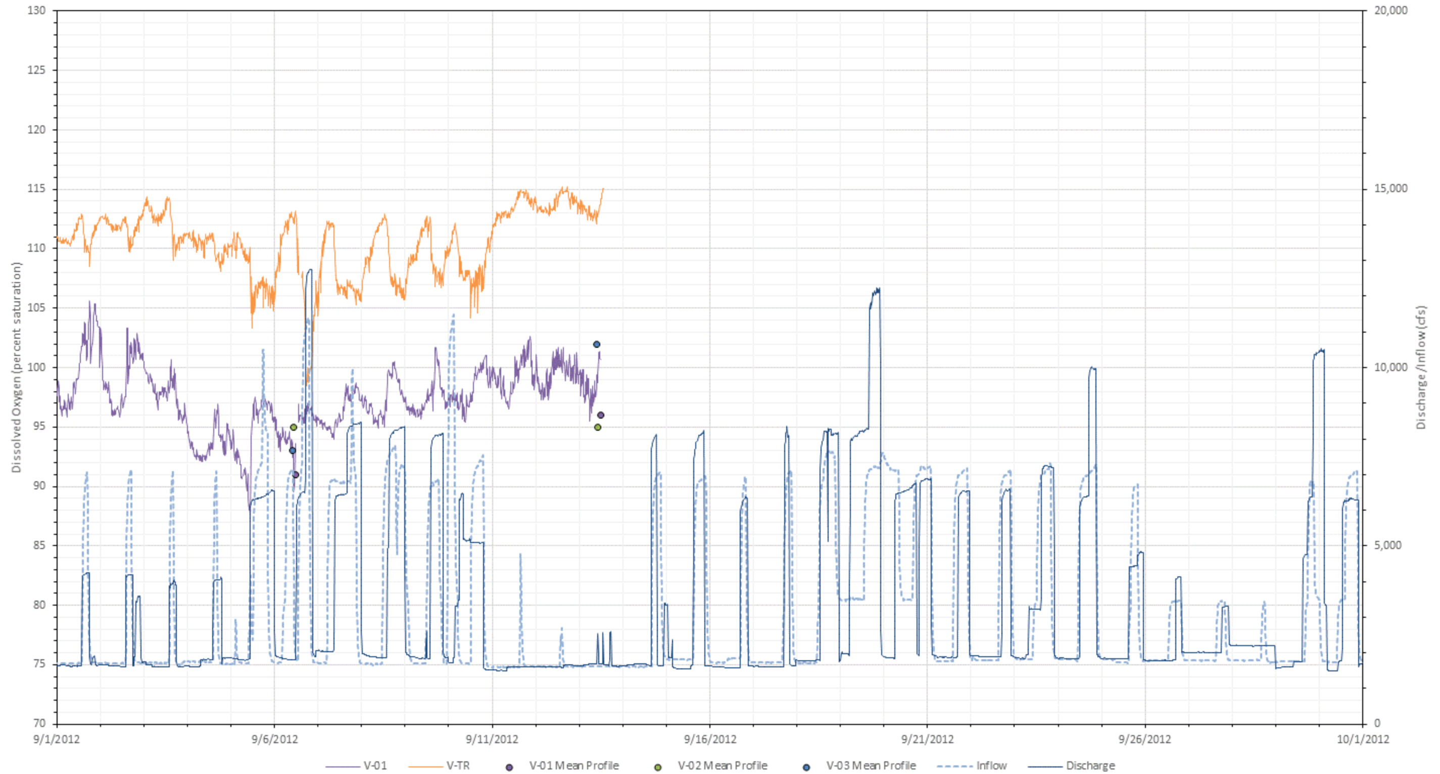
Figure L-36. 2012 September dissolved oxygen (percent saturation) at all mainstem Vernon stations with inflow (USGS Gage No. 01154500) and Vernon project discharge.
