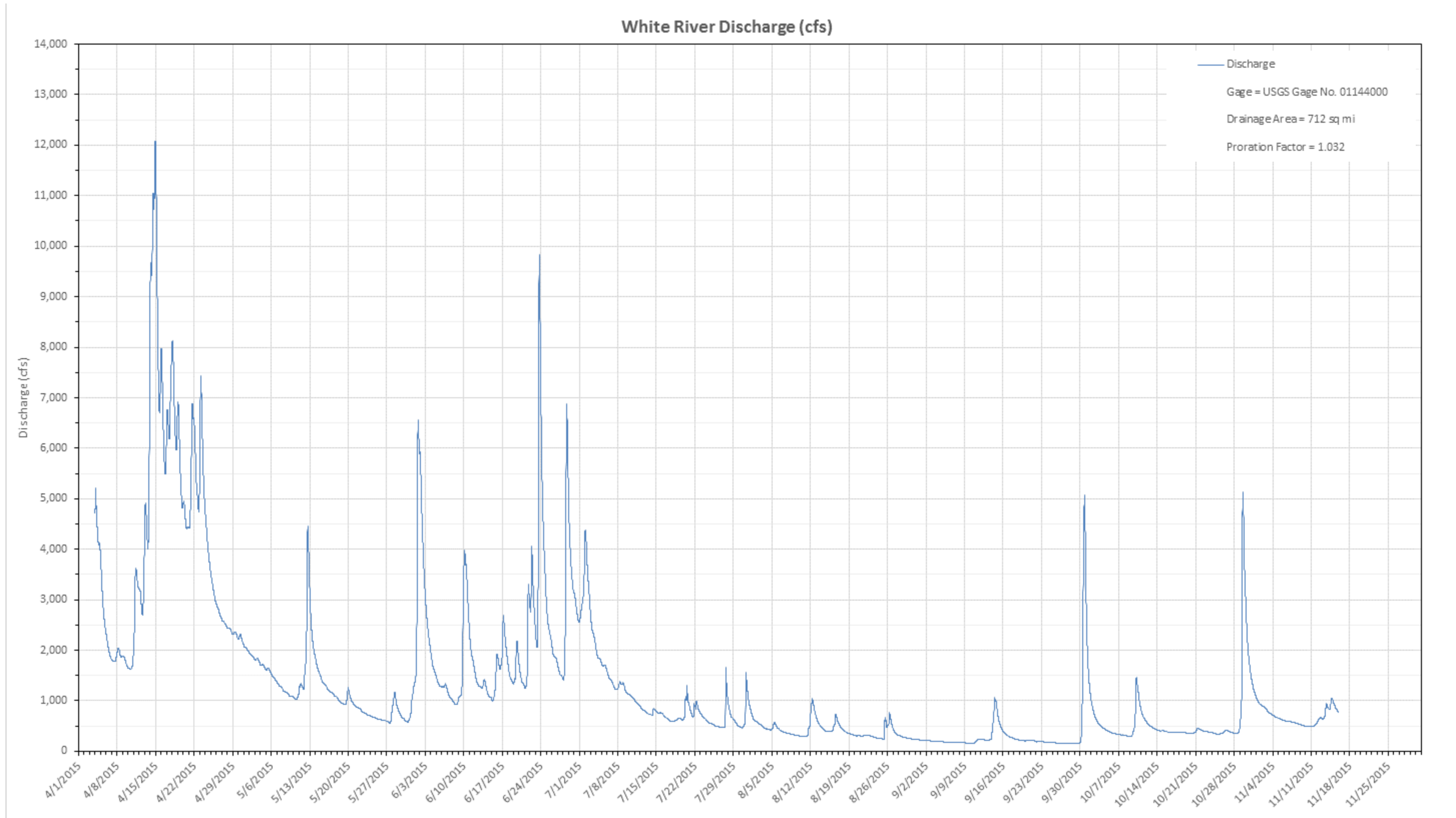
Figure C-3. 2015 White River hydrograph of the study period from April 1 through November 15. Discharges estimated based on prorated flows at USGS Gage No. 01144000.
