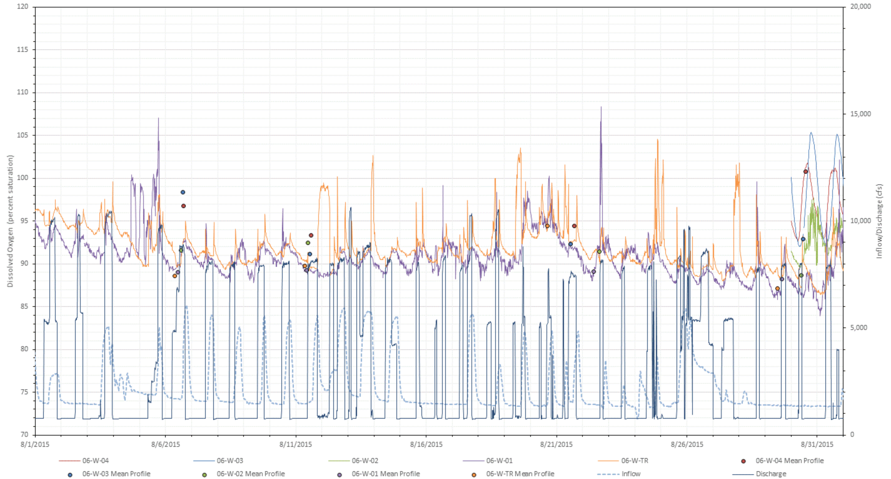
Figure F-38. 2015 August dissolved oxygen (percent saturation) at all Wilder mainstem stations with inflow (USGS Gage No. 01138500) and Wilder project discharge.
