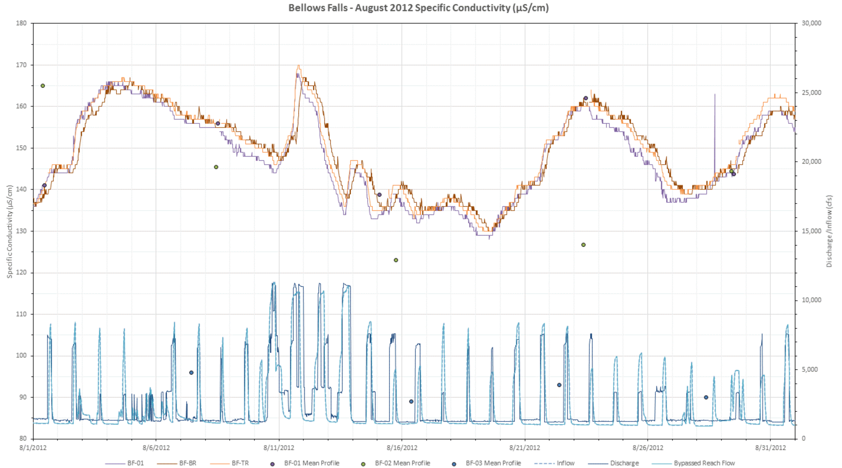
Figure L-55. 2012 August specific conductivity ( \mu\text{S}/\text{cm} ) at all Bellows Falls stations with inflow (USGS Gage No. 01144500), bypassed reach flow, and Bellows Falls project discharge.
