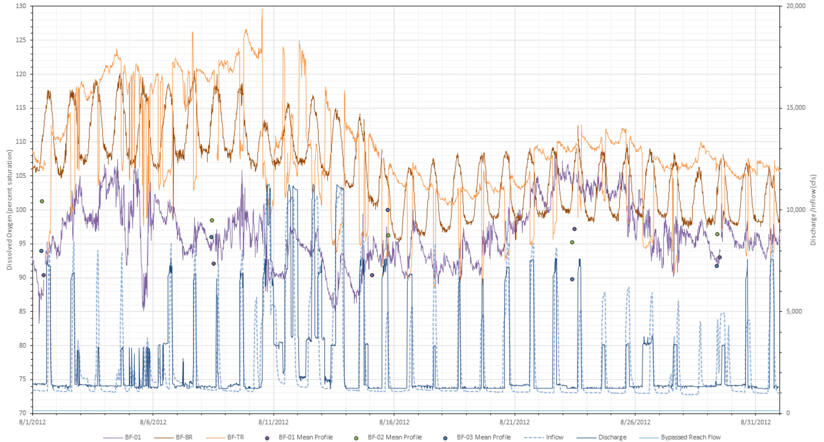
Figure L-31. 2012 August dissolved oxygen (percent saturation) at all Bellows Falls stations with inflow (USGS Gage No. 01144500), bypassed reach flow, and Bellows Falls project discharge.
