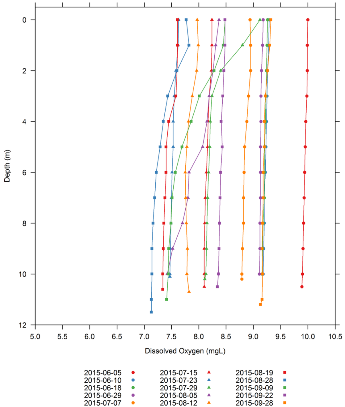
Figure H-50. Vertical profiles of dissolved oxygen (mg/L) collected at the Bellows Falls forebay 06-BF-01 water quality monitoring station.
