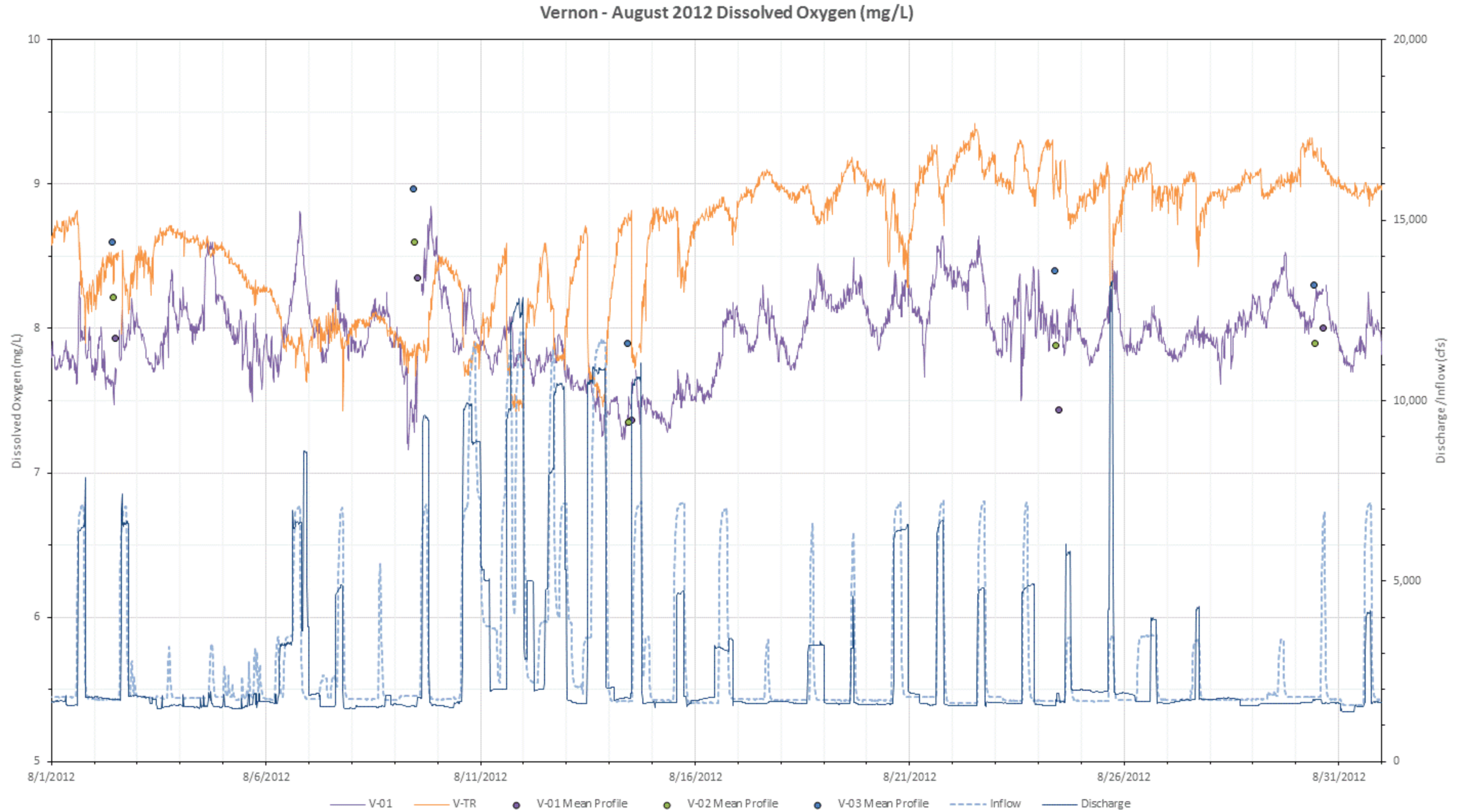
Figure L-23. 2012 August dissolved oxygen (mg/L) at all mainstem Vernon stations with inflow (USGS Gage No. 01154500) and Vernon project discharge.
