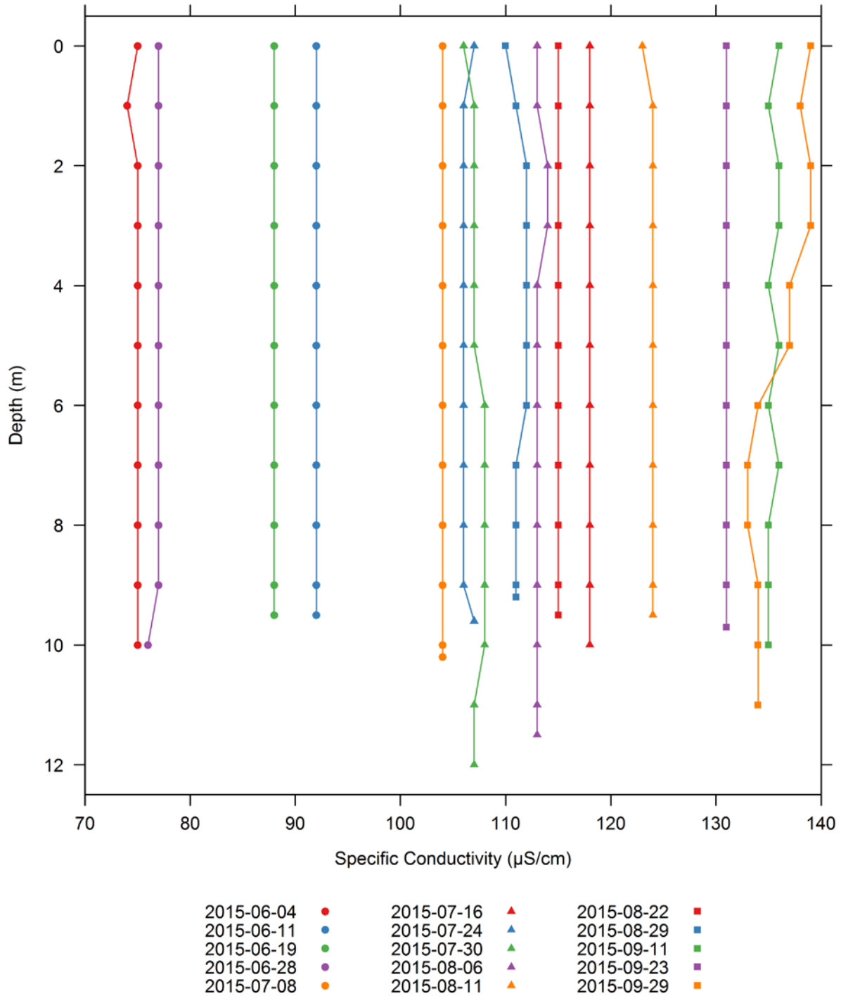
Figure H-22. Vertical profiles of specific conductivity ( \mu\text{S}/\text{cm} ) collected at the Wilder forebay 06-W-01 water quality monitoring station.
