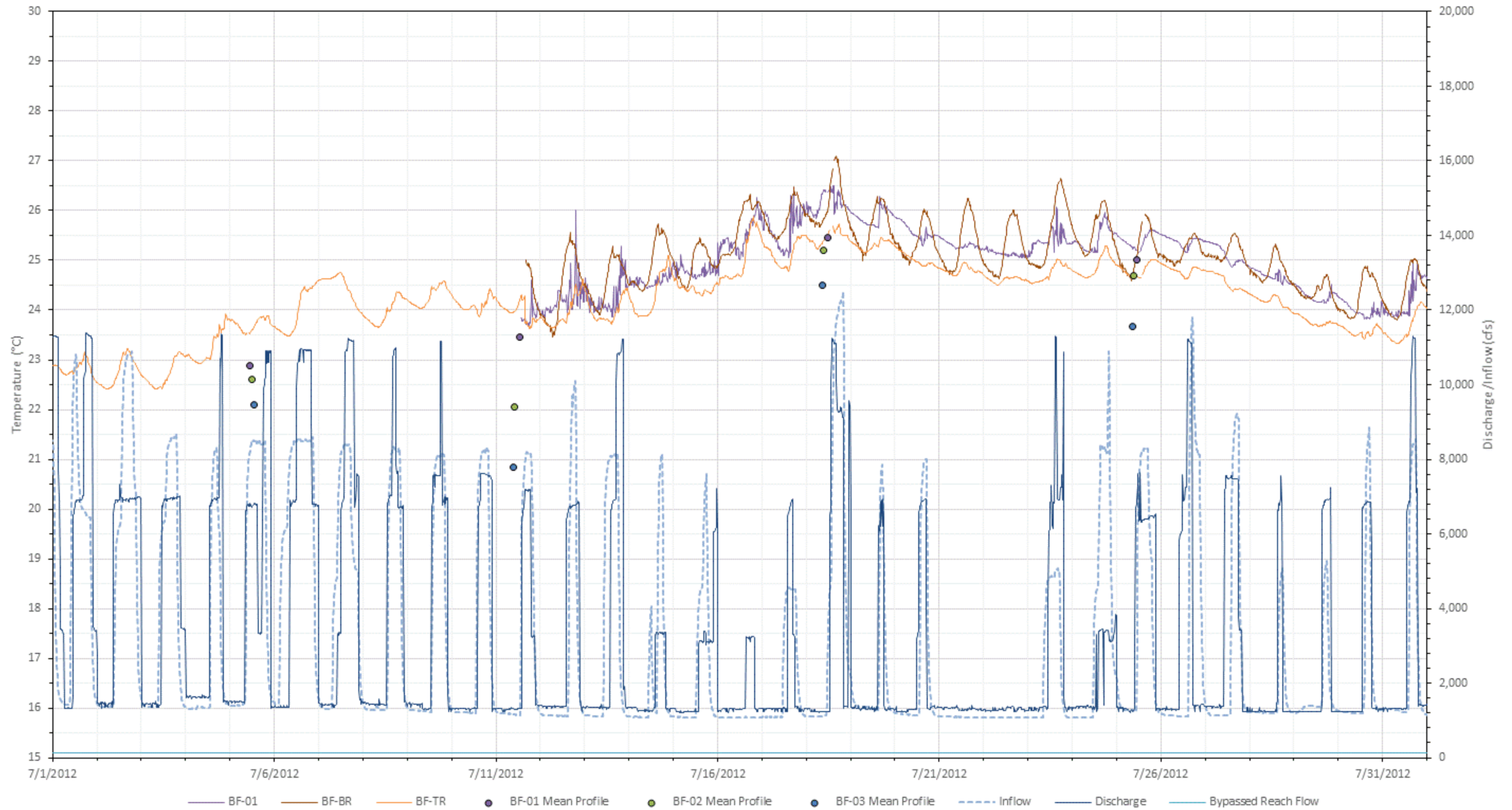
Figure L-6. 2012 July water temperatures at all Bellows Falls stations with inflow (USGS Gage No. 01144500), bypassed reach flow, and Bellows Falls project discharge.
