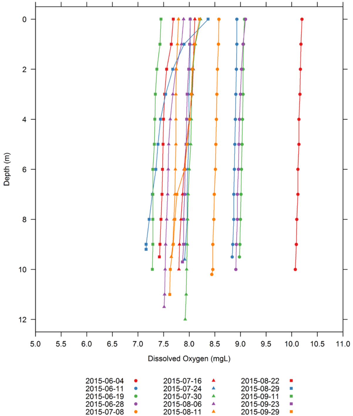
Figure H-20. Vertical profiles of dissolved oxygen (mg/L) collected at the Wilder forebay 06-W-01 water quality monitoring station.
