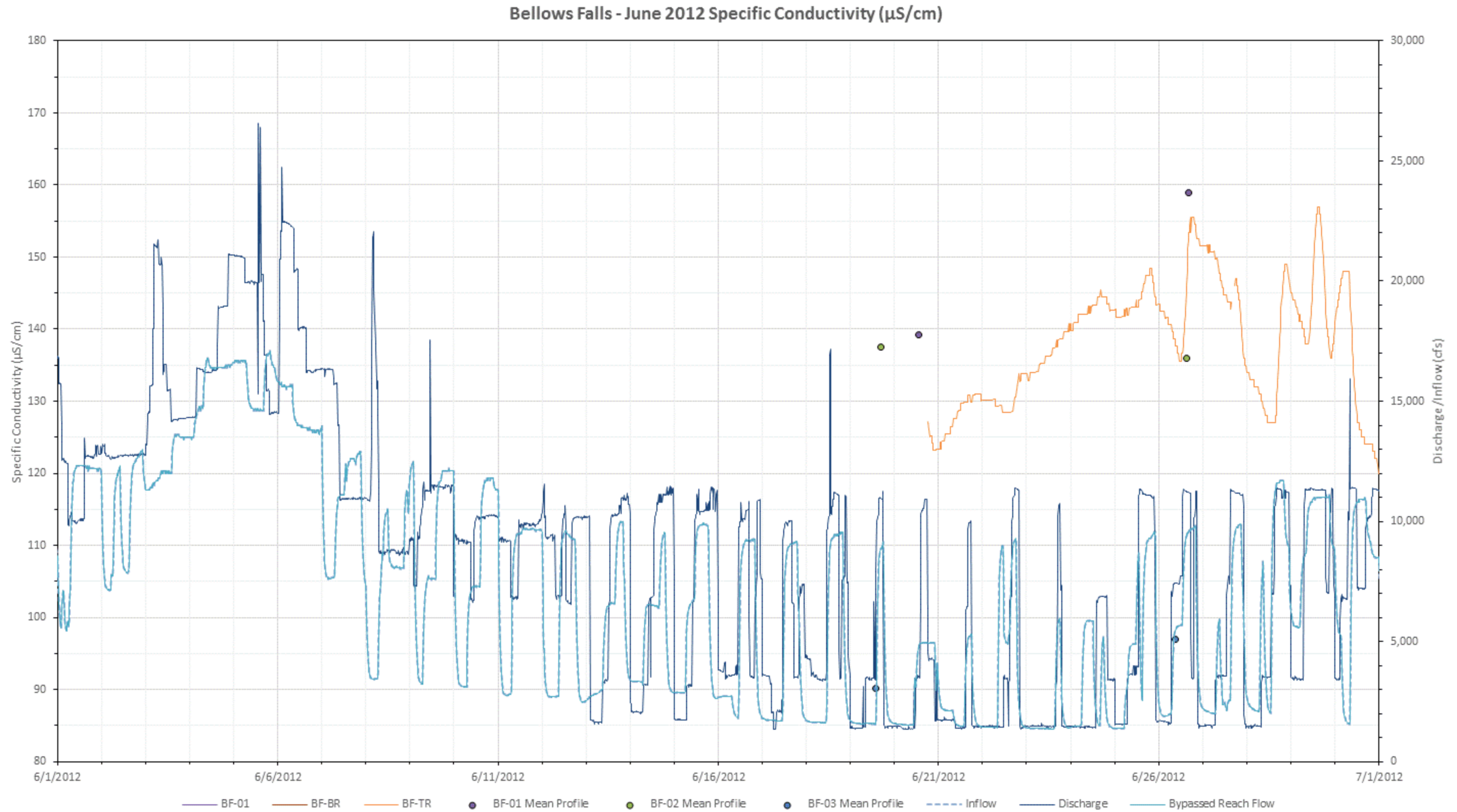
Figure L-53. 2012 June specific conductivity ( \mu\text{S}/\text{cm} ) at all Bellows Falls stations with inflow (USGS Gage No. 01144500), bypassed reach flow, and Bellows Falls project discharge.
