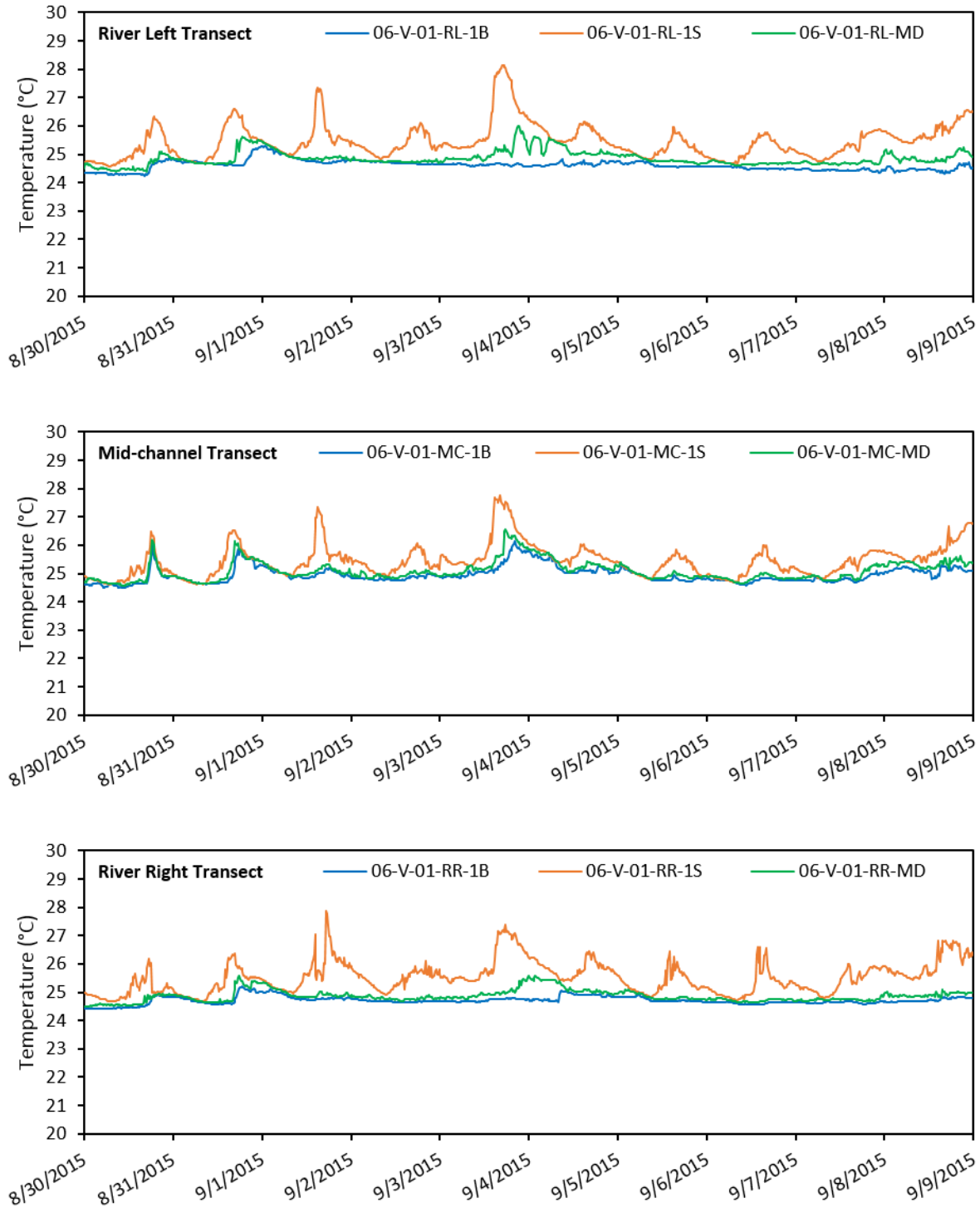
Figure I-12. Continuous water temperature collected at the Vernon forebay 06-V-01 water quality monitoring station during the high temperature low flow monitoring period. Loggers were deployed at one meter below the surface (1S), mid-depth (MD), and one meter above the river bottom (1B).
