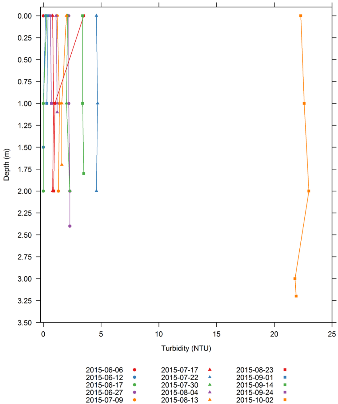
Figure H-66. Vertical profiles of turbidity (NTU) collected at the Vernon upstream 06-V-04 water quality monitoring station.
