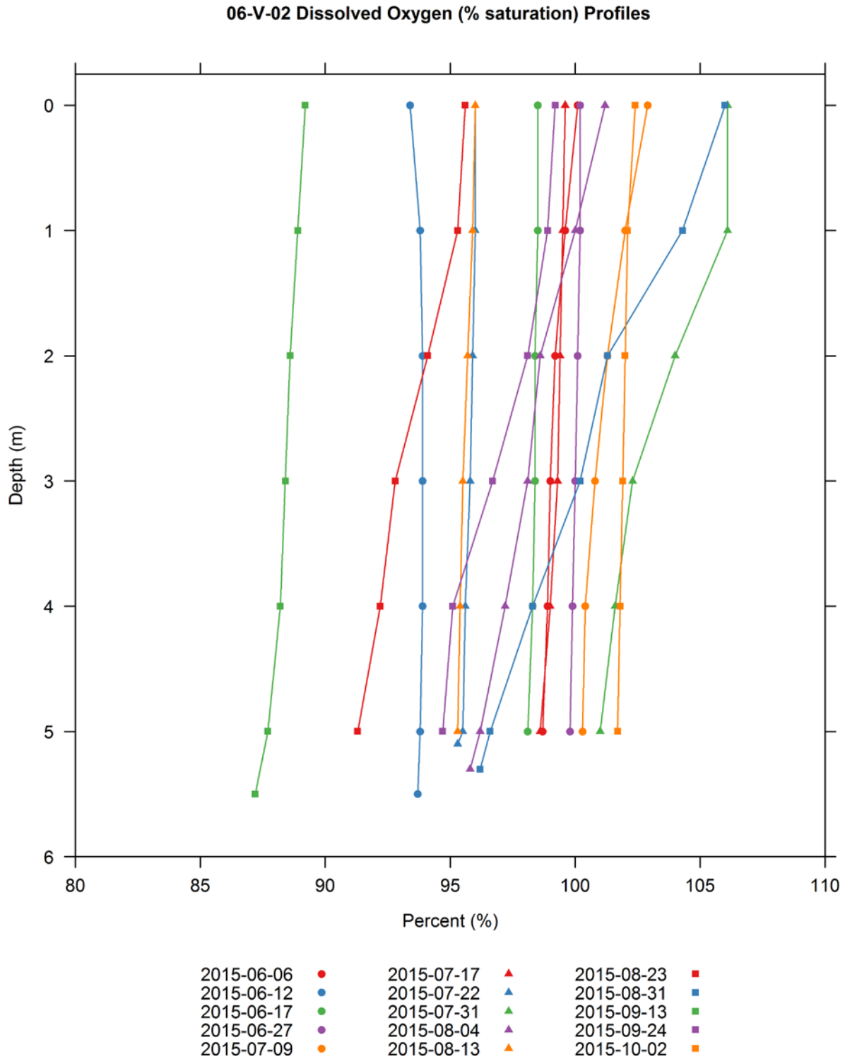
Figure H-75. Vertical profiles of dissolved oxygen (percent saturation) collected at the Vernon middle impoundment 06-V-02 water quality monitoring station.
