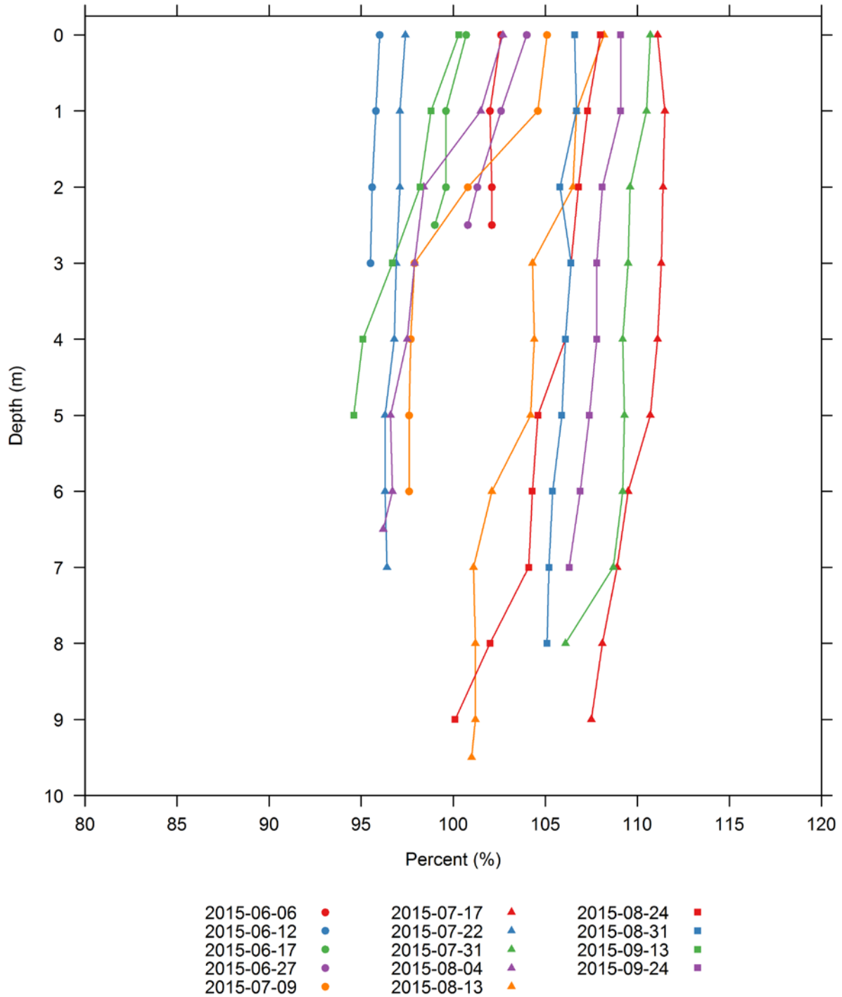
Figure H-87. Vertical profiles of dissolved oxygen (percent saturation) collected at the Vernon tailrace 06-V-TR water quality monitoring station.
