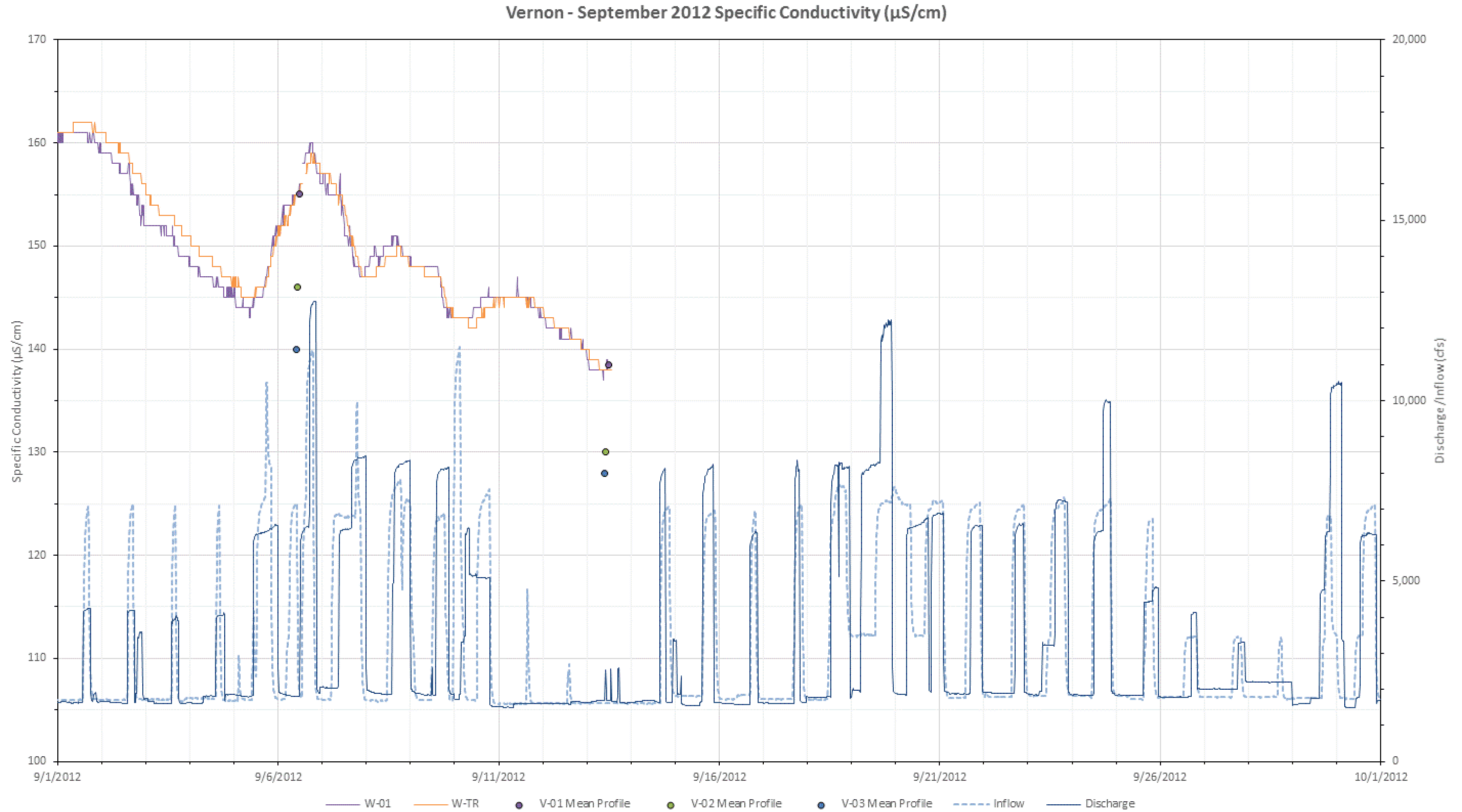
Figure L-60. 2012 September specific conductivity ( \mu\text{S}/\text{cm} ) at all mainstem Vernon stations with inflow (USGS Gage No. 01154500) and Vernon project discharge.
