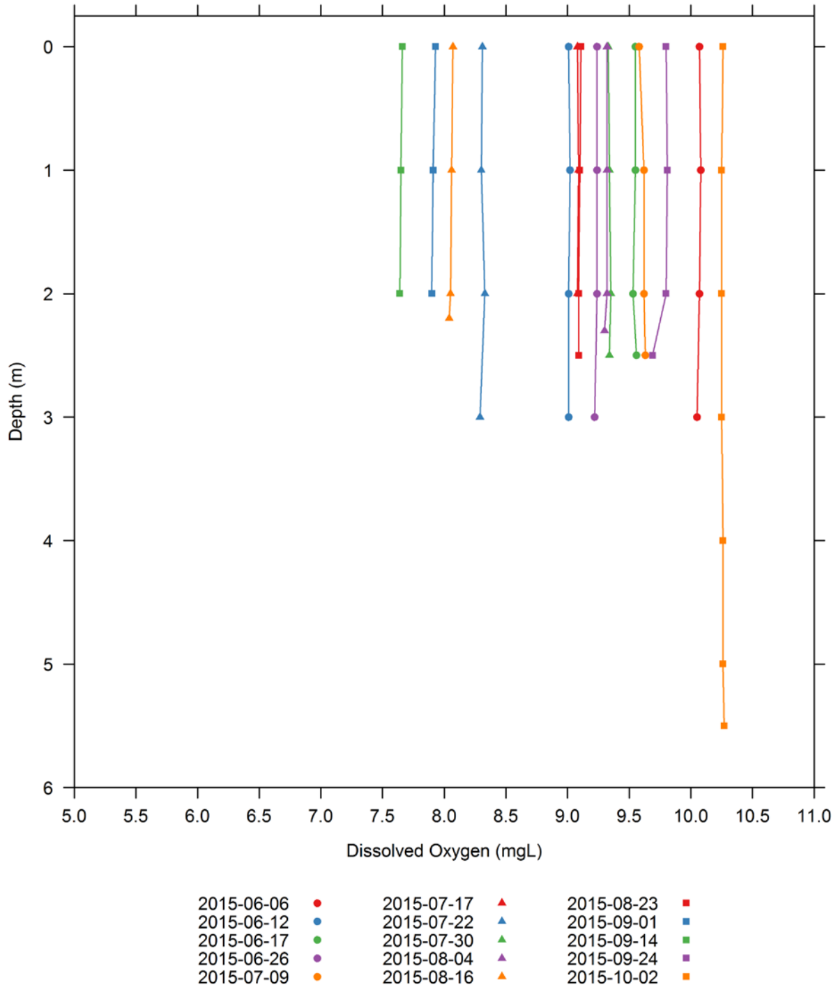
Figure H-68. Vertical profiles of dissolved oxygen (mg/L) collected at the Vernon upper impoundment 06-V-03 water quality monitoring station.
