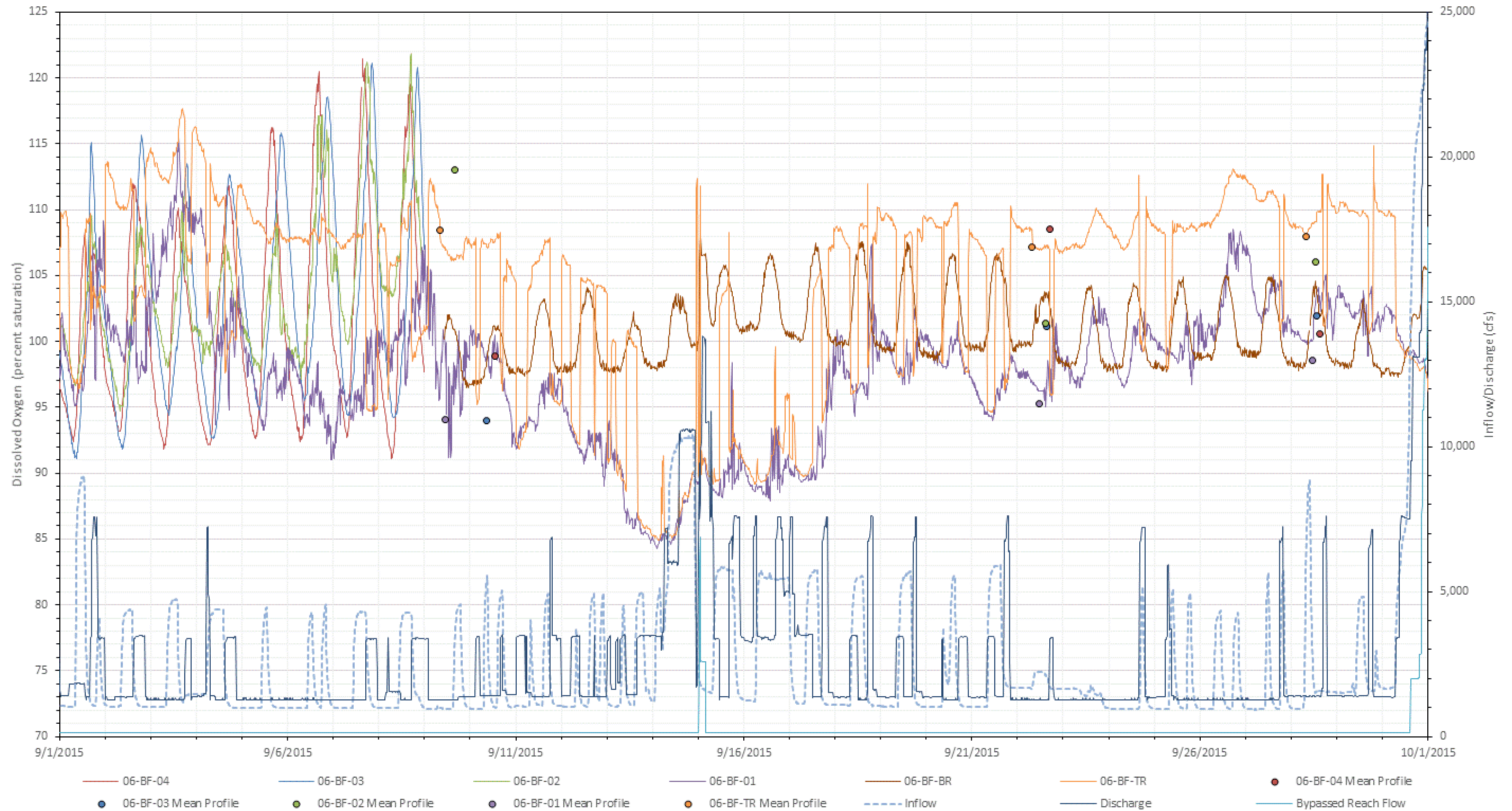
Figure F-43. 2015 September dissolved oxygen (percent saturation) at all Bellows Falls stations with inflow (USGS Gage No. 01144500), bypassed reach flow, and project discharge.
