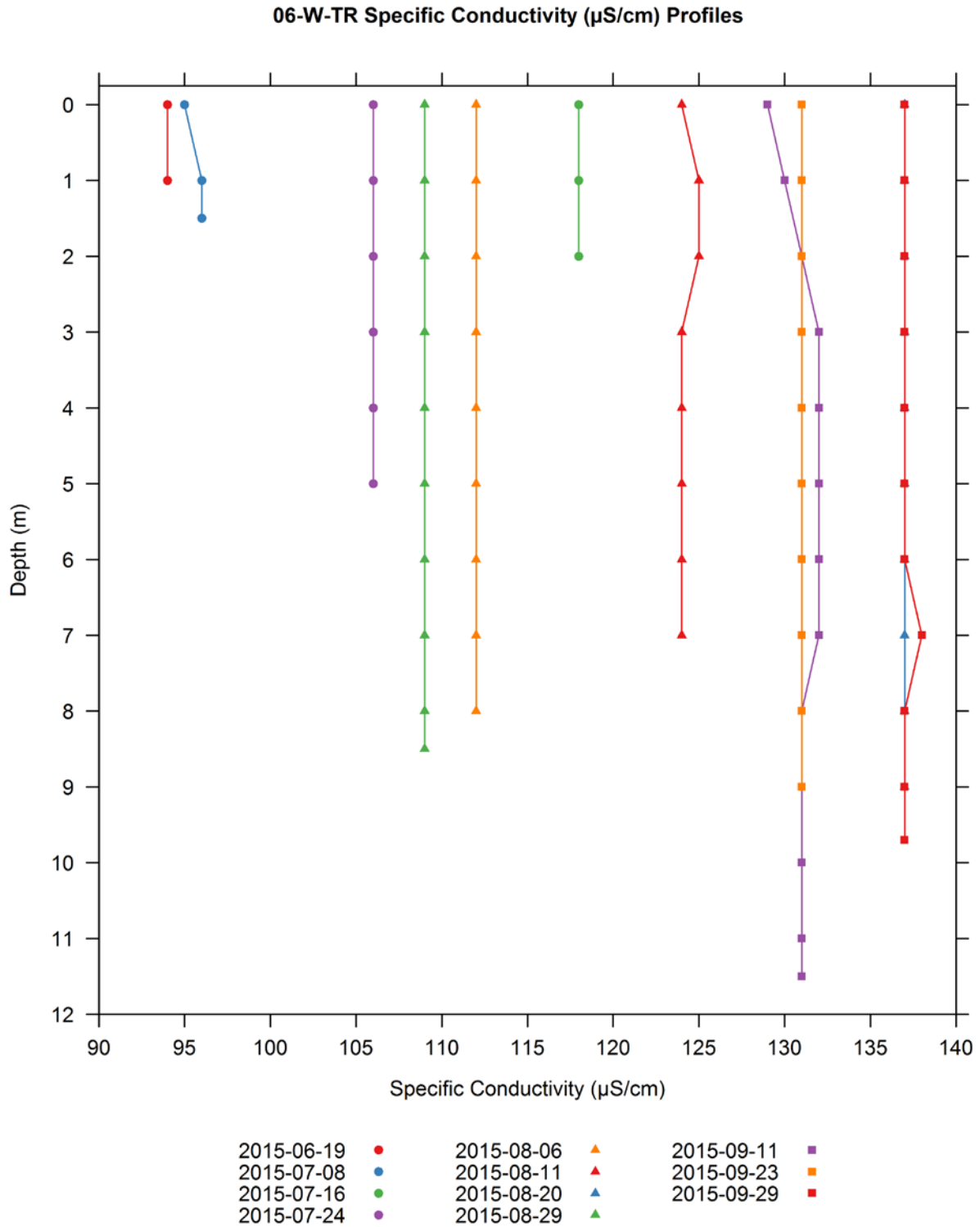
Figure H-28. Vertical profiles of specific conductivity ( \mu\text{S}/\text{cm} ) collected at the Wilder tailrace 06-W-TR water quality monitoring station.
