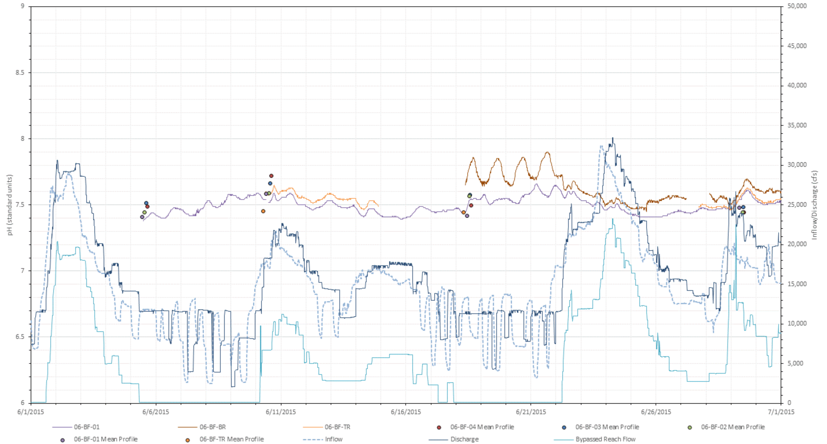
Bellows Falls - June 2015 pH (standard units)
