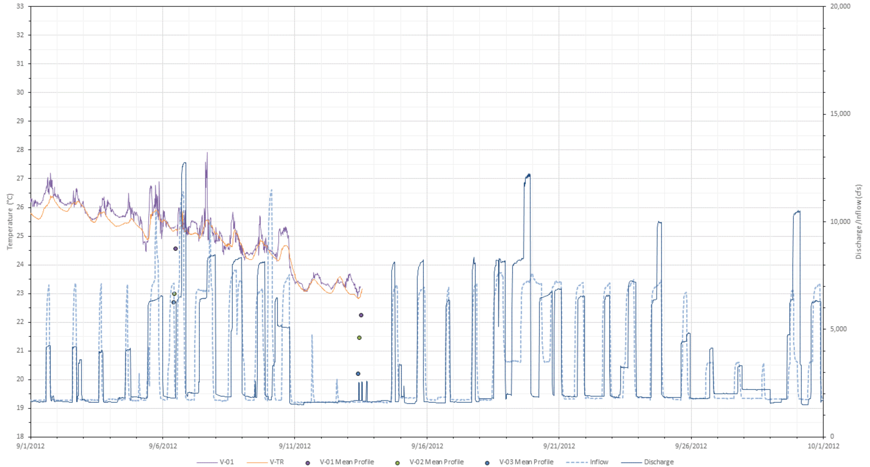
Figure L-12. 2012 September water temperatures at all mainstem Vernon stations with inflow (USGS Gage No. 01154500) and Vernon project discharge.
