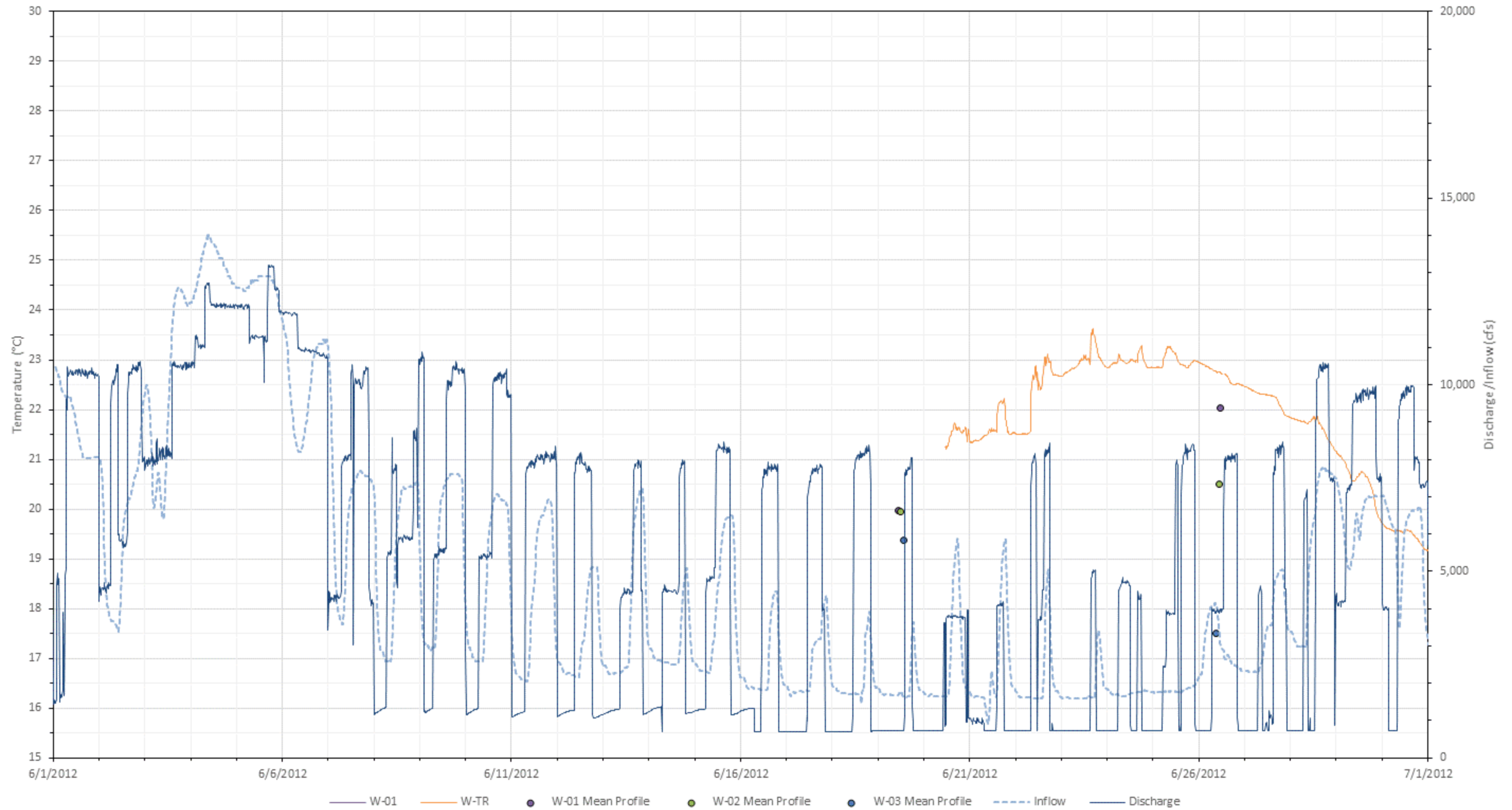
Figure L-1. 2012 June water temperatures at all Wilder stations with inflow (USGS Gage No. 01138500) and Wilder project discharge.
