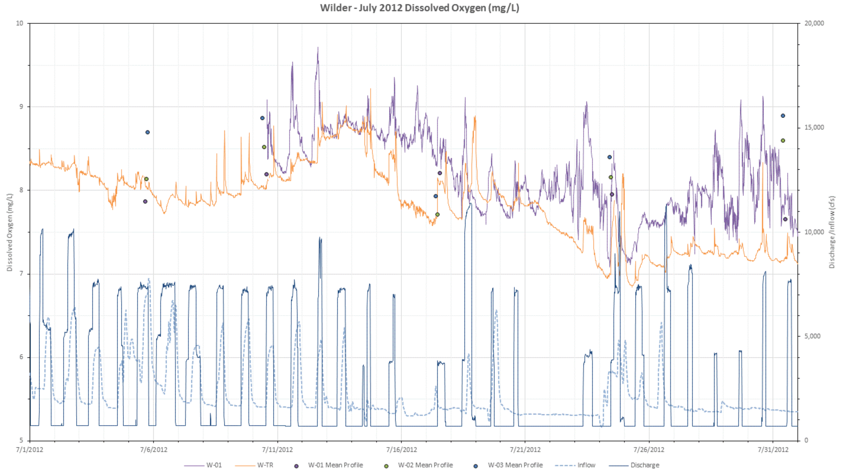
Figure L-14. 2012 July dissolved oxygen (mg/L) at all Wilder mainstem stations with inflow (USGS Gage No. 01138500) and Wilder project discharge.
