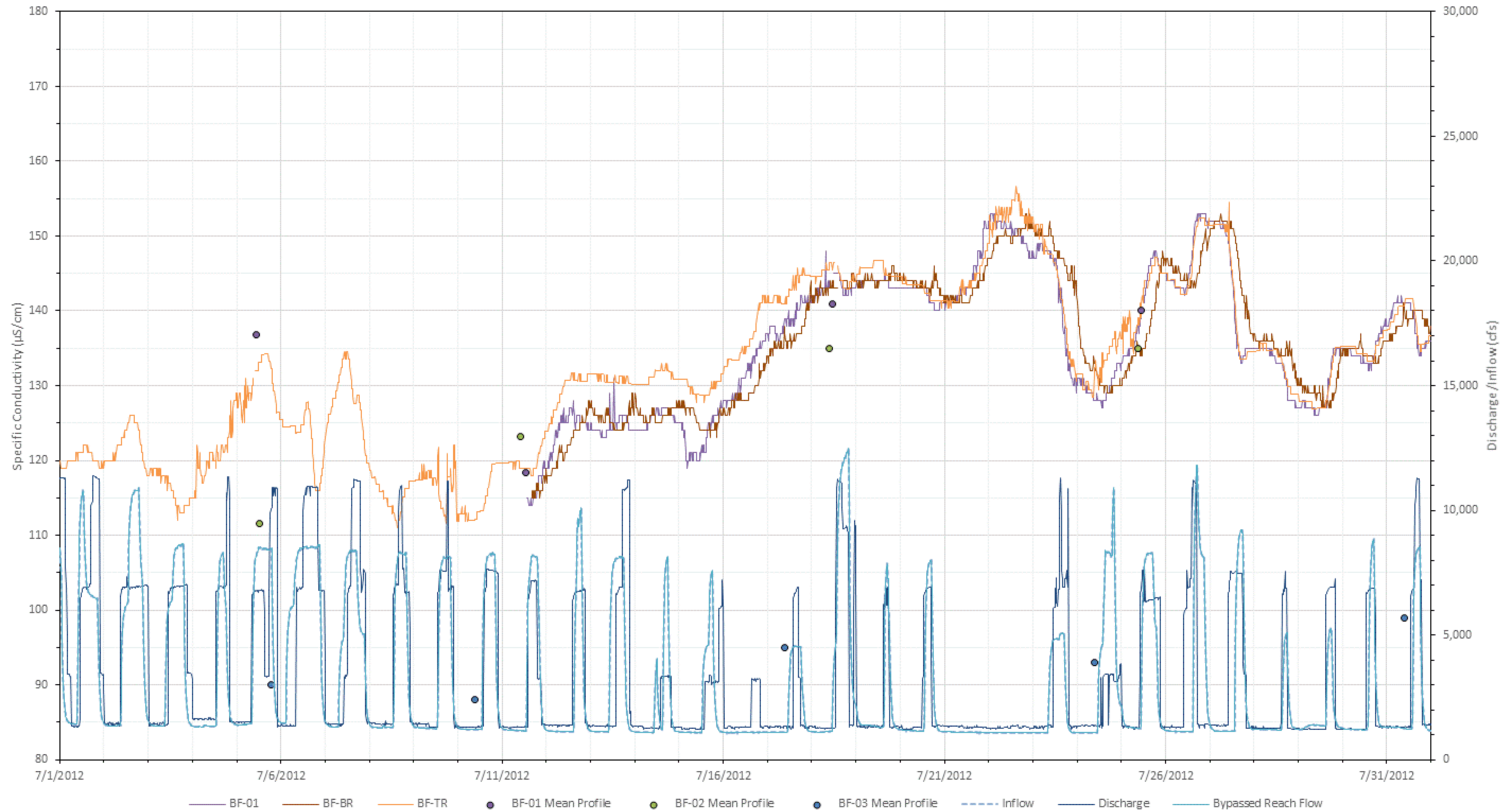
Figure L-54. 2012 July specific conductivity ( \mu\text{S}/\text{cm} ) at all Bellows Falls stations with inflow (USGS Gage No. 01144500), bypassed reach flow, and Bellows Falls project discharge.
