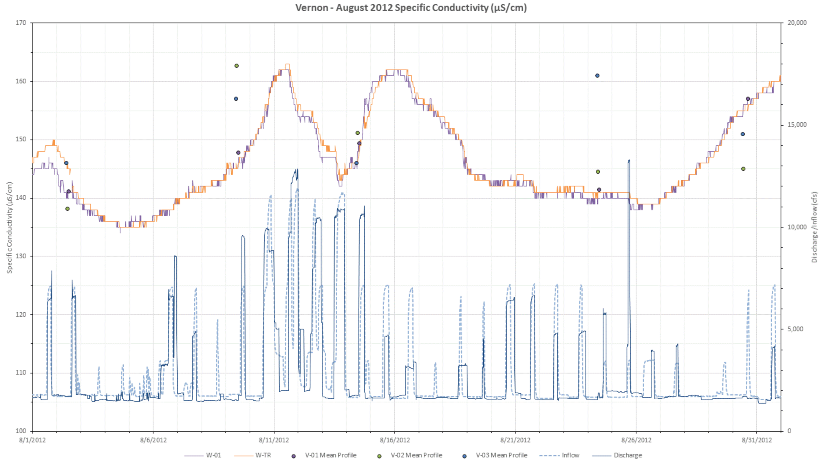
Figure L-59. 2012 August specific conductivity ( \mu\text{S}/\text{cm} ) at all mainstem Vernon stations with inflow (USGS Gage No. 01154500) and Vernon project discharge.
