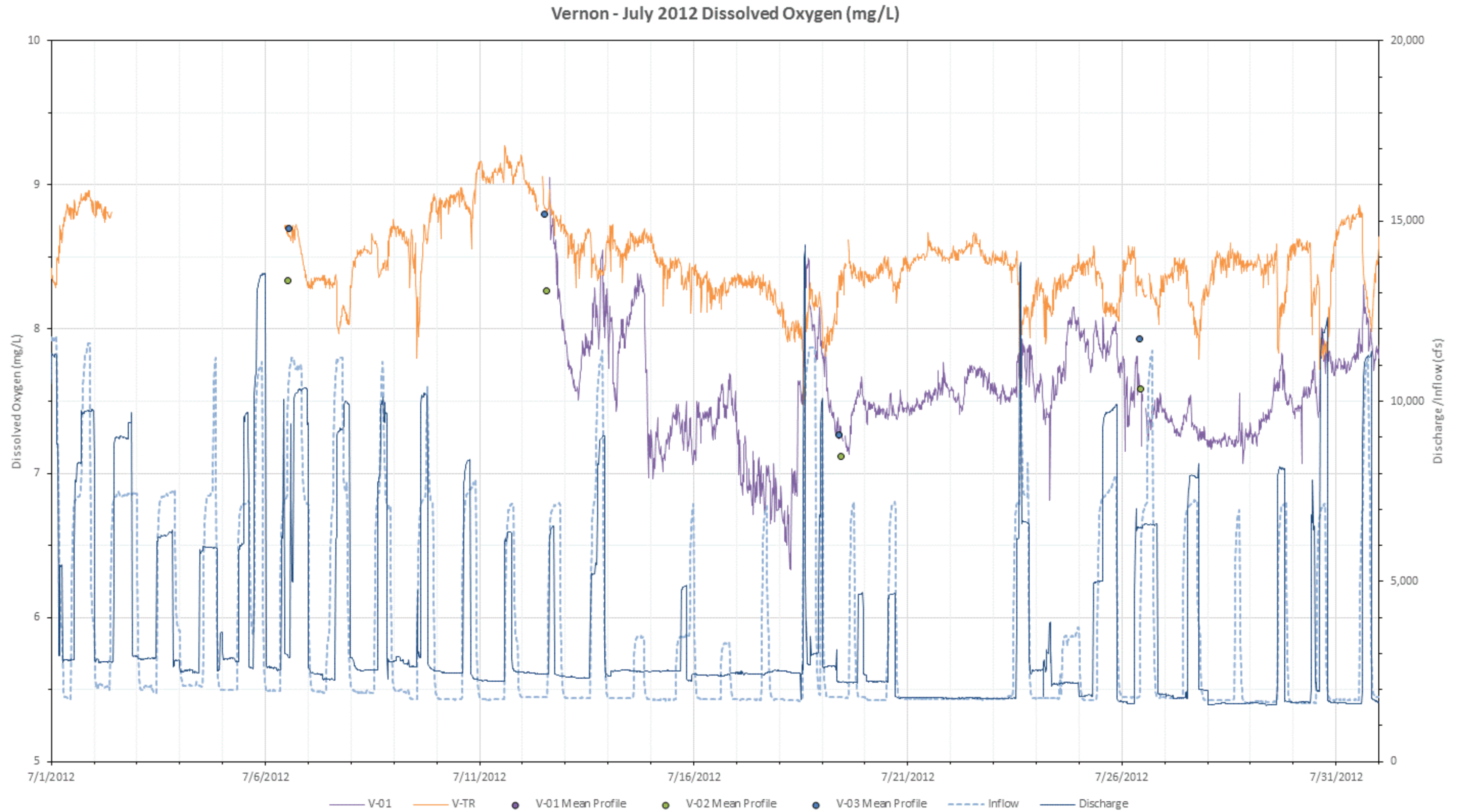
Figure L-22. 2012 July dissolved oxygen (mg/L) at all mainstem Vernon stations with inflow (USGS Gage No. 01154500) and Vernon project discharge.
