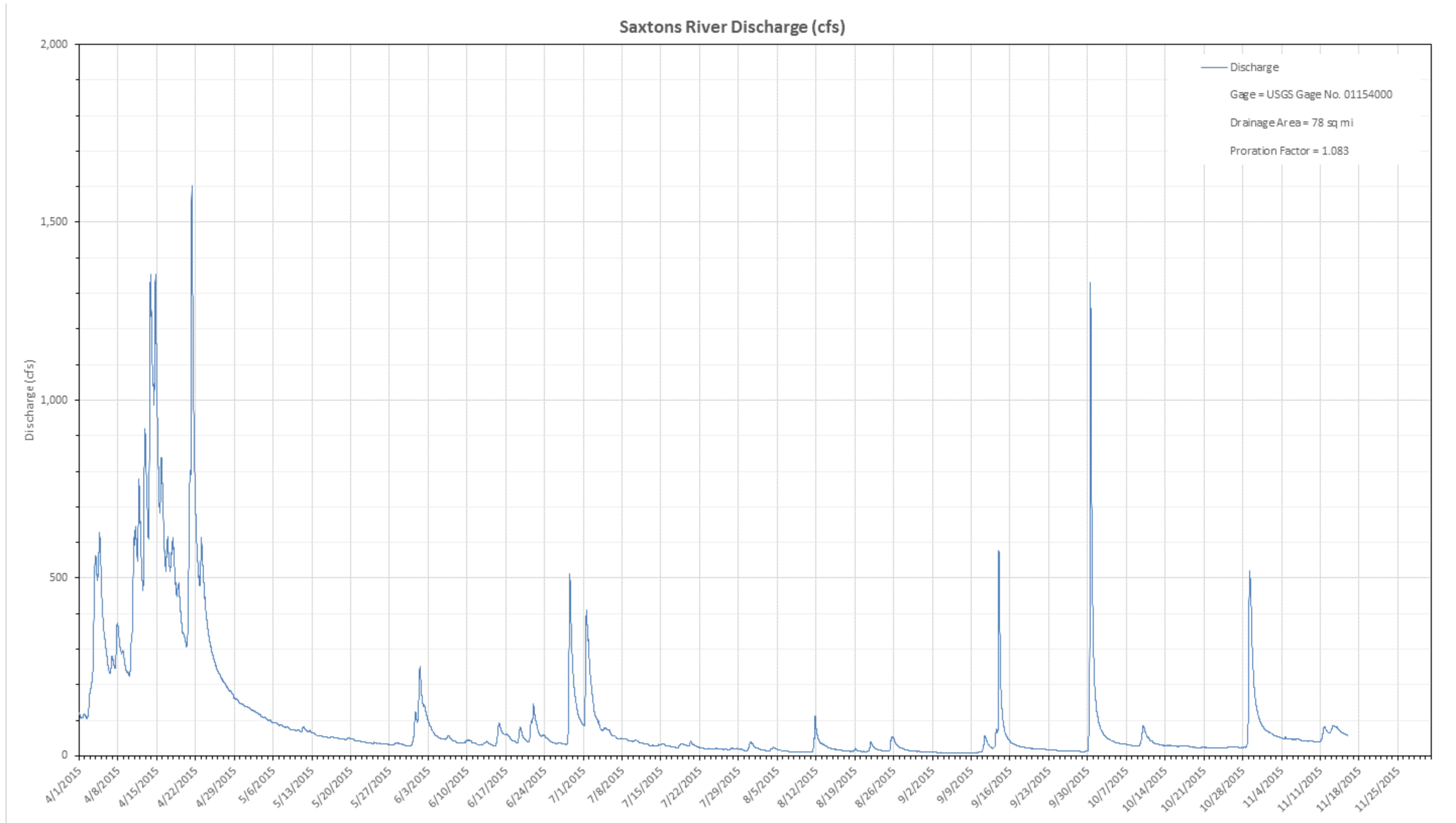
Figure C-8. 2015 Saxtons River hydrograph of the study period from April 1 through November 15. Discharges estimated based on prorated flow at USGS Gage No. 01154000.
