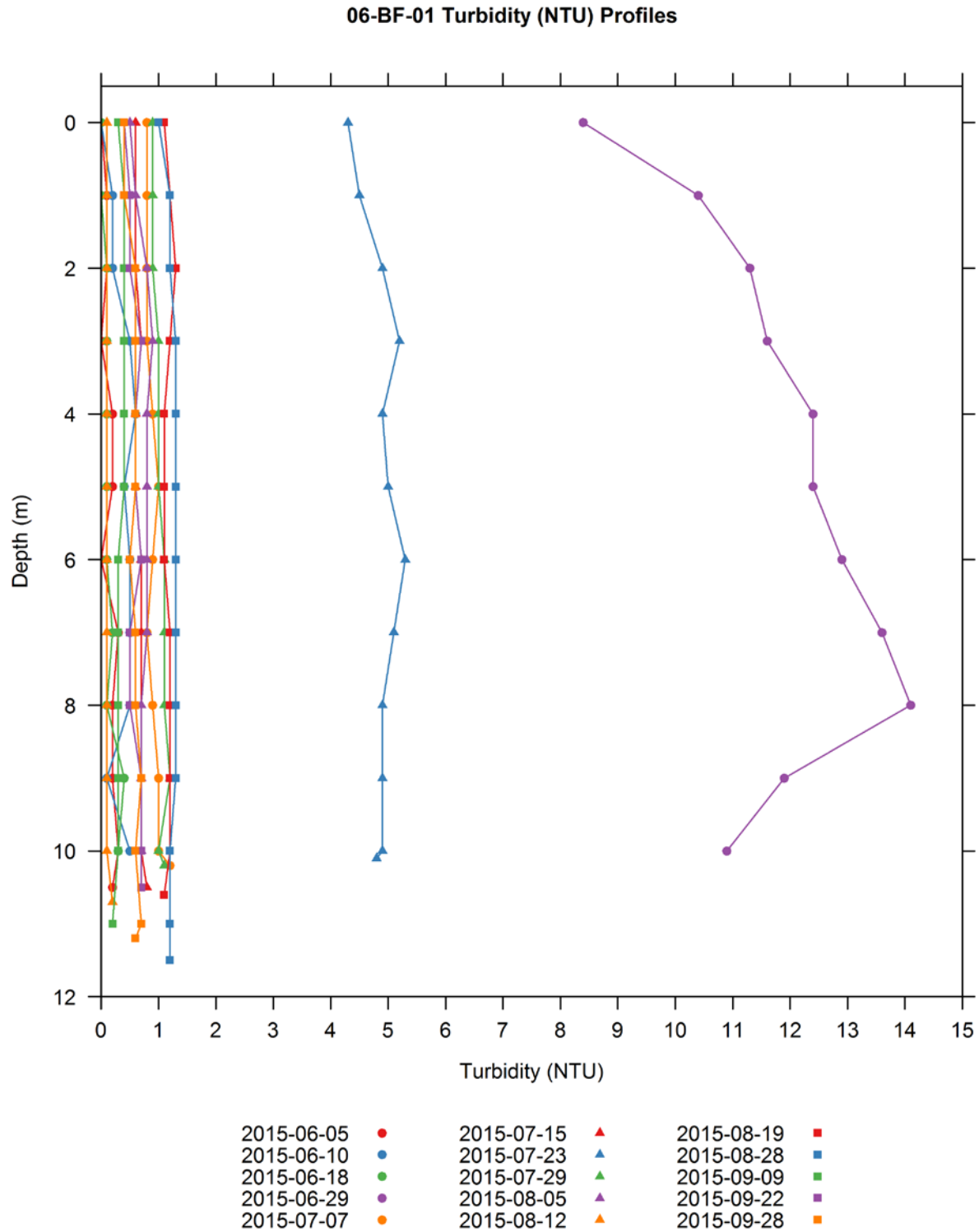
Figure H-54. Vertical profiles of NTU (NTU) collected at the Bellows Falls forebay 06-BF-01 water quality monitoring station.
