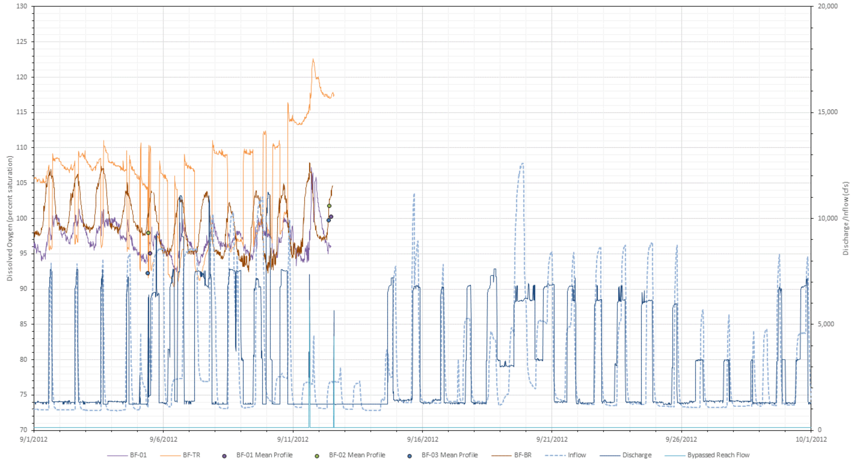
Bellows Falls - September 2012 Dissolved Oxygen (percent saturation)
