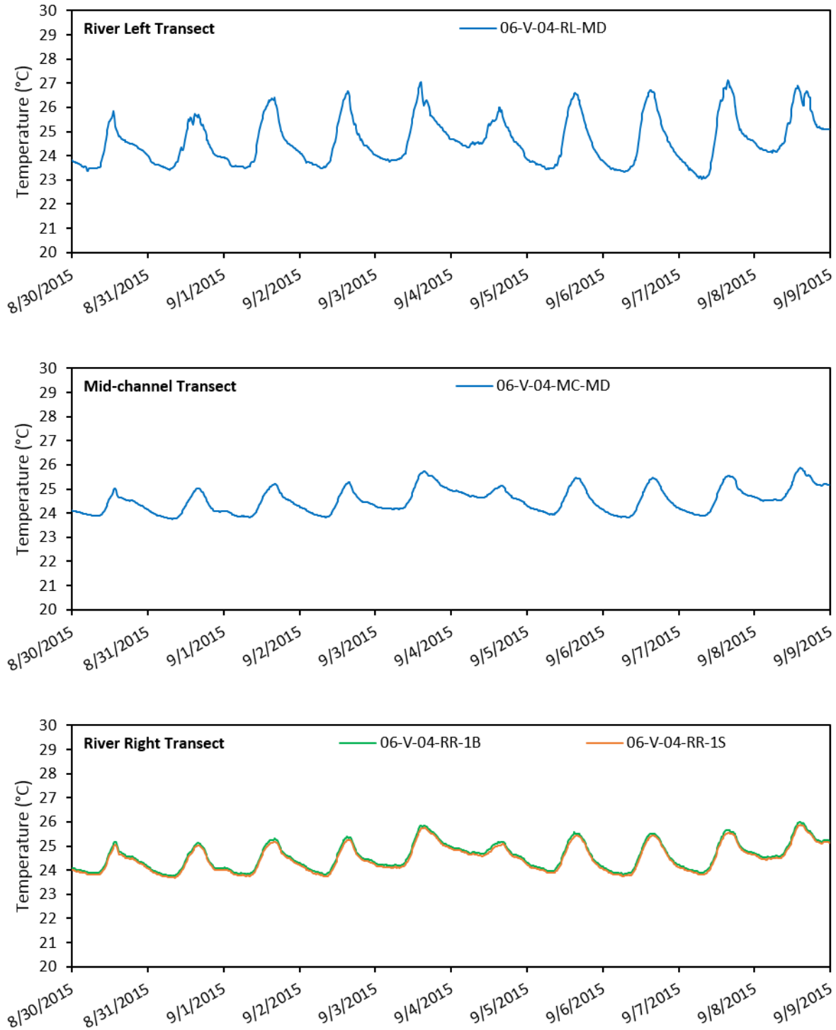
Figure I-9. Continuous water temperature collected at the Vernon 06-V-04 water quality monitoring station during the high temperature low flow monitoring period. Loggers were deployed at one meter below the surface (1S), mid-depth (MD), and one meter above the river bottom (1B).
