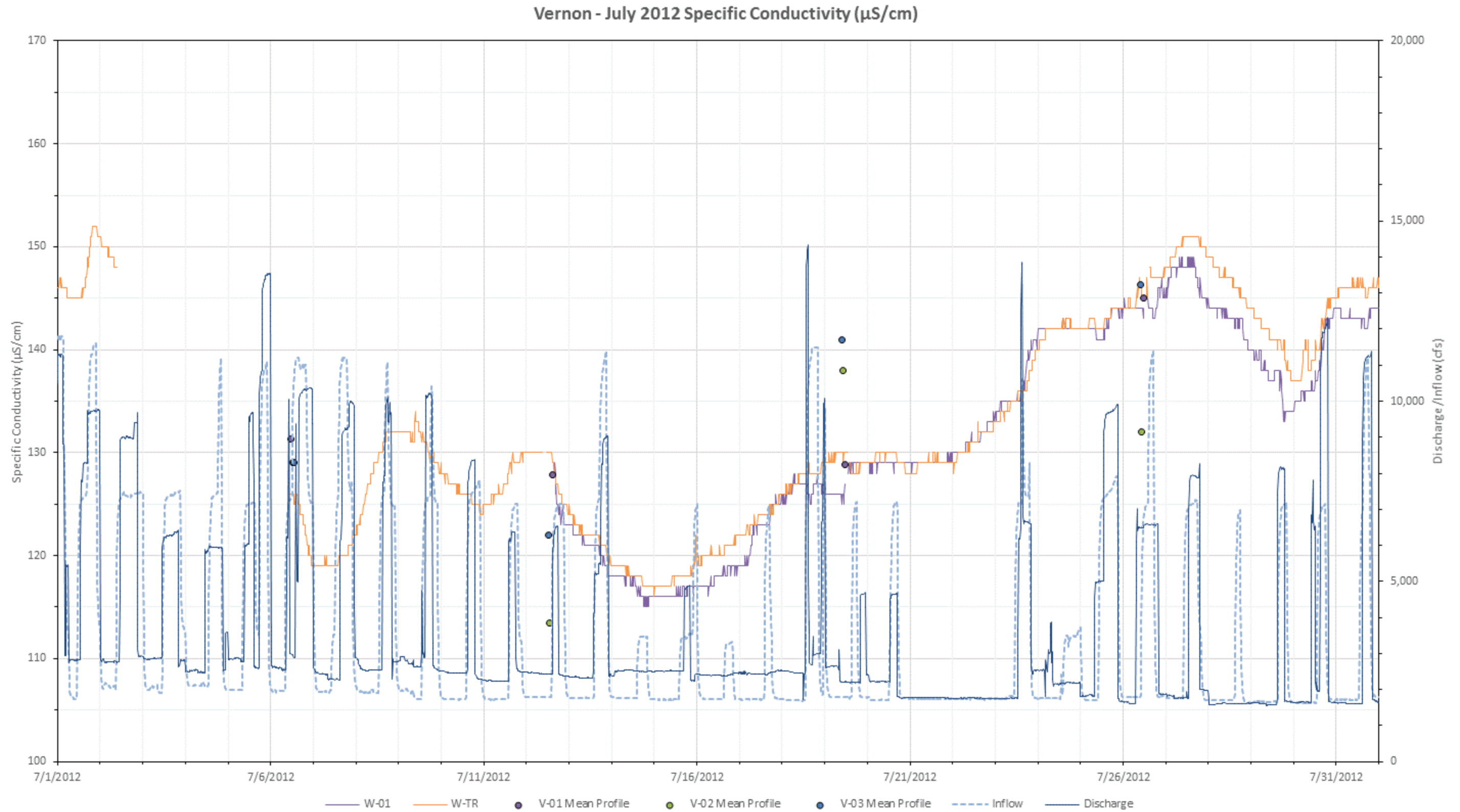
Figure L-58. 2012 July specific conductivity ( \mu\text{S}/\text{cm} ) at all mainstem Vernon stations with inflow (USGS Gage No. 01154500) and Vernon project discharge.
