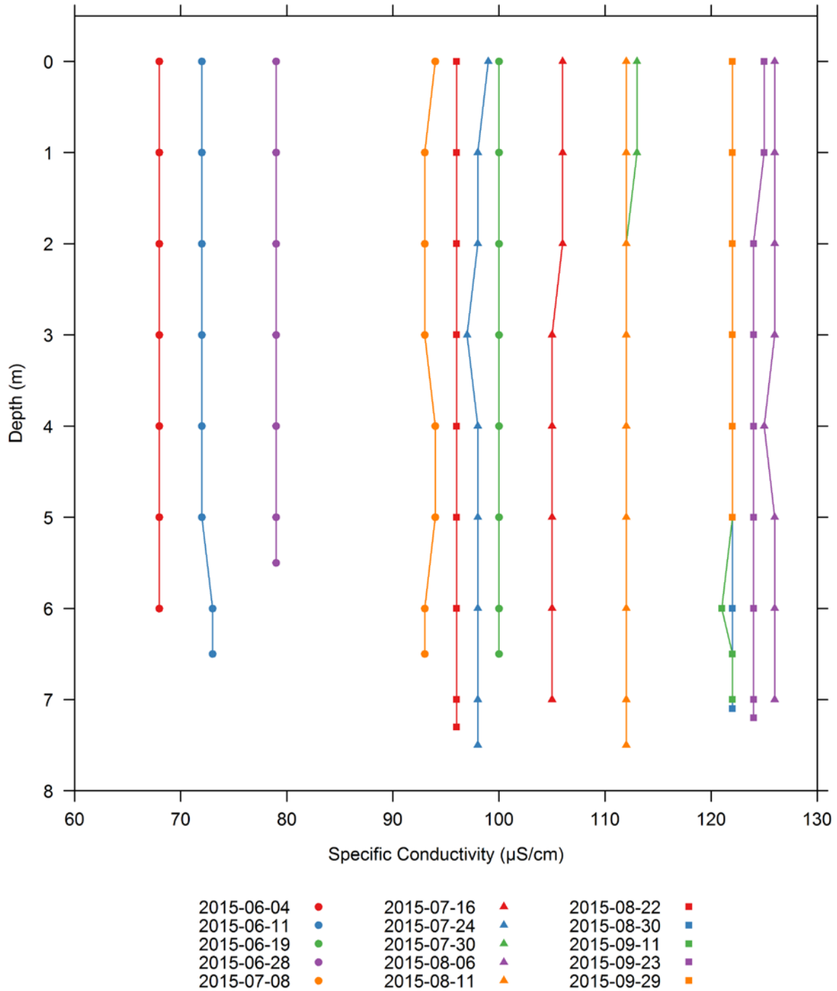
Figure H-16. Vertical profiles of specific conductivity ( \mu\text{S}/\text{cm} ) collected at the Wilder middle impoundment 06-W-02 water quality monitoring station.
