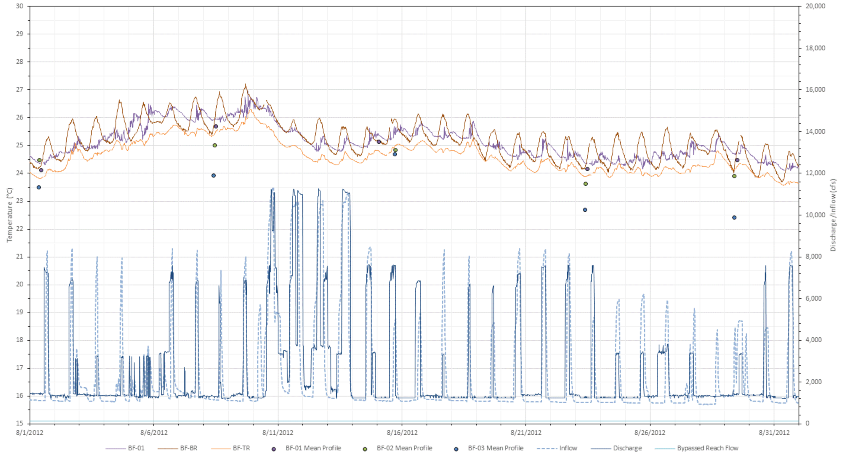
Figure L-7. 2012 August water temperatures at all Bellows Falls stations with inflow (USGS Gage No. 01144500), bypassed reach flow, and Bellows Falls project discharge.
