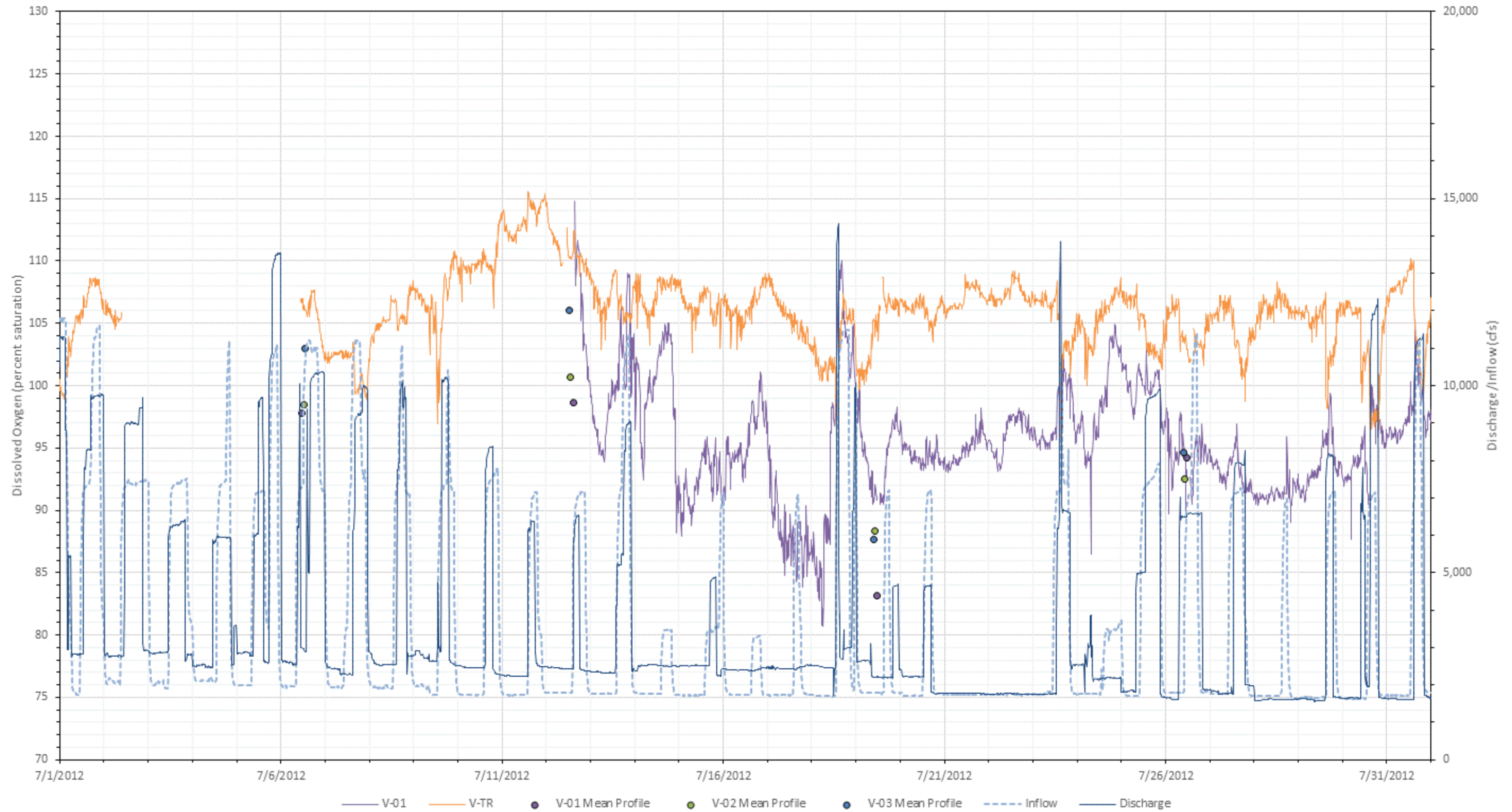
Figure L-34. 2012 July dissolved oxygen (percent saturation) at all mainstem Vernon stations with inflow (USGS Gage No. 01154500) and Vernon project discharge.
