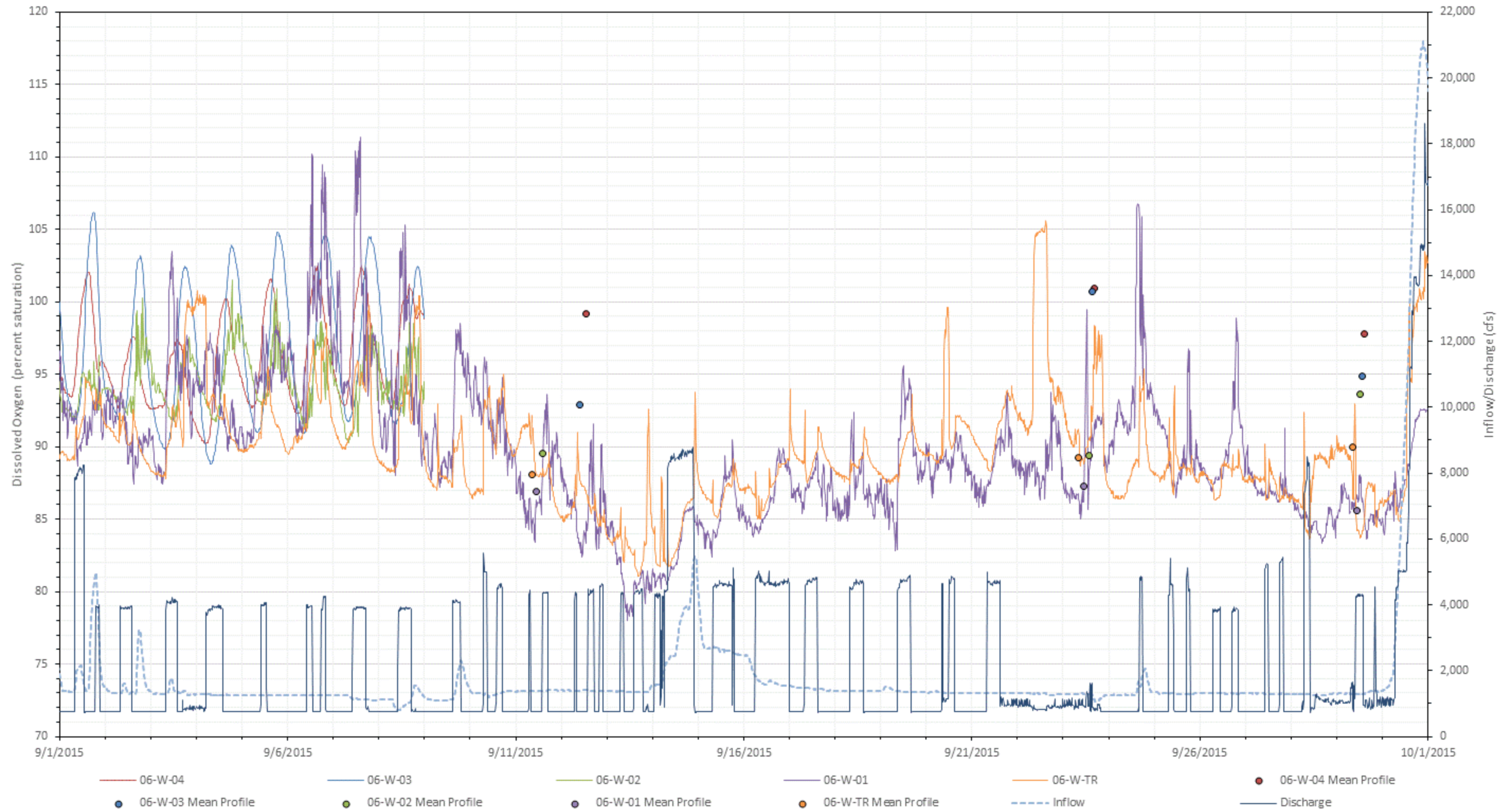
Figure F-39. 2015 September dissolved oxygen (percent saturation) at all Wilder mainstem stations with inflow (USGS Gage No. 01138500) and Wilder project discharge.
