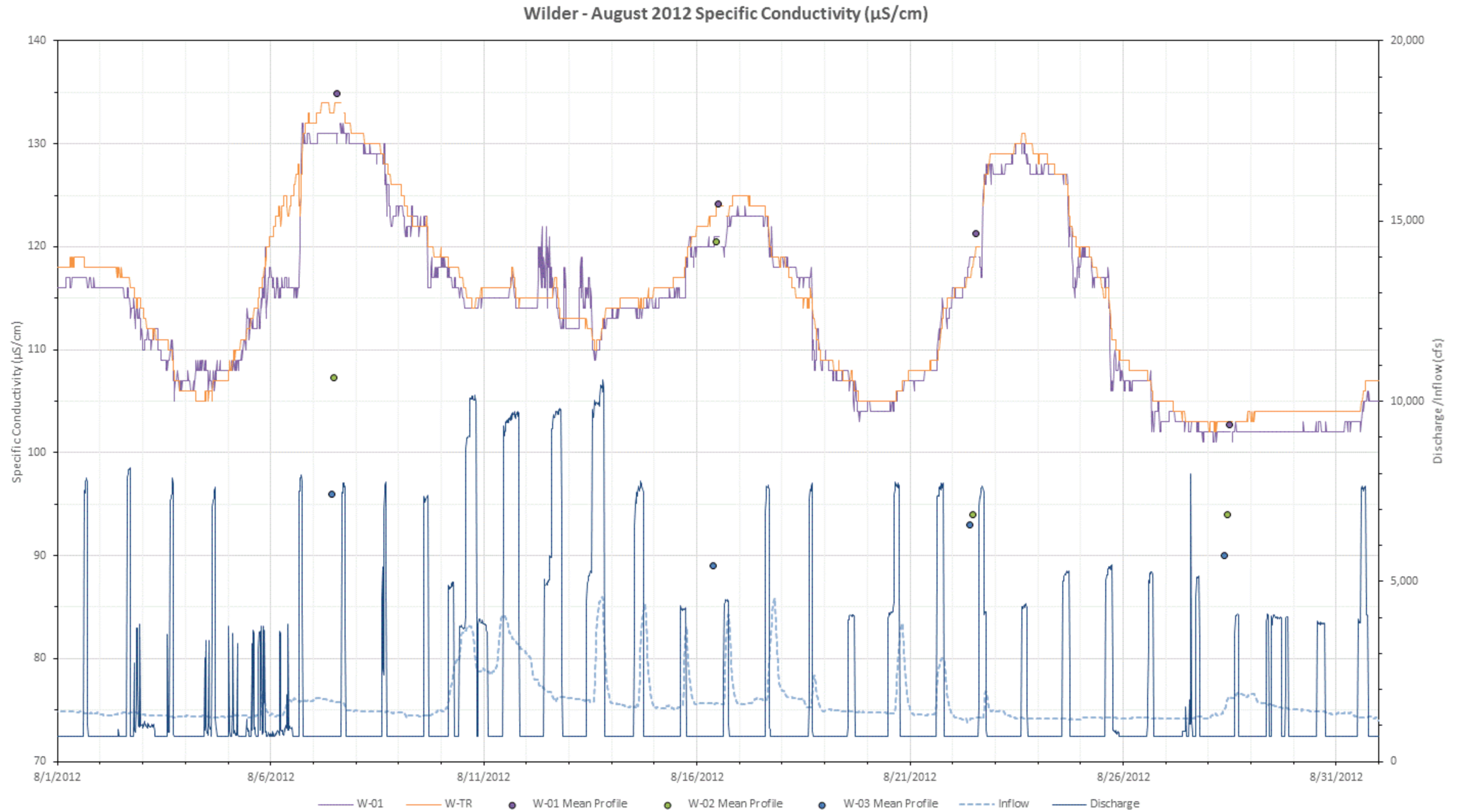
Figure L-51. 2012 August specific conductivity ( \mu\text{S}/\text{cm} ) at all Wilder mainstem stations with inflow (USGS Gage No. 01138500) and Wilder project discharge.
