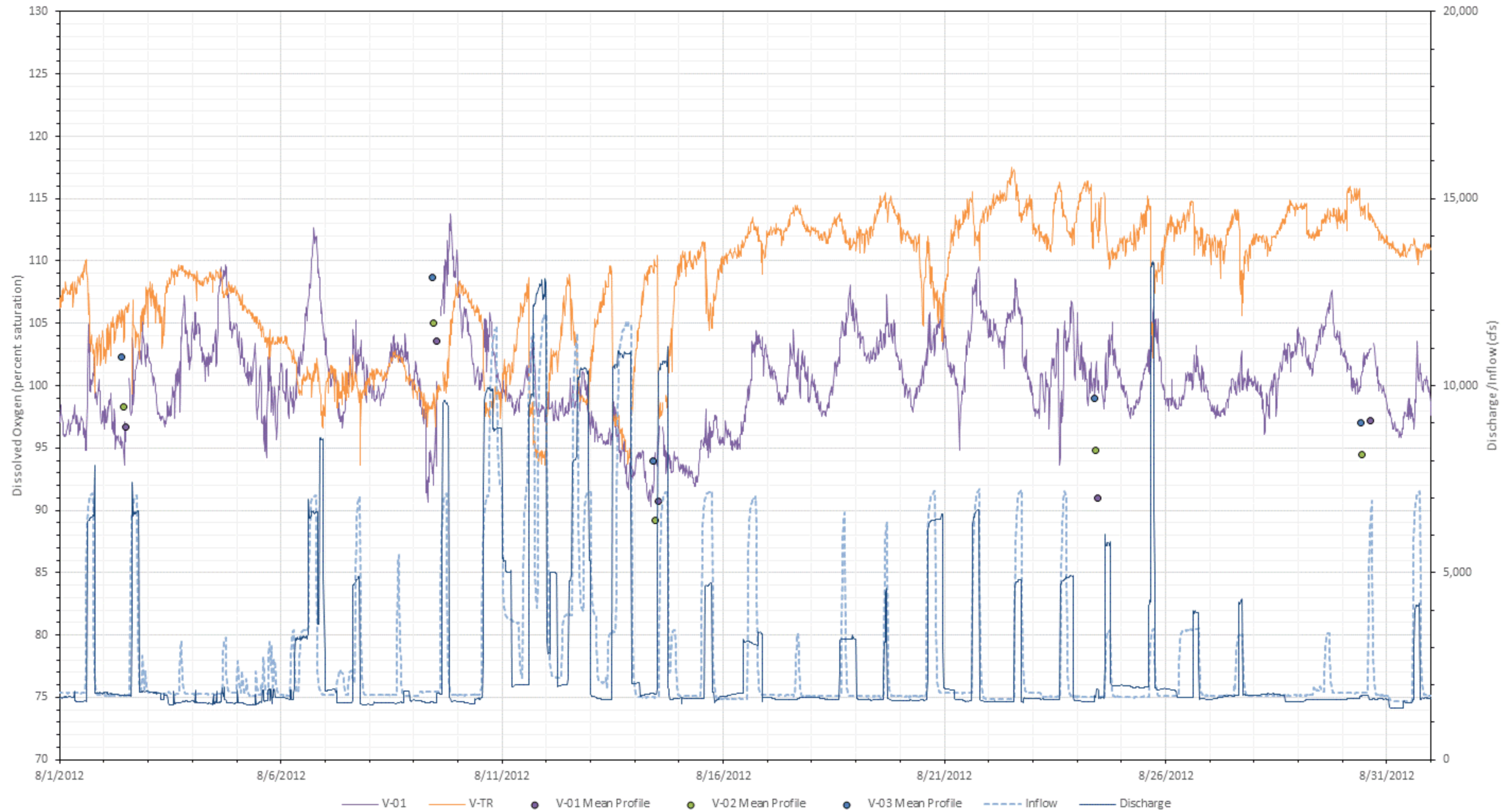
Figure L-35. 2012 August dissolved oxygen (percent saturation) at all mainstem Vernon stations with inflow (USGS Gage No. 01154500) and Vernon project discharge.
