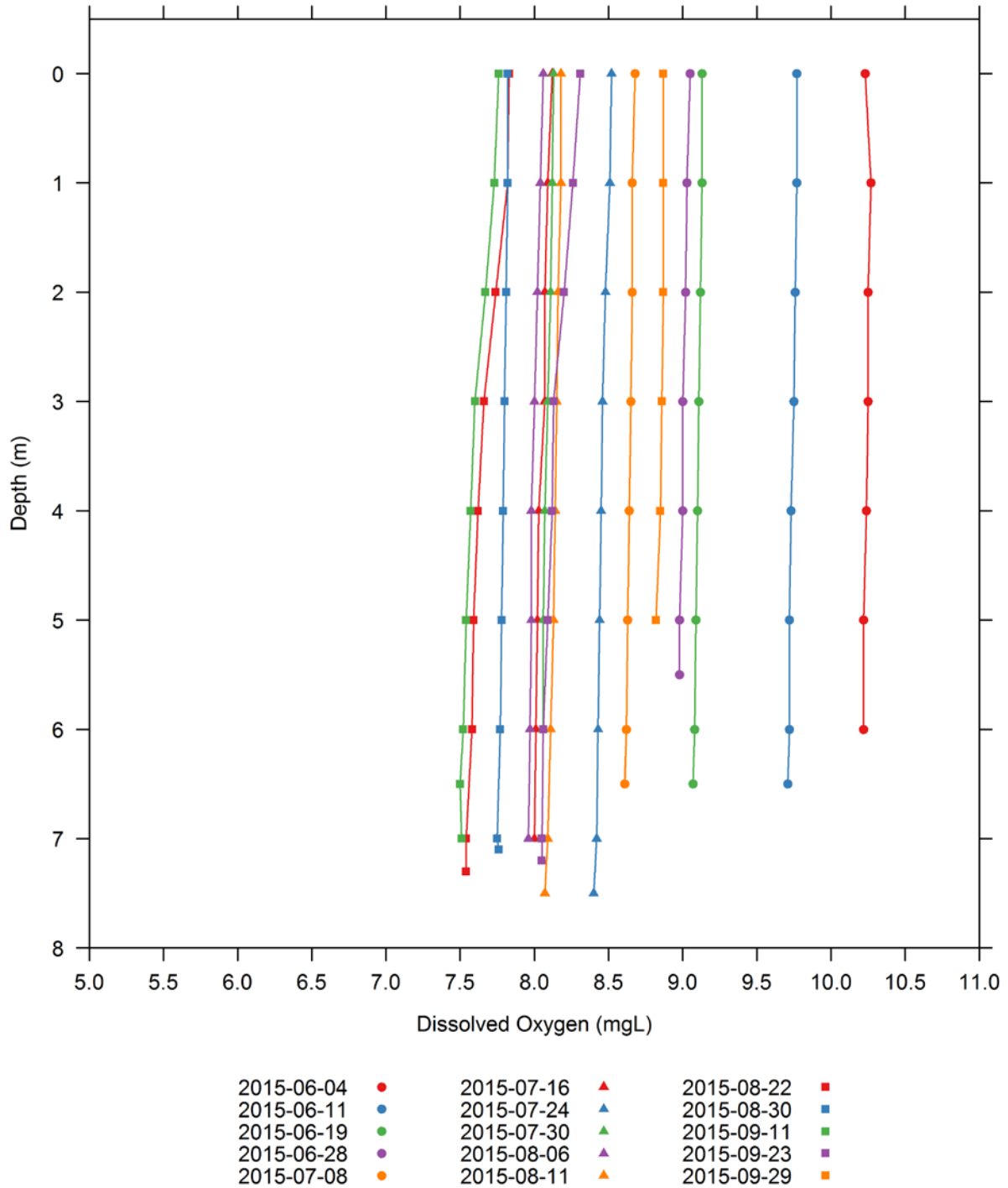
Figure H-14. Vertical profiles of dissolved oxygen (mg/L) collected at the Wilder middle impoundment 06-W-02 water quality monitoring station.
