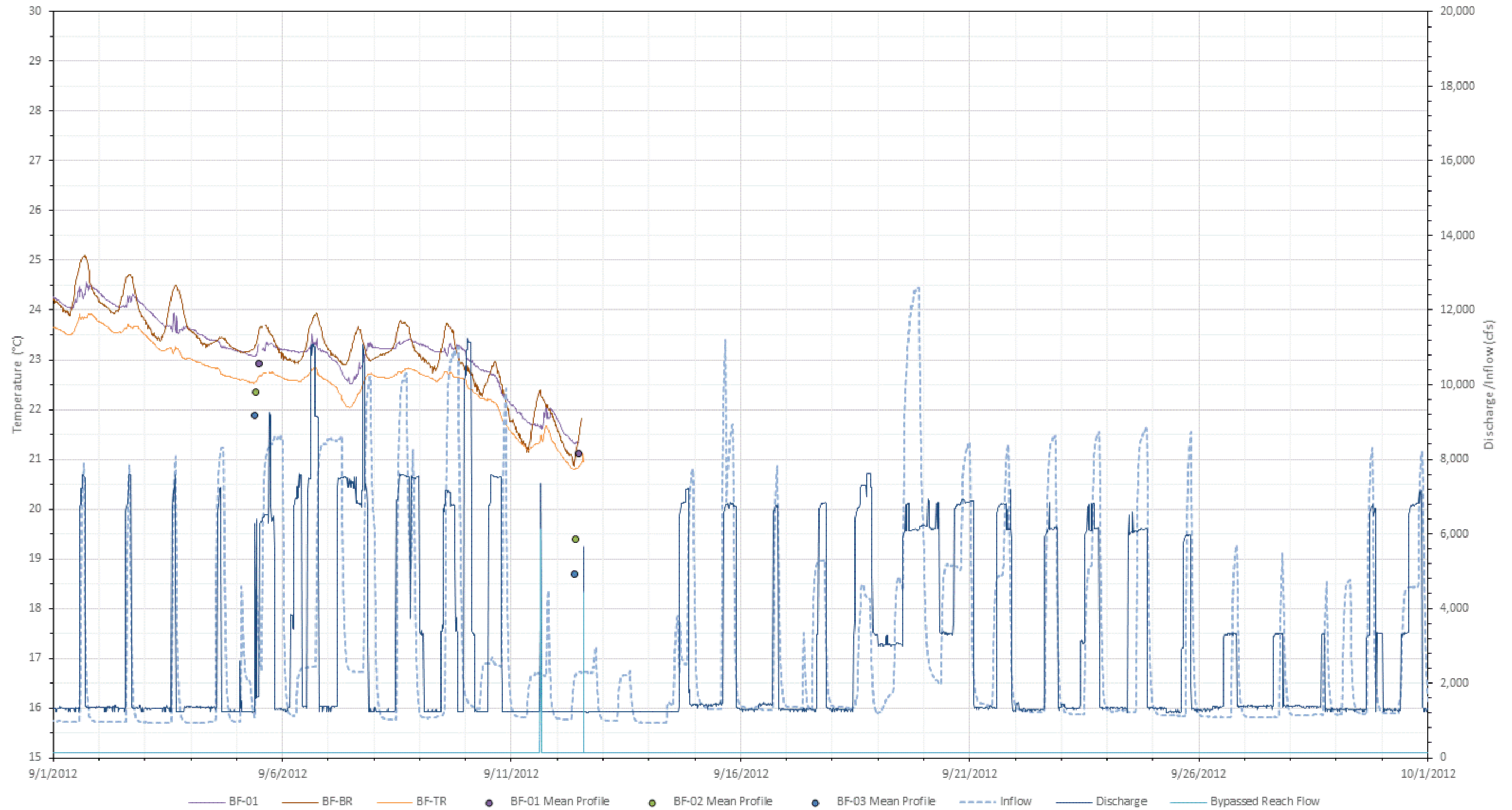
Figure L-8. 2012 September water temperatures at all Bellows Falls stations with inflow (USGS Gage No. 01144500), bypassed reach flow, and Bellows Falls project discharge.
