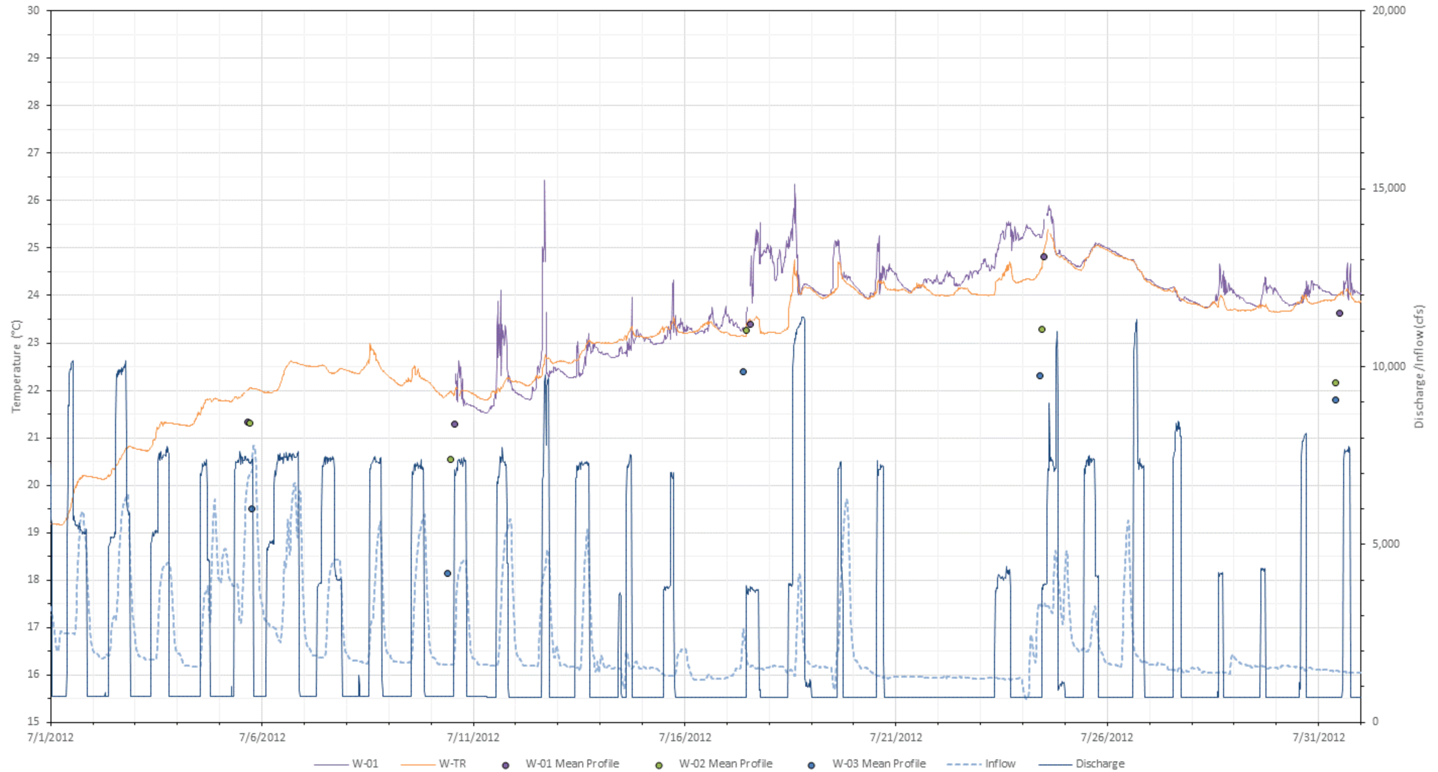
Figure L-2. 2012 July water temperatures at all Wilder stations with inflow (USGS Gage No. 01138500) and Wilder project discharge.
