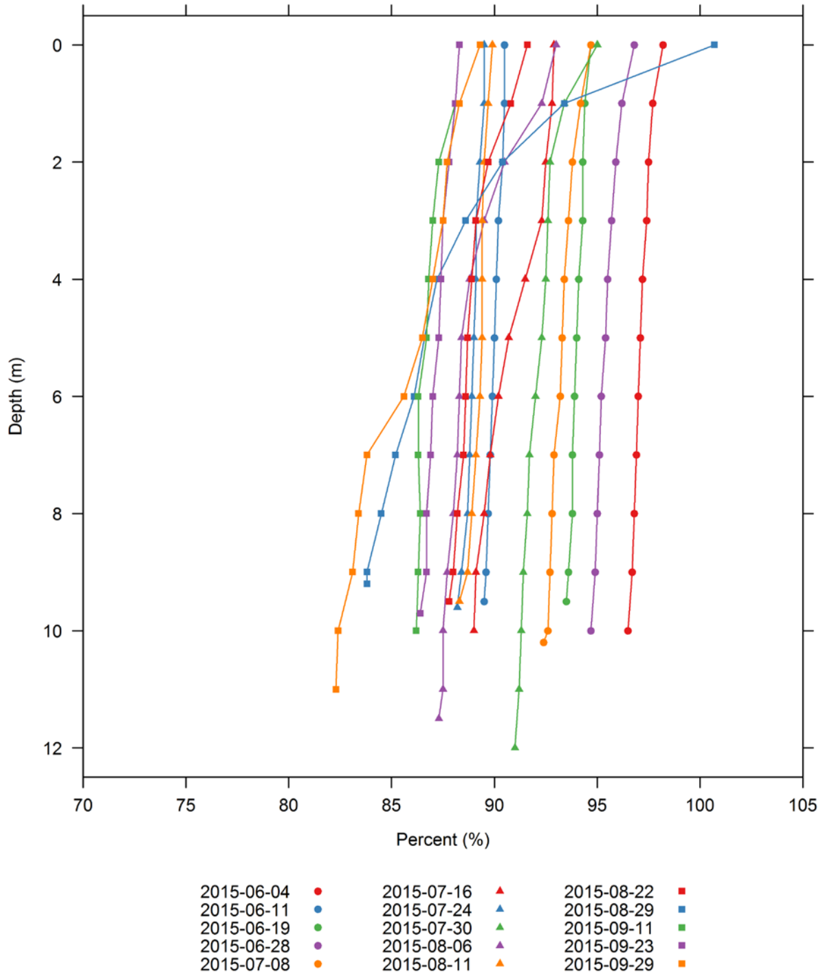
Figure H-21. Vertical profiles of dissolved oxygen (percent saturation) collected at the Wilder forebay 06-W-01 water quality monitoring station.
