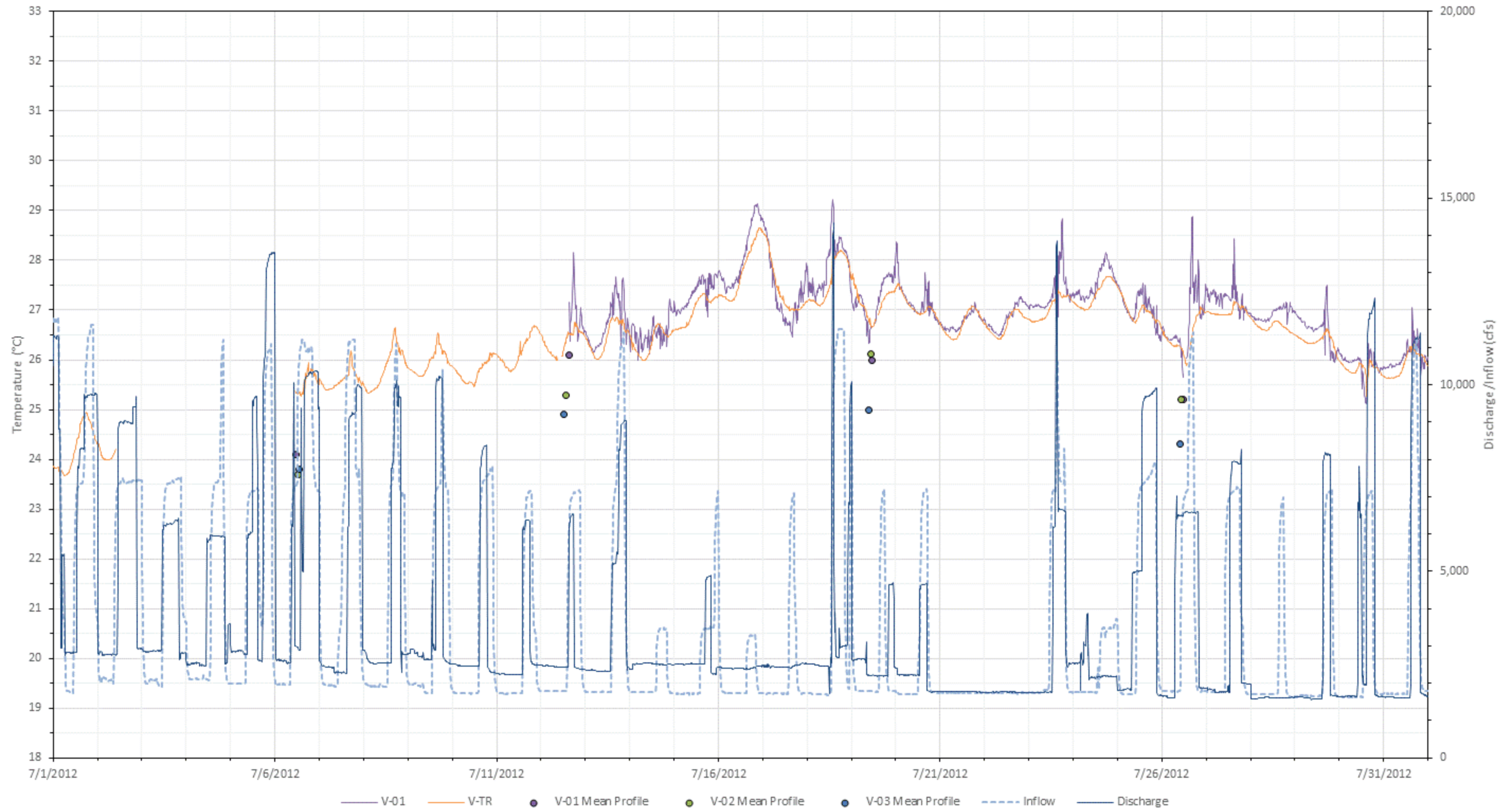
Figure L-10. 2012 July water temperatures at all mainstem Vernon stations with inflow (USGS Gage No. 01154500) and Vernon project discharge.
