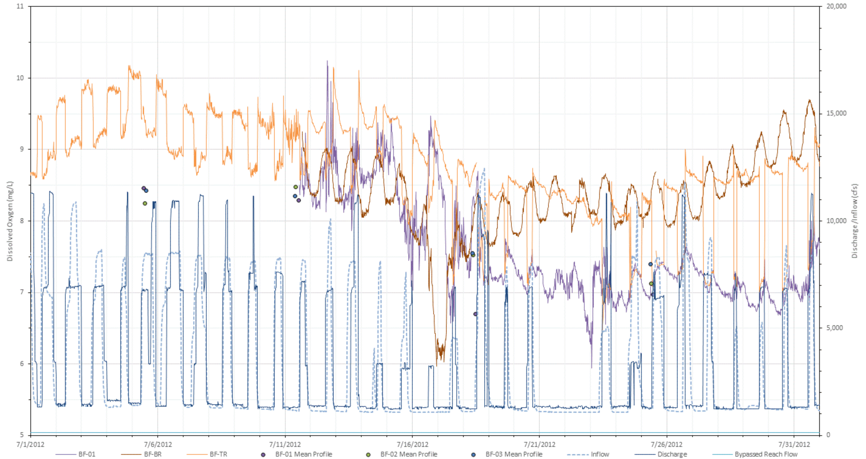
Figure L-18. 2012 July dissolved oxygen (mg/L) at all Bellows Falls stations with inflow (USGS Gage No. 01144500), bypassed reach flow, and Bellows Falls project discharge.
