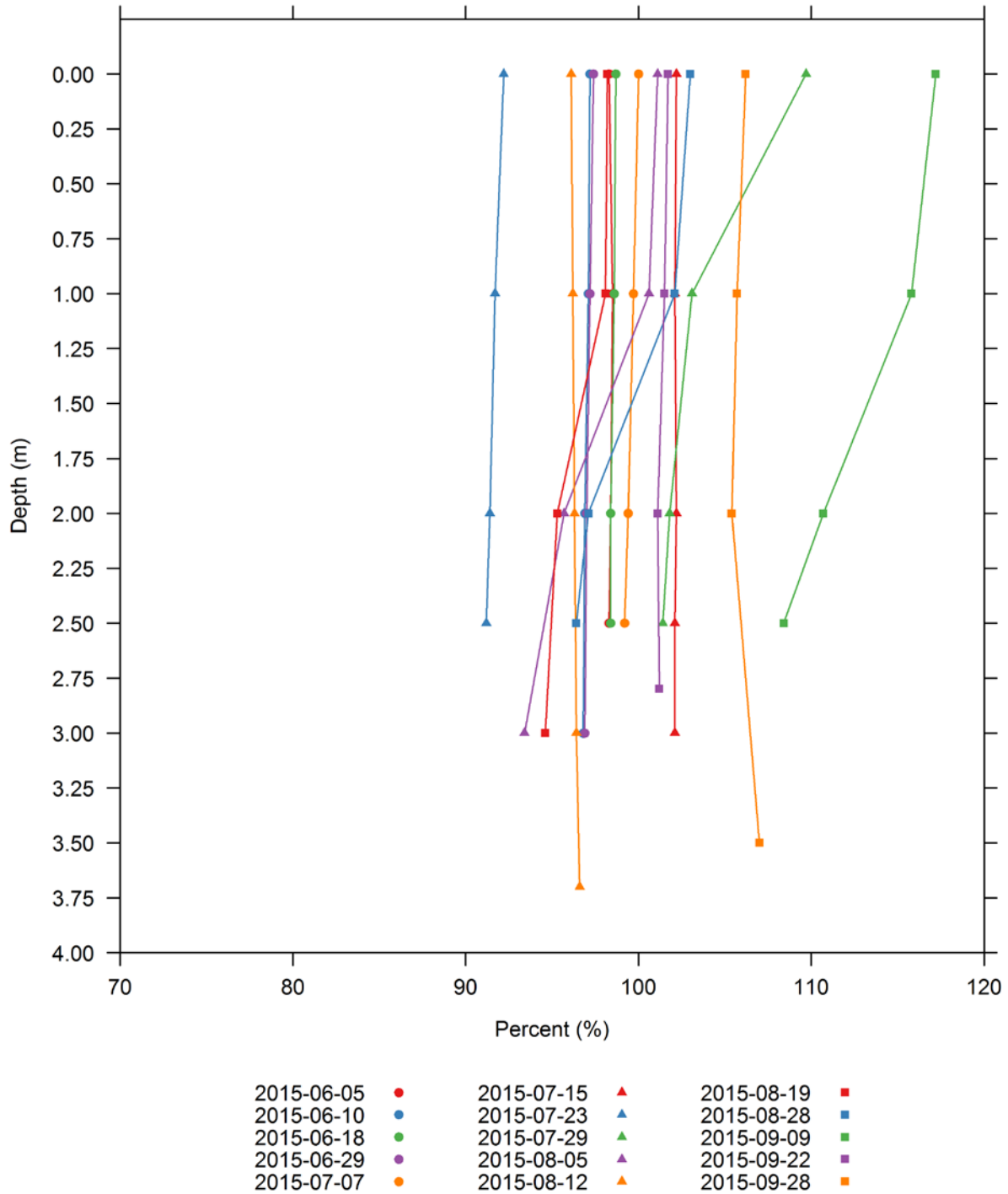
Figure H-45. Vertical profiles of dissolved oxygen (percent saturation) collected at the Bellows Falls middle impoundment 06-BF-02 water quality monitoring station.
