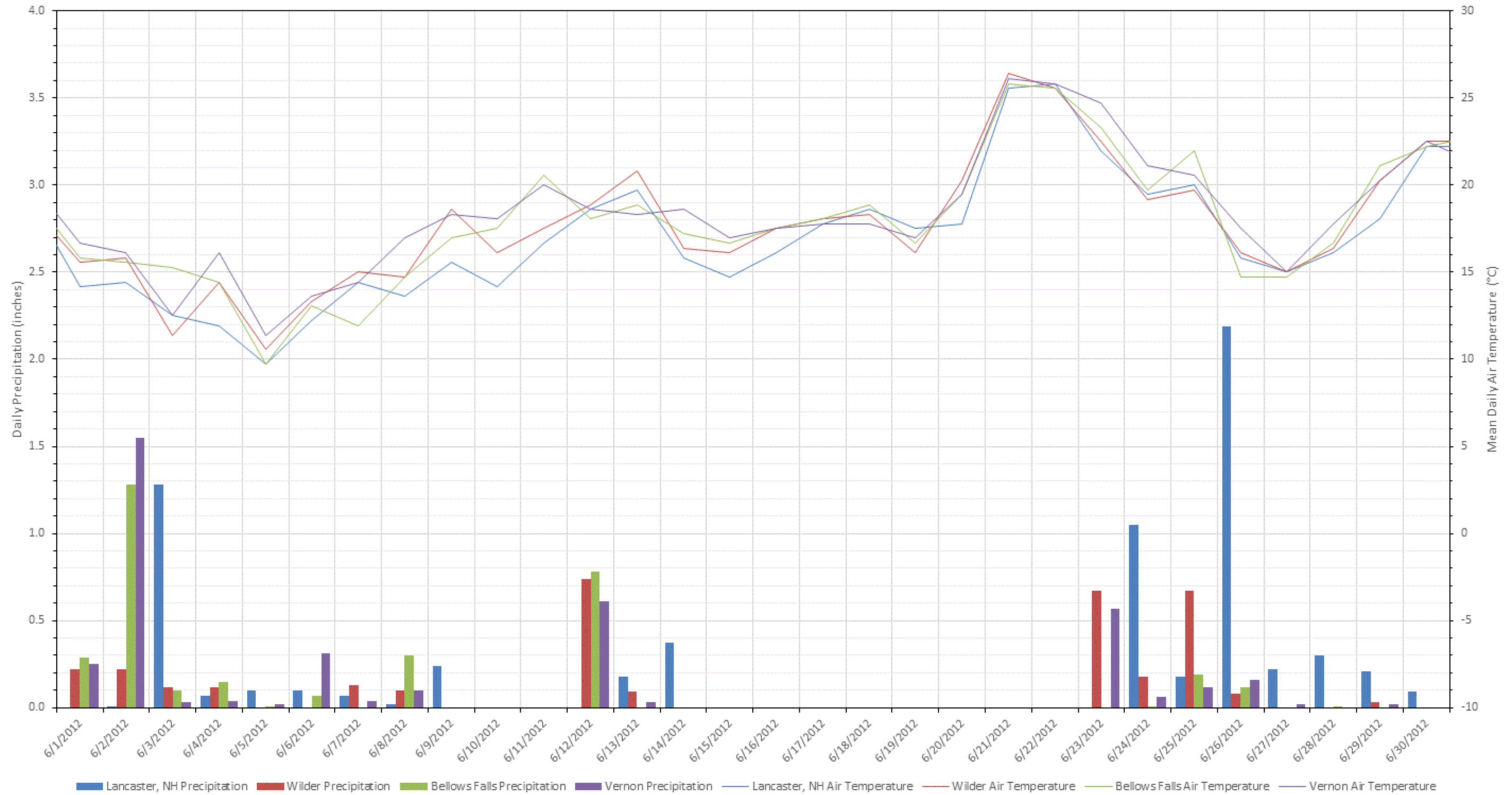
Figure M-1. 2012 June daily mean air temperature (°C) and daily precipitation (inches) for the study area.
