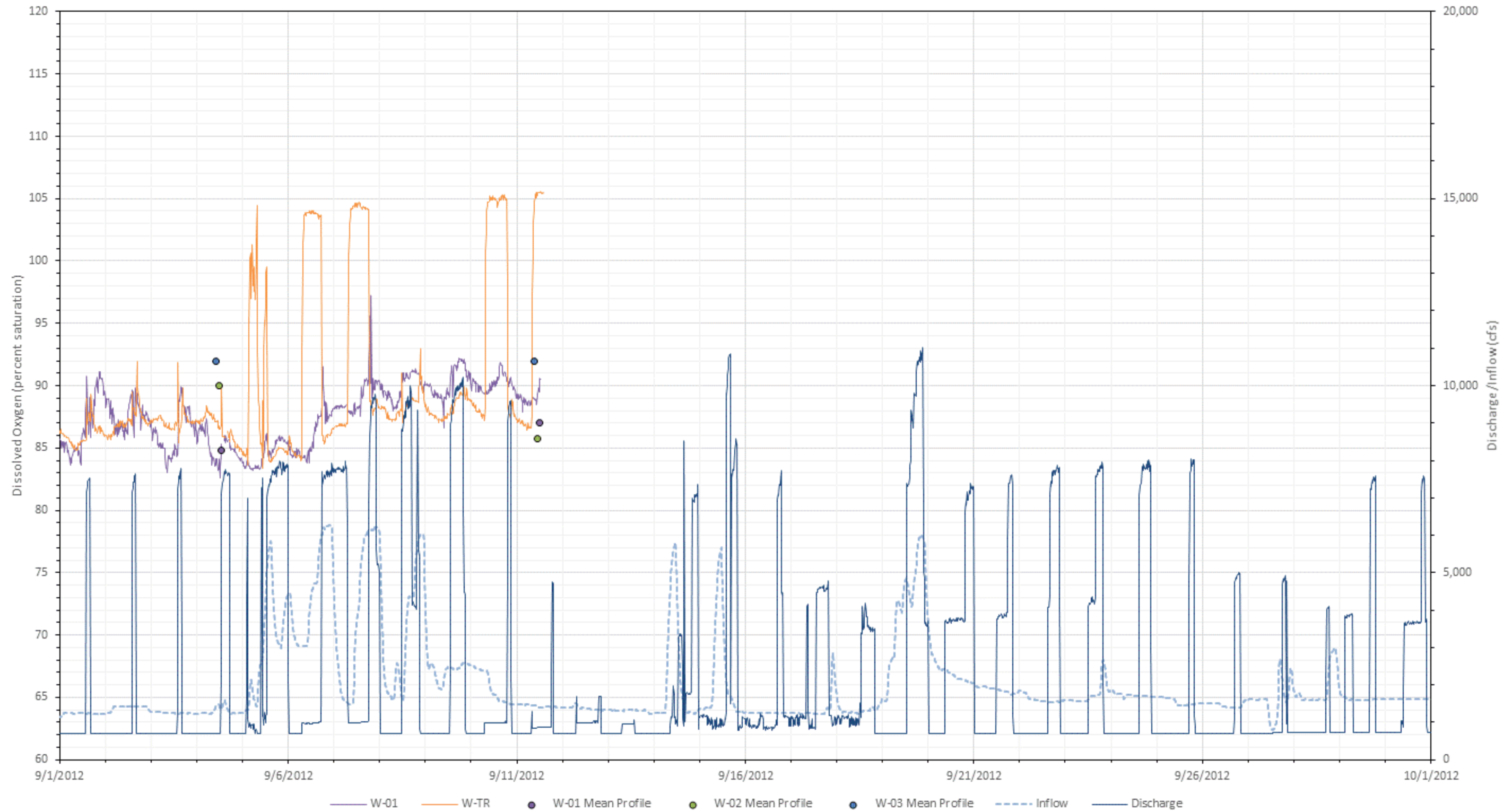
Figure L-28. 2012 September dissolved oxygen (percent saturation) at all Wilder mainstem stations with inflow (USGS Gage No. 01138500) and Wilder project discharge.
