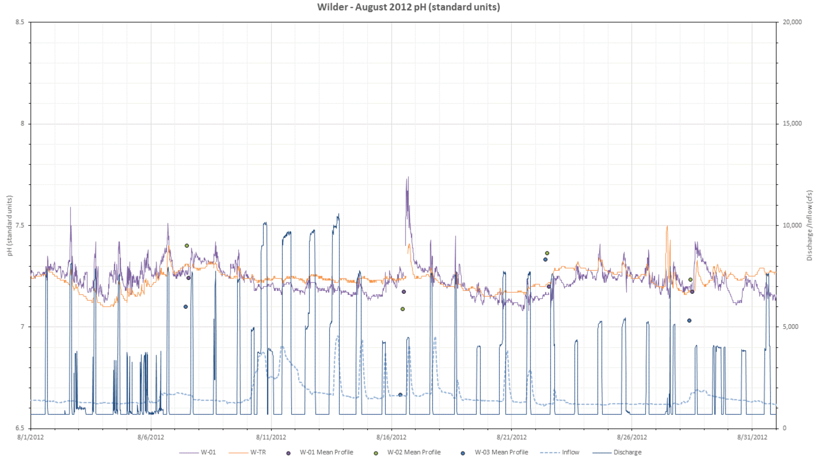
Figure L-39. 2012 August pH (standard units) at all Wilder mainstem stations with inflow (USGS Gage No. 01138500) and Wilder project discharge.
