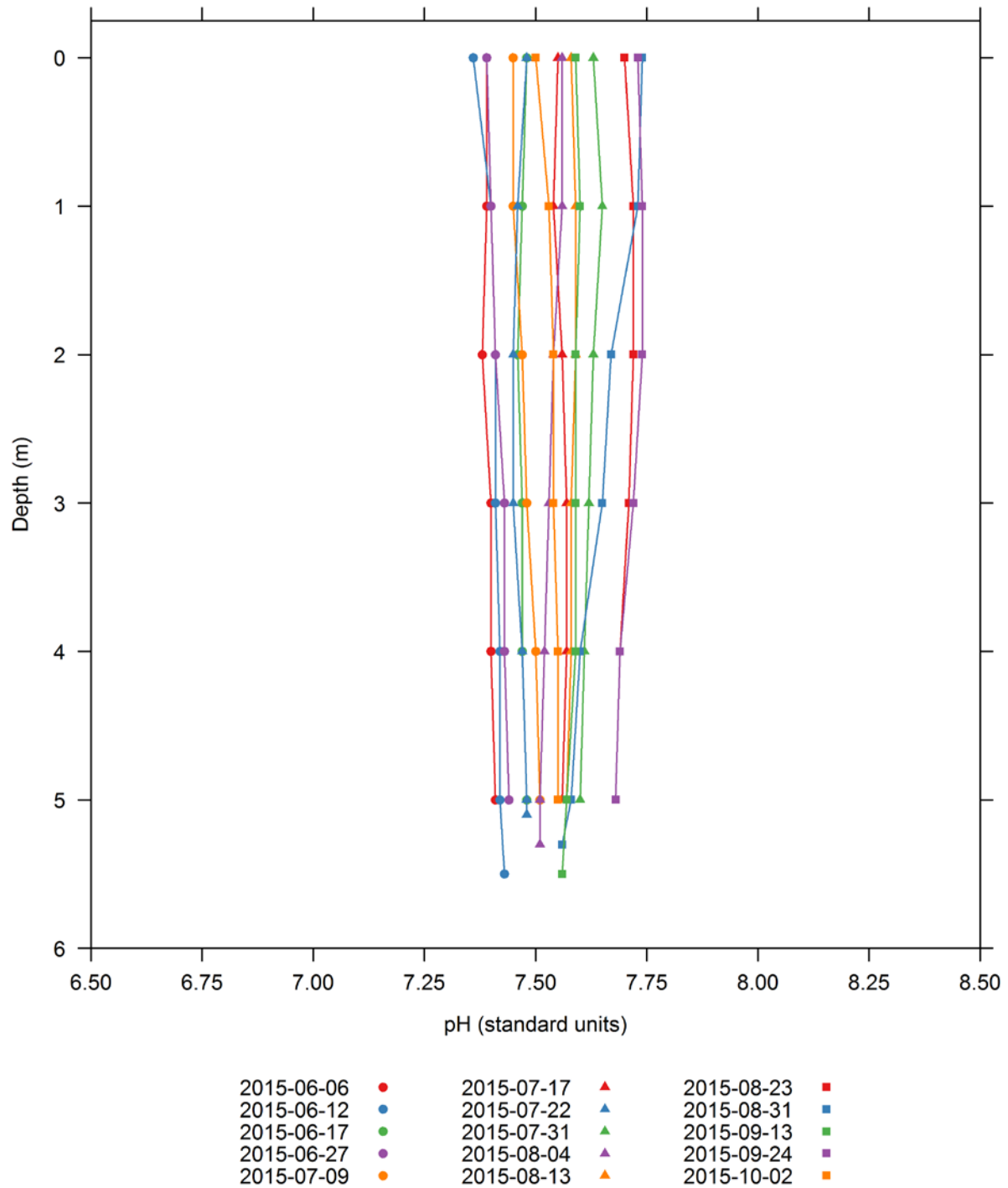
Figure H-77. Vertical profiles of pH (standard units) collected at the Vernon middle impoundment 06-V-02 water quality monitoring station.
