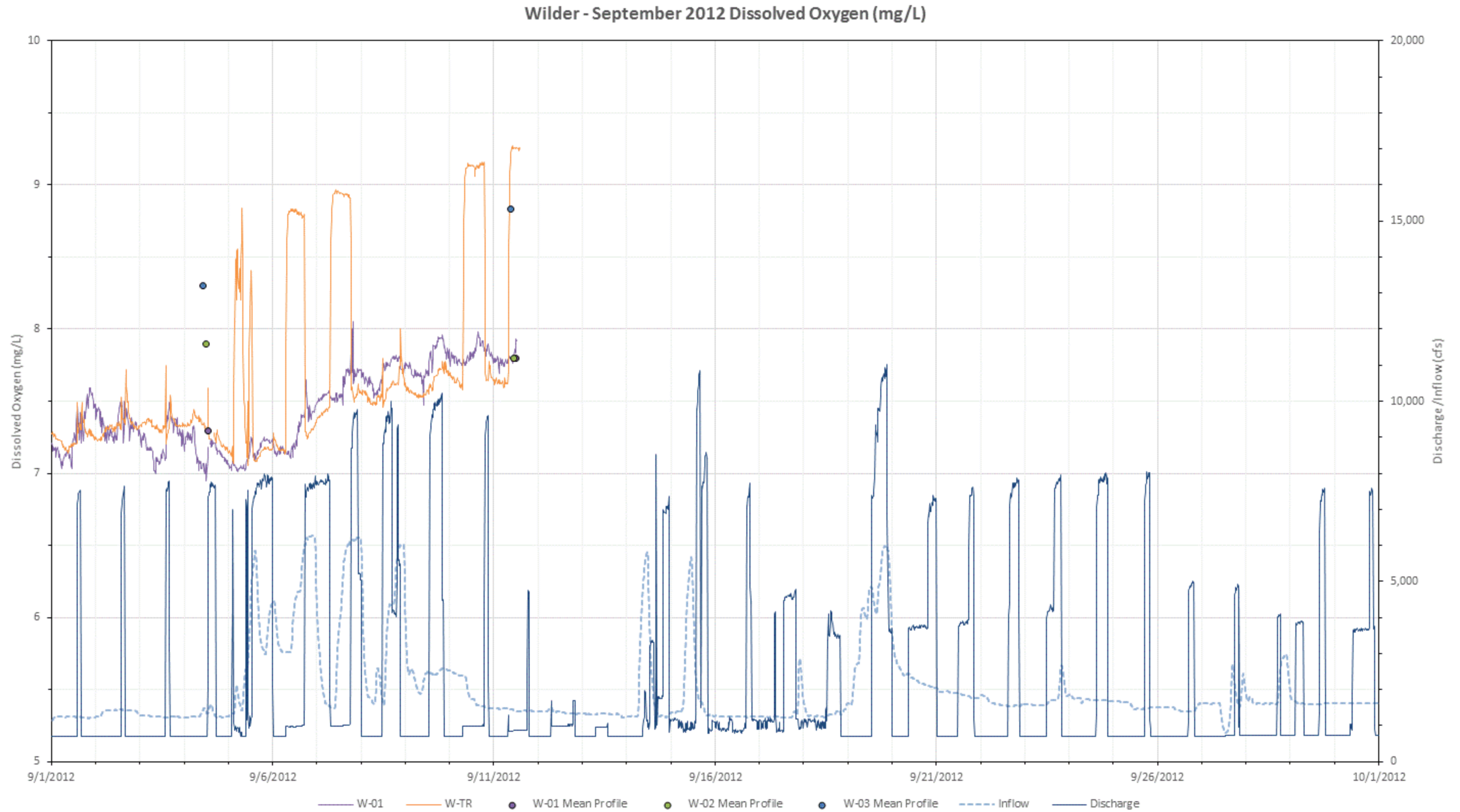
Figure L-16. 2012 September dissolved oxygen (mg/L) at all Wilder mainstem stations with inflow (USGS Gage No. 01138500) and Wilder project discharge.
