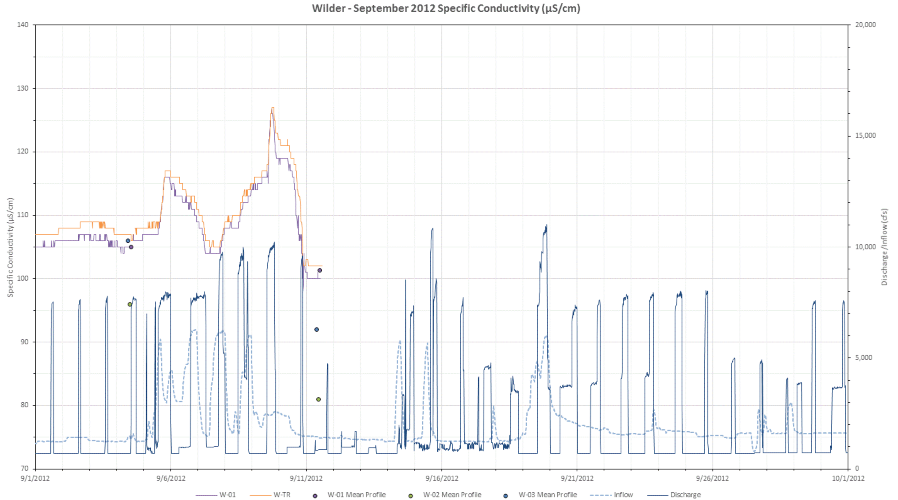
Figure L-52. 2012 September specific conductivity ( \mu\text{S}/\text{cm} ) at all Wilder mainstem stations with inflow (USGS Gage No. 01138500) and Wilder project discharge.
