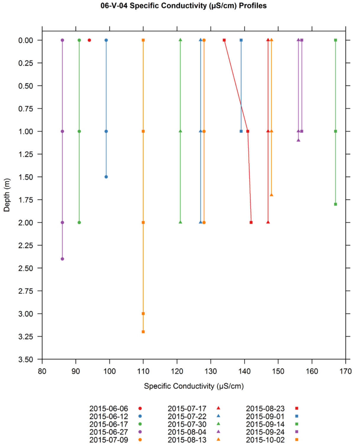
Figure H-64. Vertical profiles of specific conductivity ( \mu\text{S}/\text{cm} ) collected at the Vernon upstream 06-V-04 water quality monitoring station.
