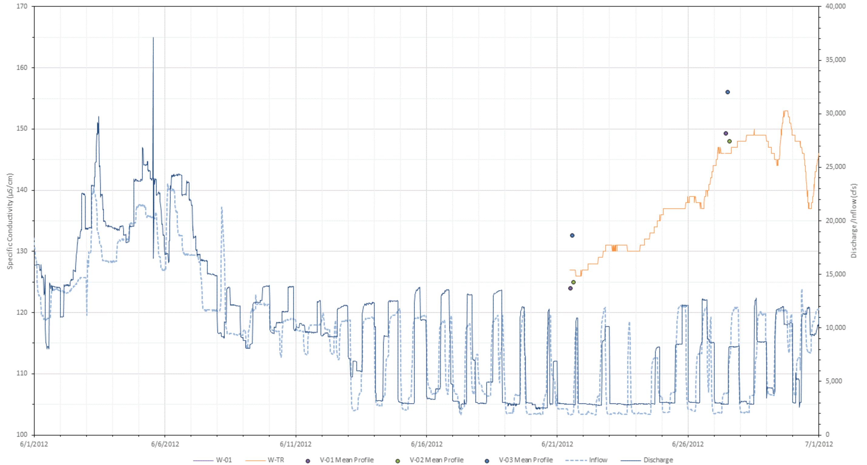
Figure L-57. 2012 June specific conductivity ( \mu\text{S}/\text{cm} ) at all mainstem Vernon stations with inflow (USGS Gage No. 01154500) and Vernon project discharge.
