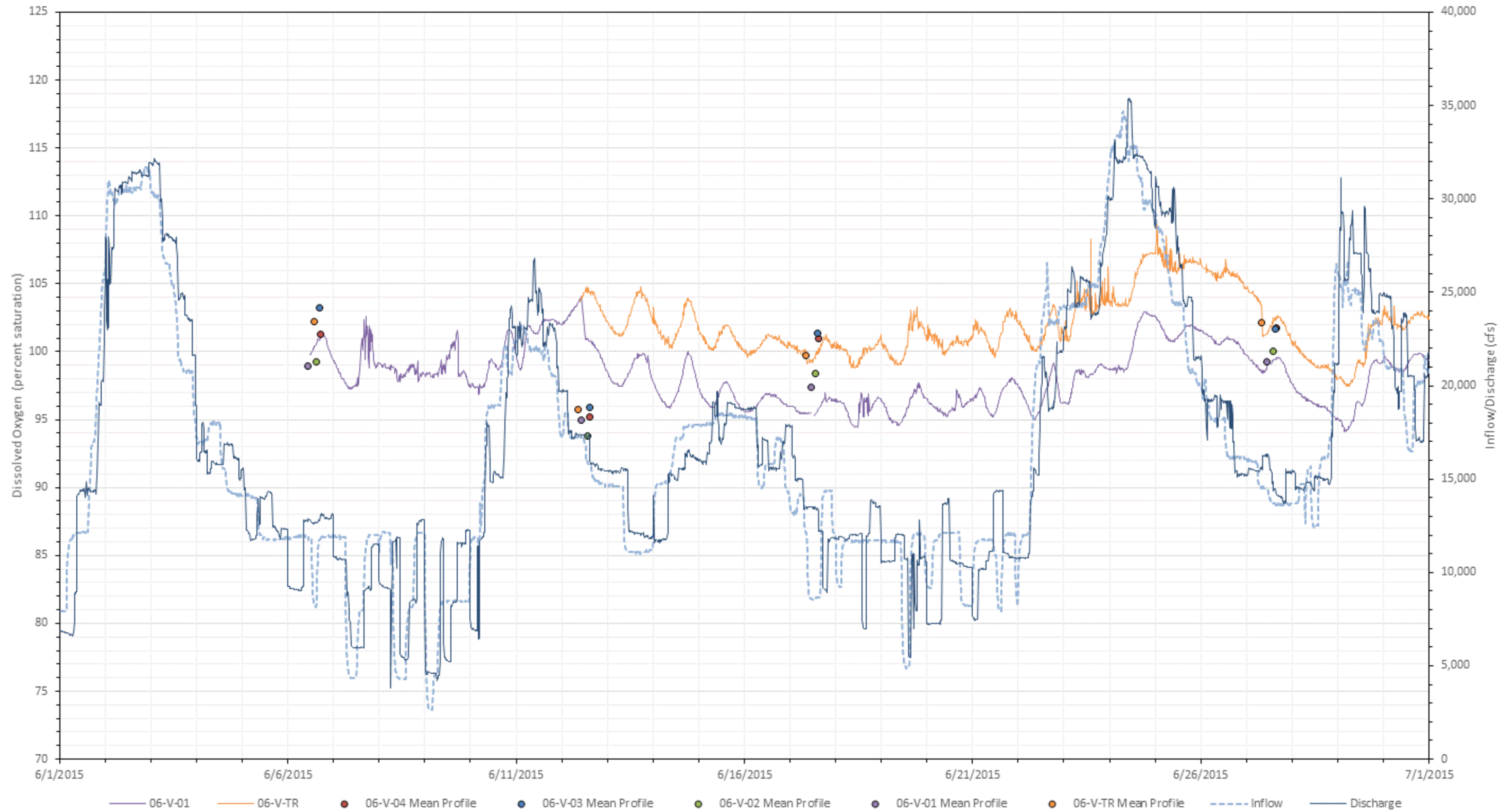
Figure F-44. 2015 June dissolved oxygen (percent saturation) at all mainstem Vernon stations with inflow (USGS Gage No. 01154500) and Vernon project discharge.
