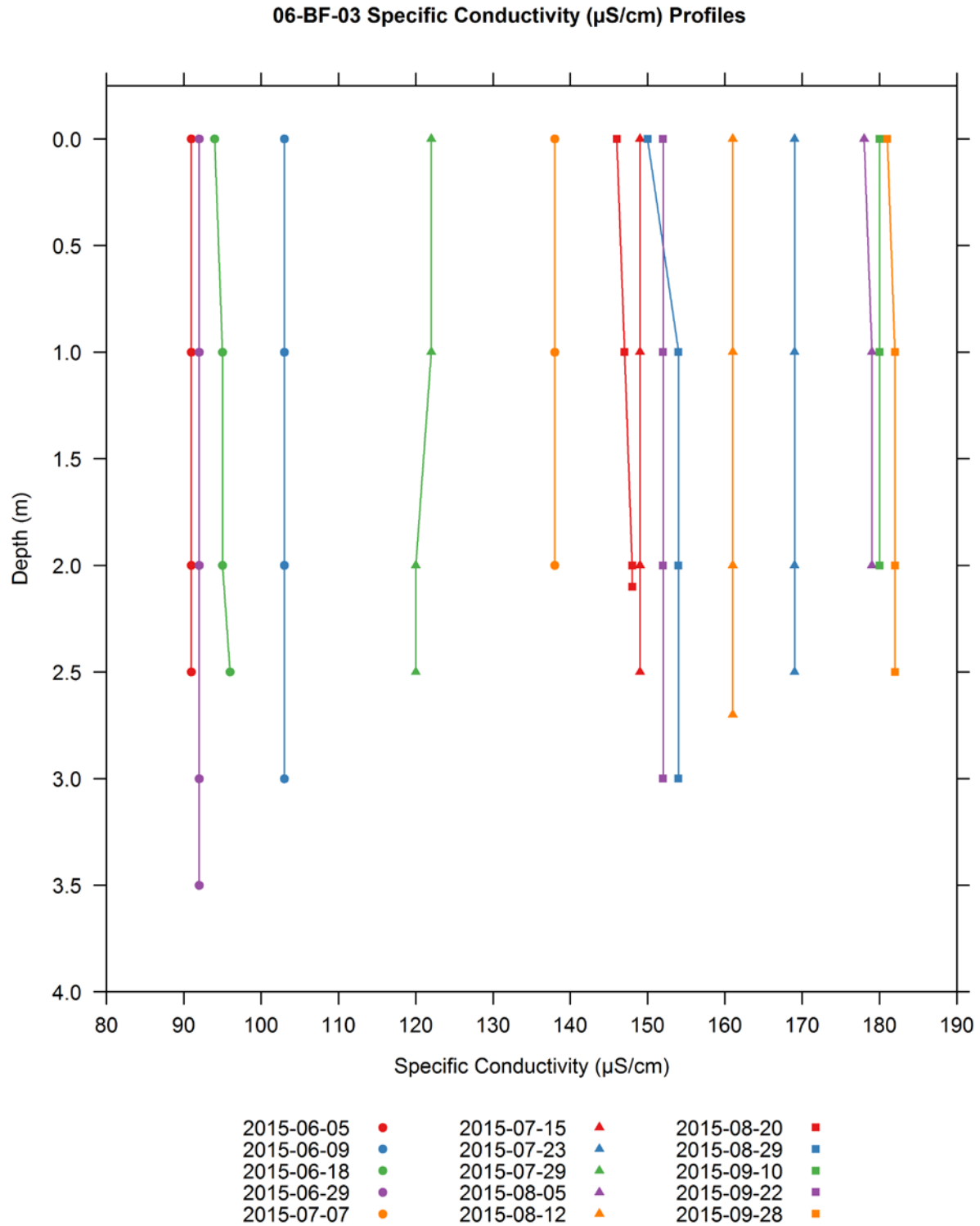
Figure H-40. Vertical profiles of specific conductivity ( \mu\text{S/cm} ) collected at the Bellows Falls upper impoundment 06-BF-03 water quality monitoring station.
