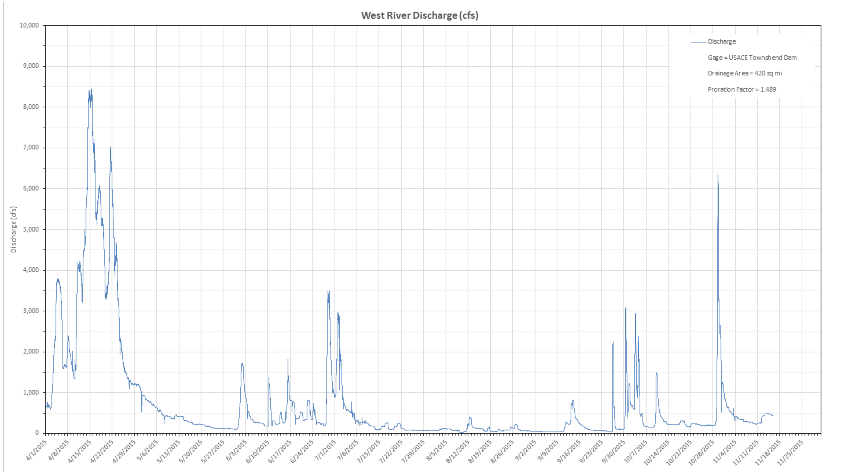
Figure C-10. 2015 West River hydrograph of the study period from April 1 through November 15. Discharges estimated based on prorated flow at Townsend Dam.
