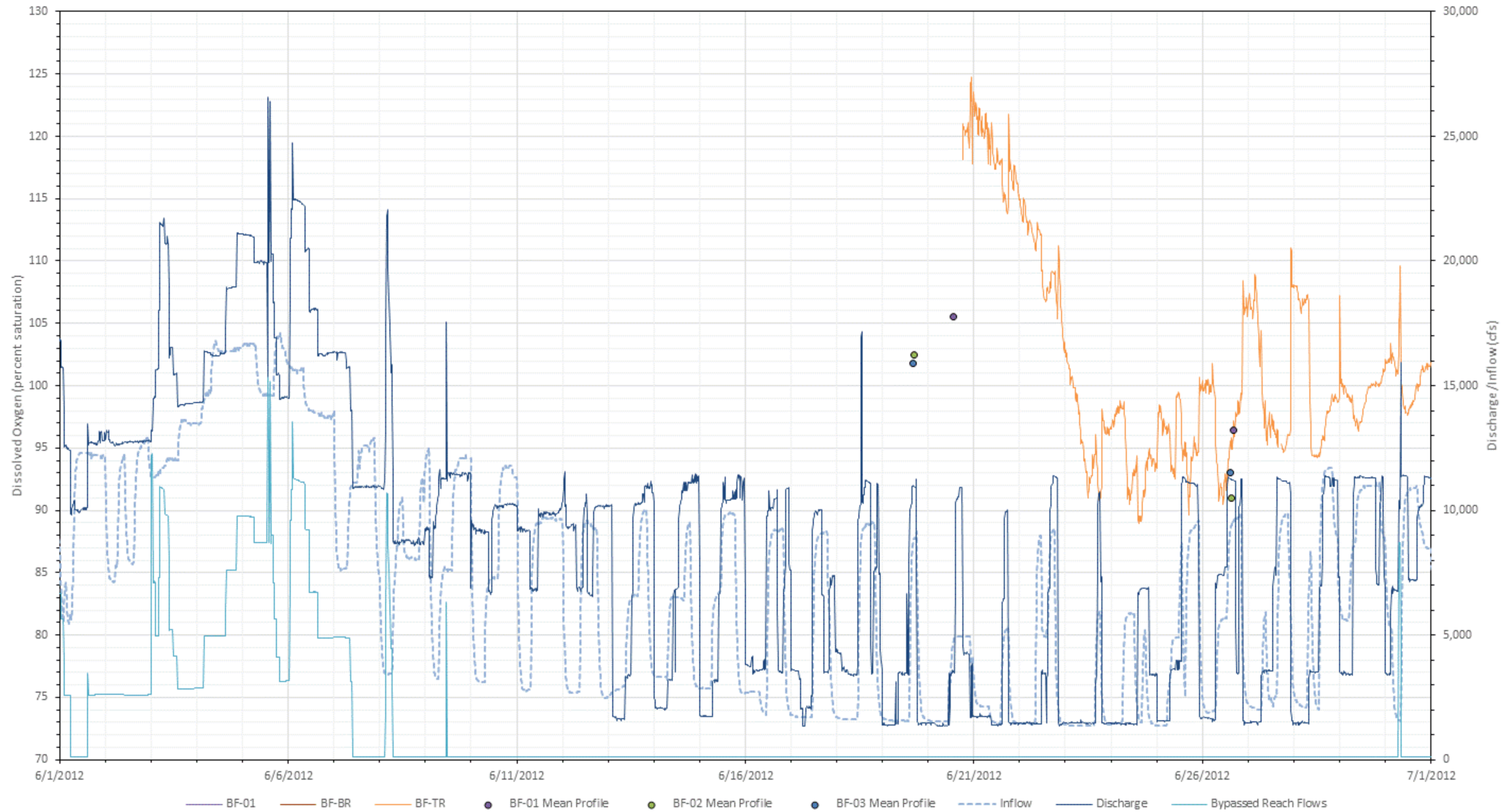
Figure L-29. 2012 June dissolved oxygen (percent saturation) at all Bellows Falls stations with inflow (USGS Gage No. 01144500), bypassed reach flow, and Bellows Falls project discharge.
