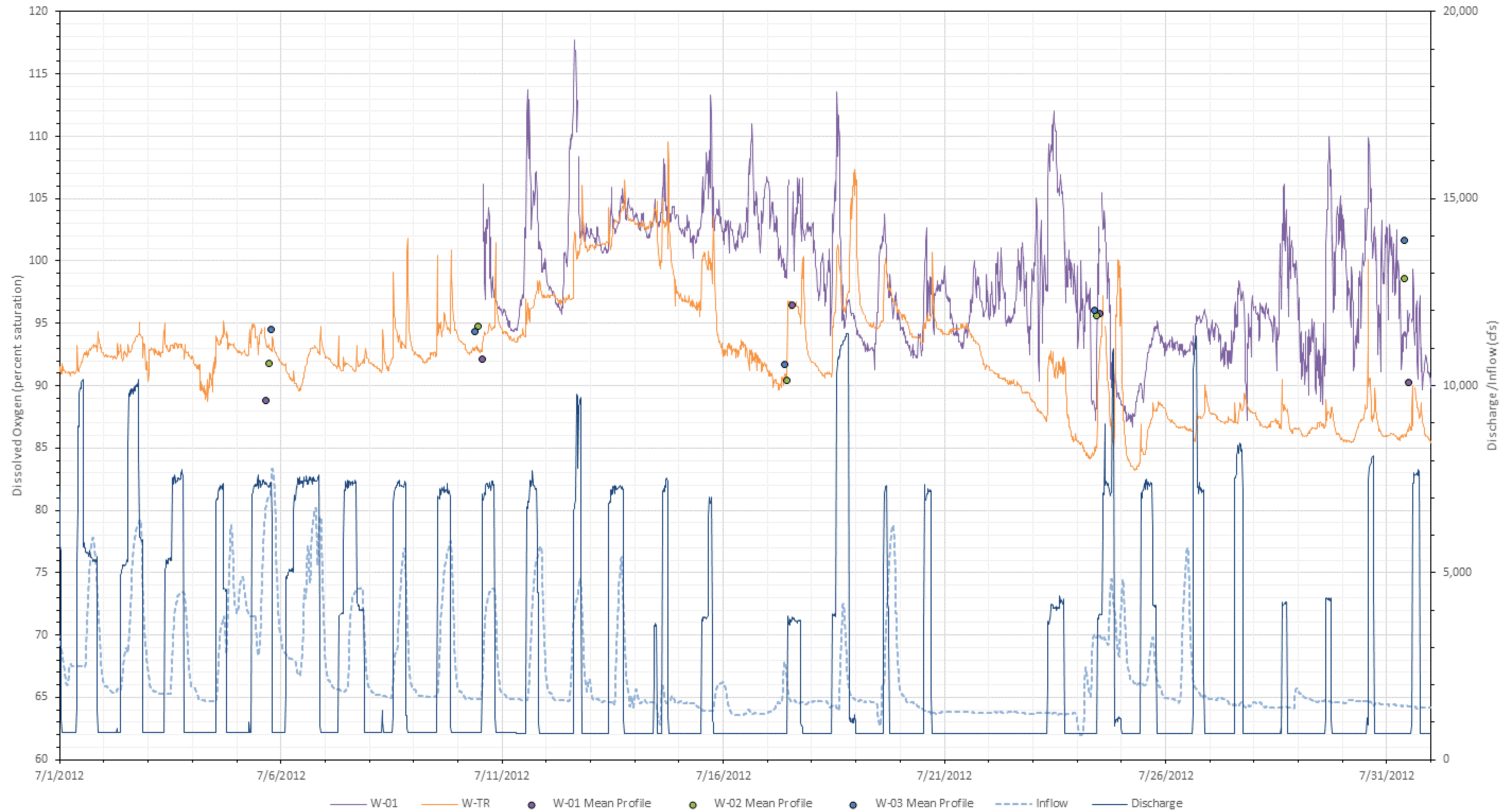
Figure L-26. 2012 July dissolved oxygen (percent saturation) at all Wilder mainstem stations with inflow (USGS Gage No. 01138500) and Wilder project discharge.
