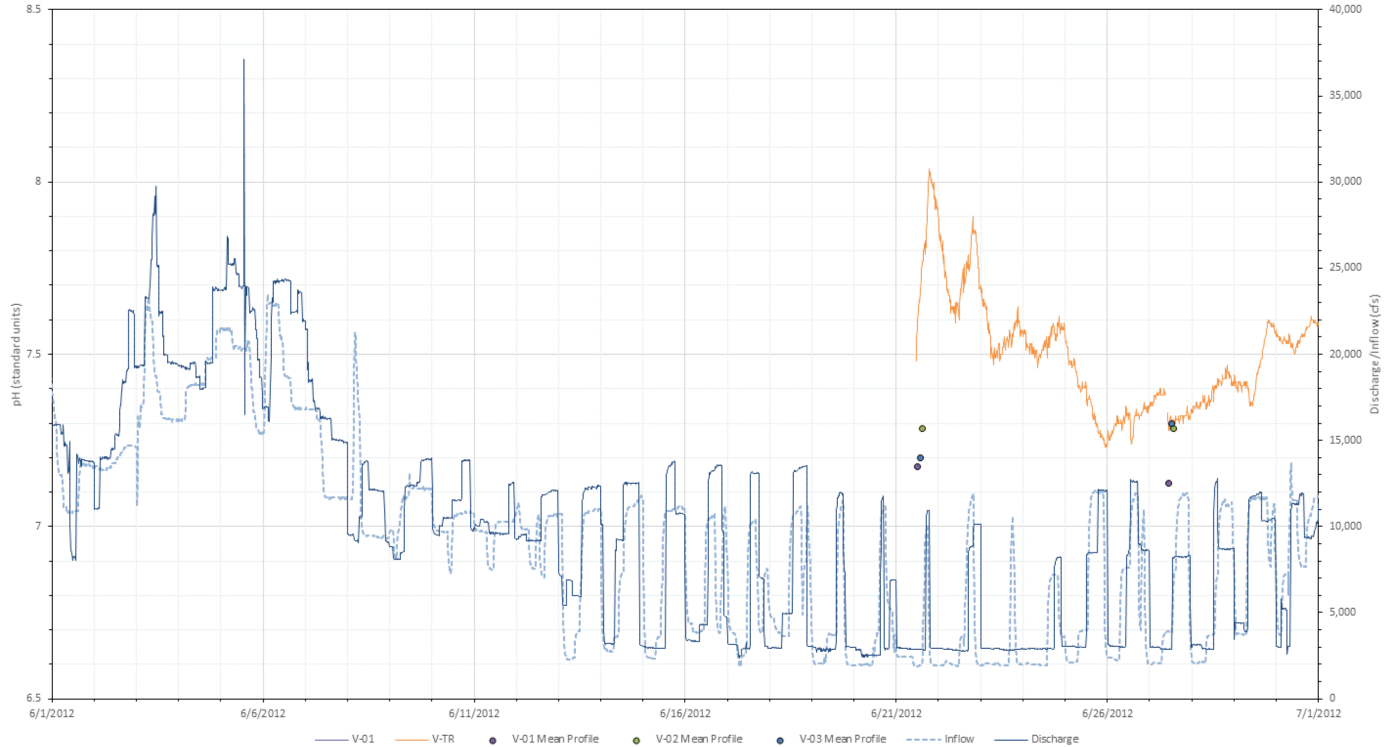
Figure L-45. 2012 June pH (standard units) at all mainstem Vernon stations with inflow (USGS Gage No. 01154500) and Vernon project discharge.
