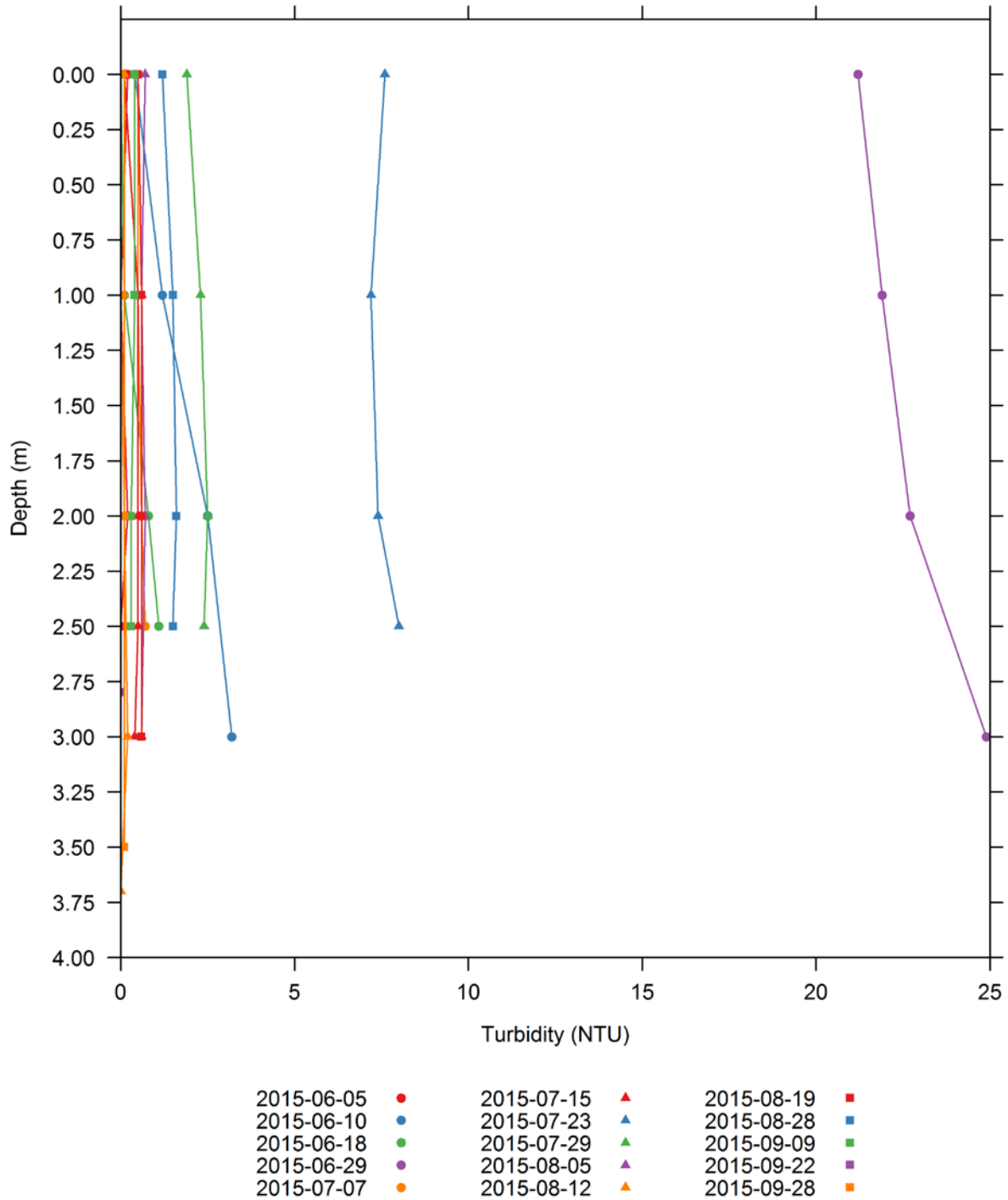
Figure H-48. Vertical profiles of NTU (NTU) collected at the Bellows Falls middle impoundment 06-BF-02 water quality monitoring station.
