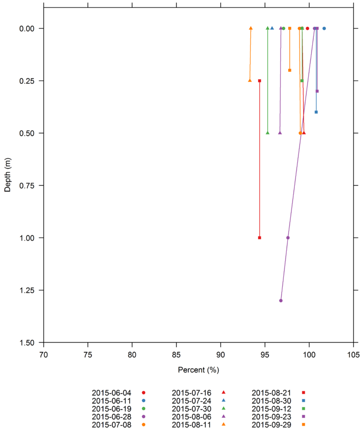
Figure H-3. Vertical profiles of dissolved oxygen (% saturation) collected at the Wilder upstream 06-W-04 water quality monitoring station.
