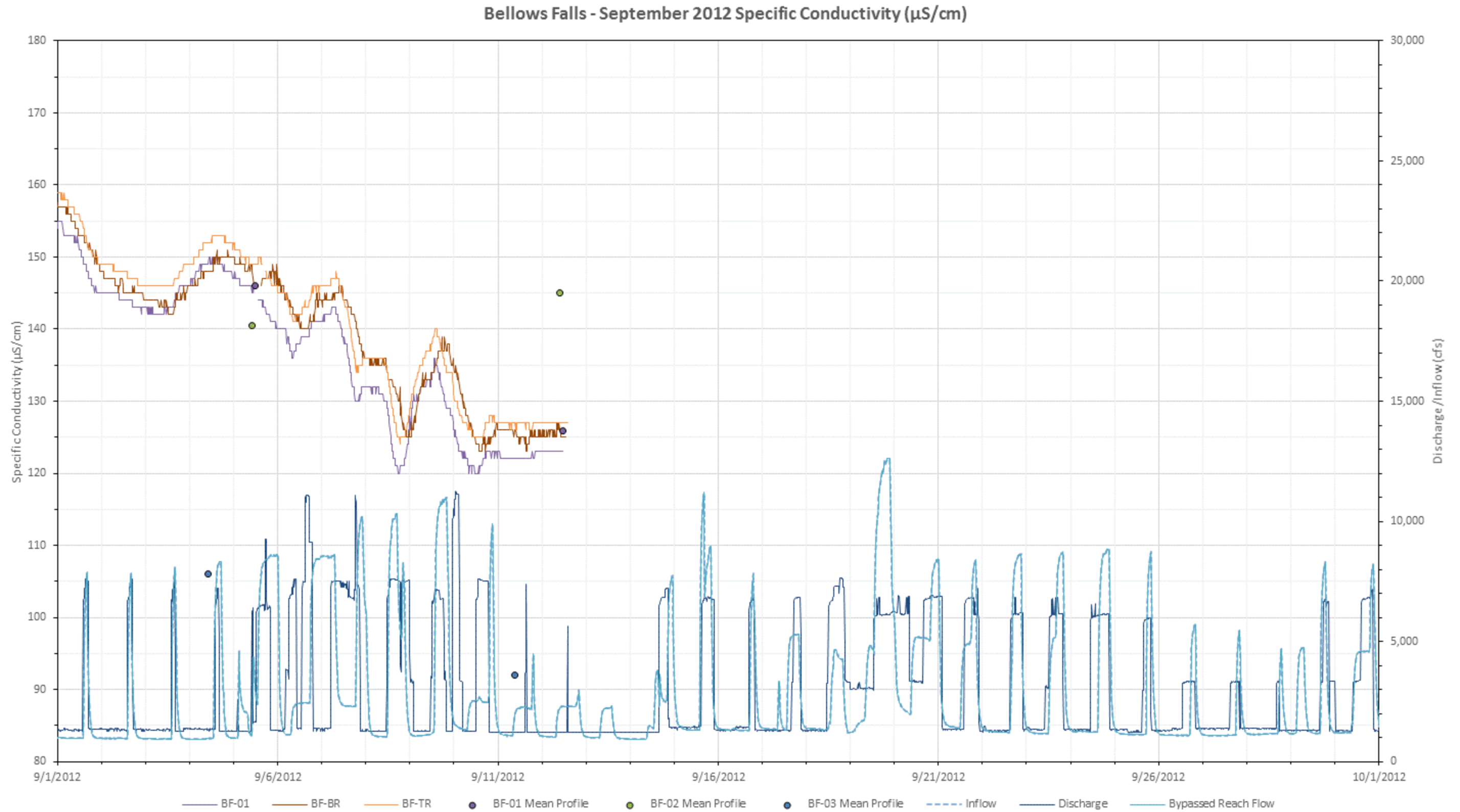
Figure L-56. 2012 September specific conductivity ( \mu\text{S}/\text{cm} ) at all Bellows Falls stations with inflow (USGS Gage No. 01144500), bypassed reach flow, and Bellows Falls project discharge.
