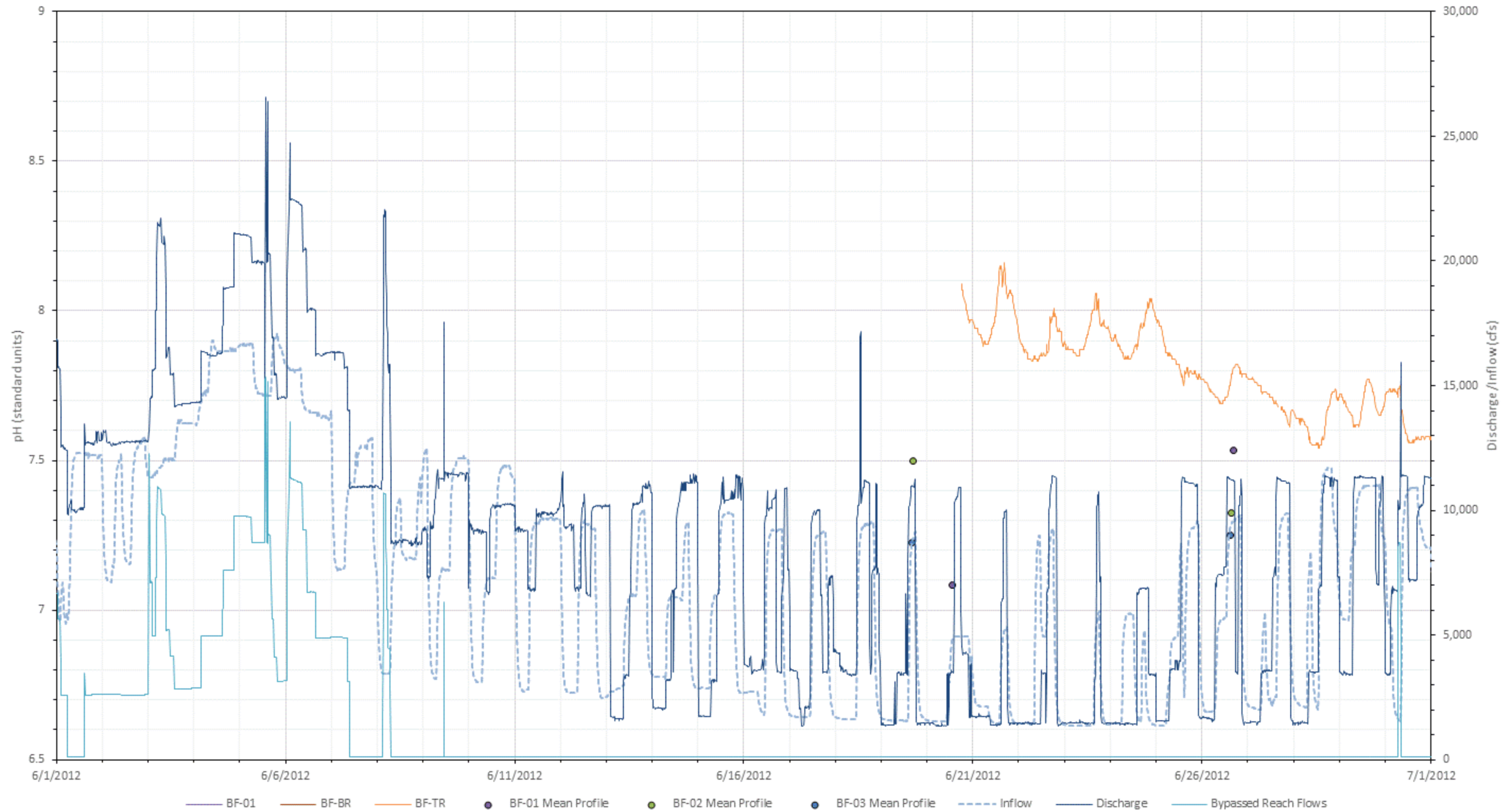
Figure L-41. 2012 June pH (standard units) at all Bellows Falls stations with inflow (USGS Gage No. 01144500), bypassed reach flow, and Bellows Falls project discharge.
