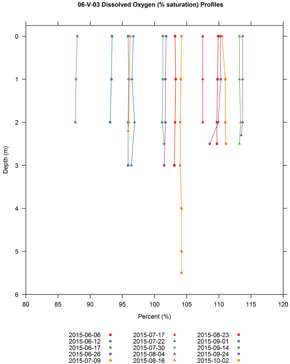
Figure H-69. Vertical profiles of dissolved oxygen (percent saturation) collected at the Vernon upper impoundment 06-V-03 water quality monitoring station.
