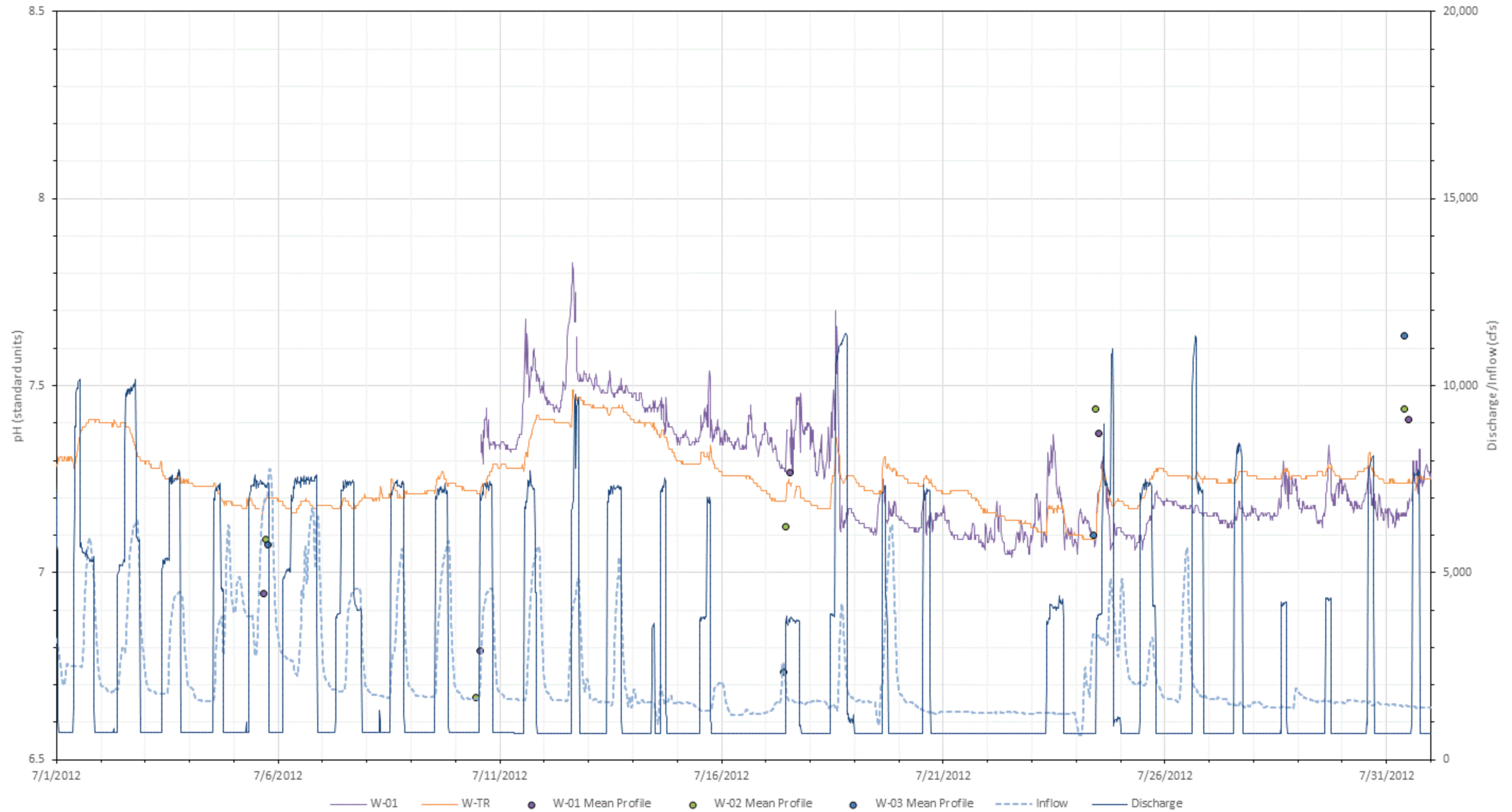
Figure L-38. 2012 July pH (standard units) at all Wilder mainstem stations with inflow (USGS Gage No. 01138500) and Wilder project discharge.
