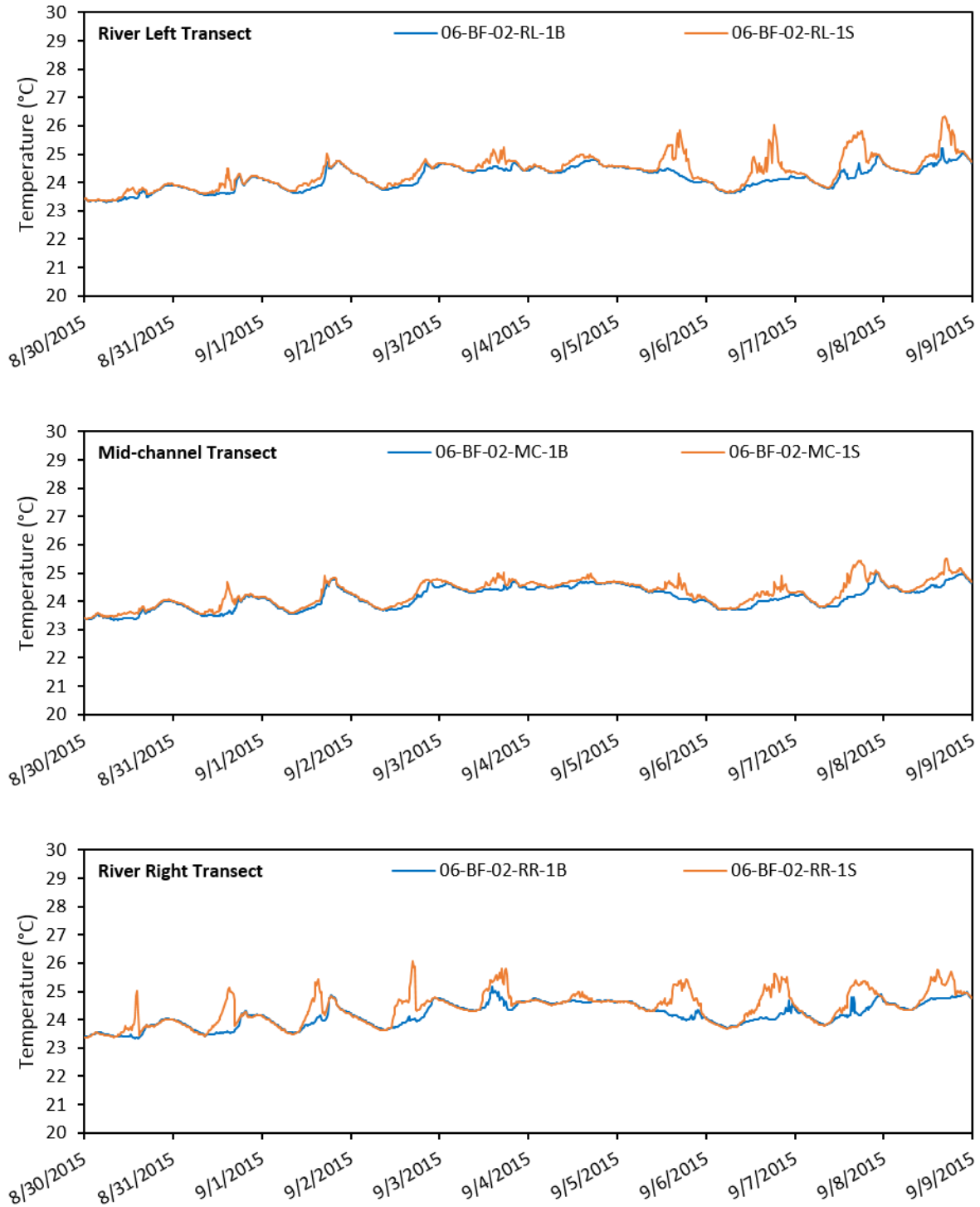
Figure I-7. Continuous water temperature collected at the Bellows Falls 06-BF-02 water quality monitoring station during the high temperature low-flow monitoring period. Loggers were deployed at one meter below the surface (1S) and one meter above the river bottom (1B).
