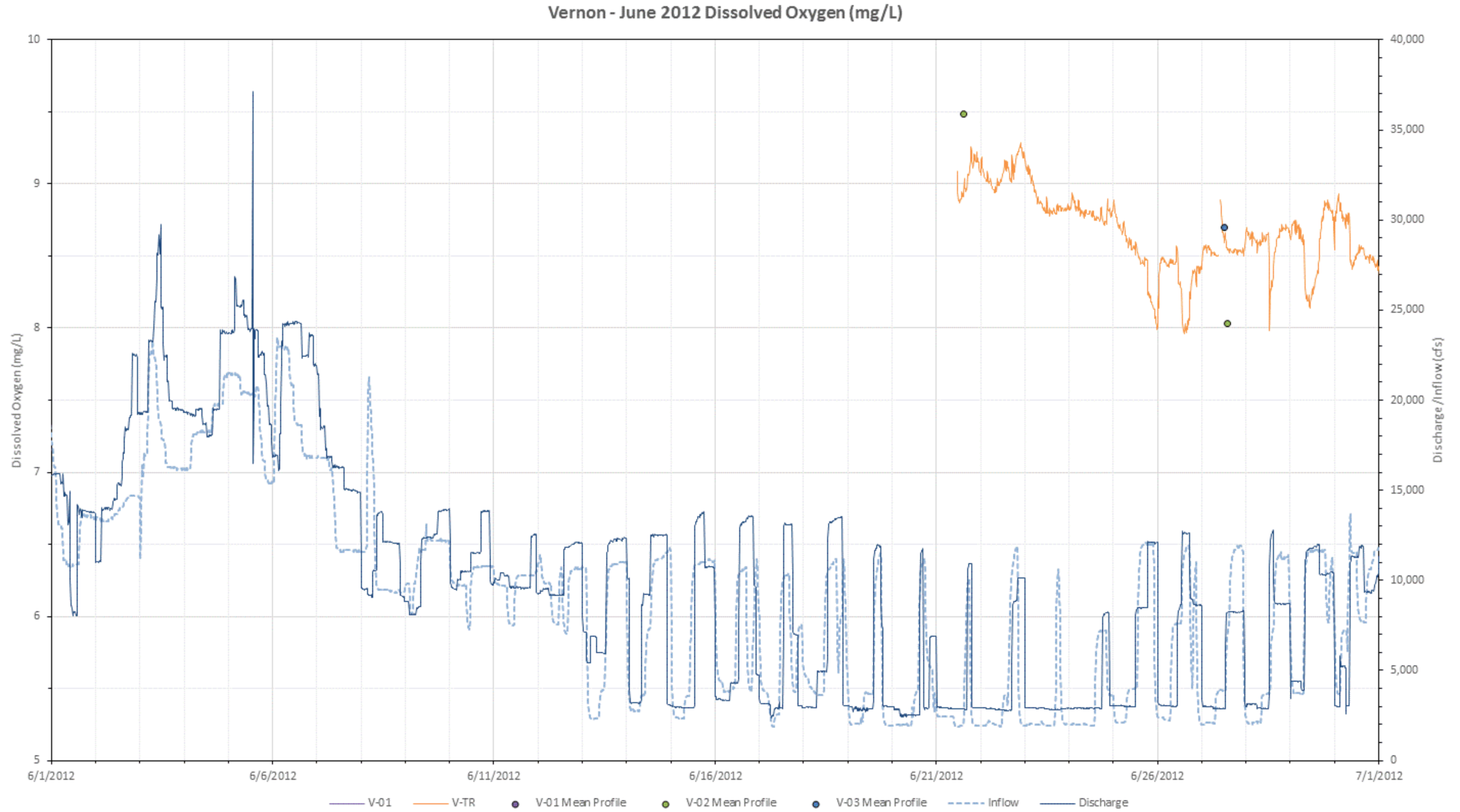
Figure L-21. 2012 June dissolved oxygen (mg/L) at all mainstem Vernon stations with inflow (USGS Gage No. 01154500) and Vernon project discharge.
