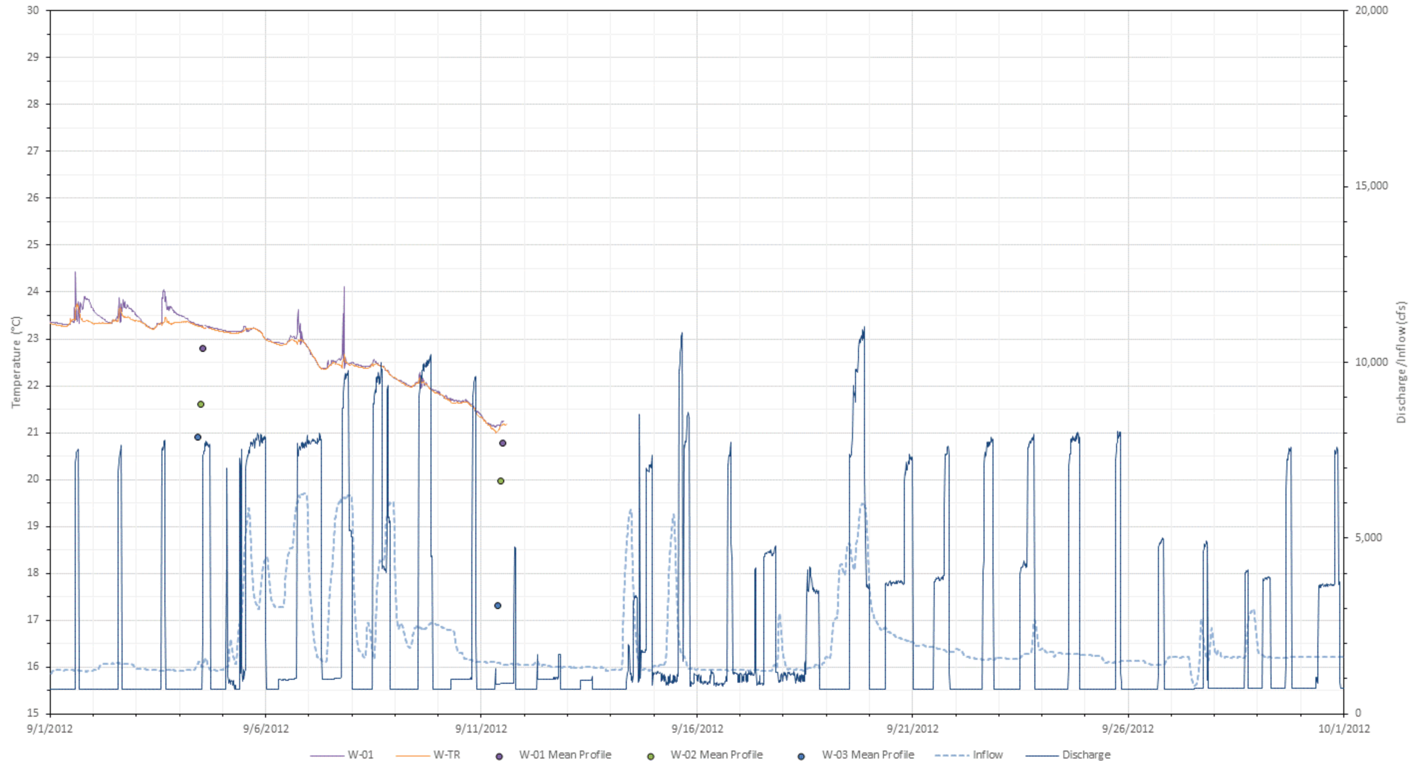
Figure L-4. 2012 September water temperatures at all Wilder stations with inflow (USGS Gage No. 01138500) and Wilder project discharge.
