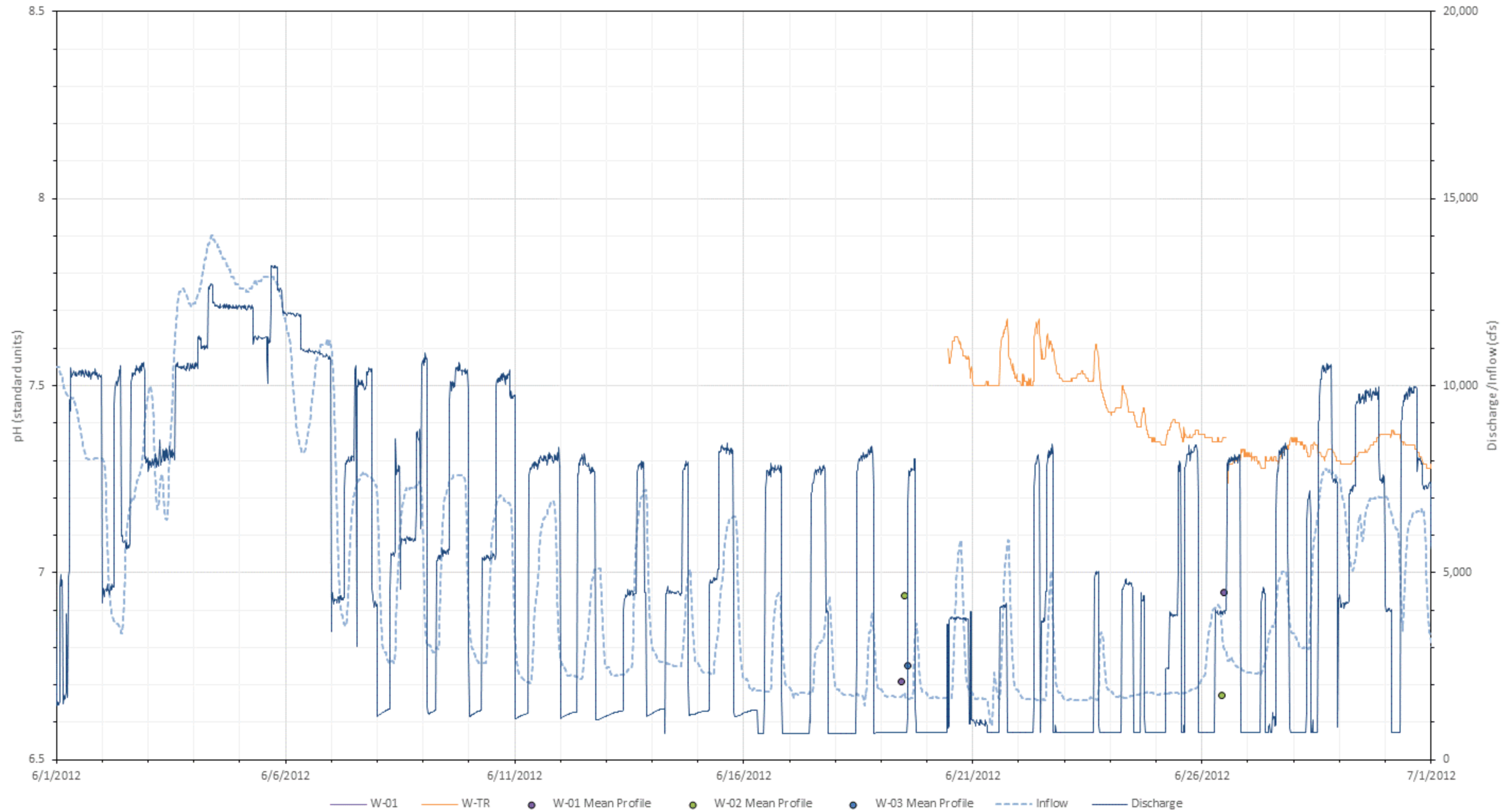
Figure L-37. 2012 June pH (standard units) at all Wilder mainstem stations with inflow (USGS Gage No. 01138500) and Wilder project discharge.
