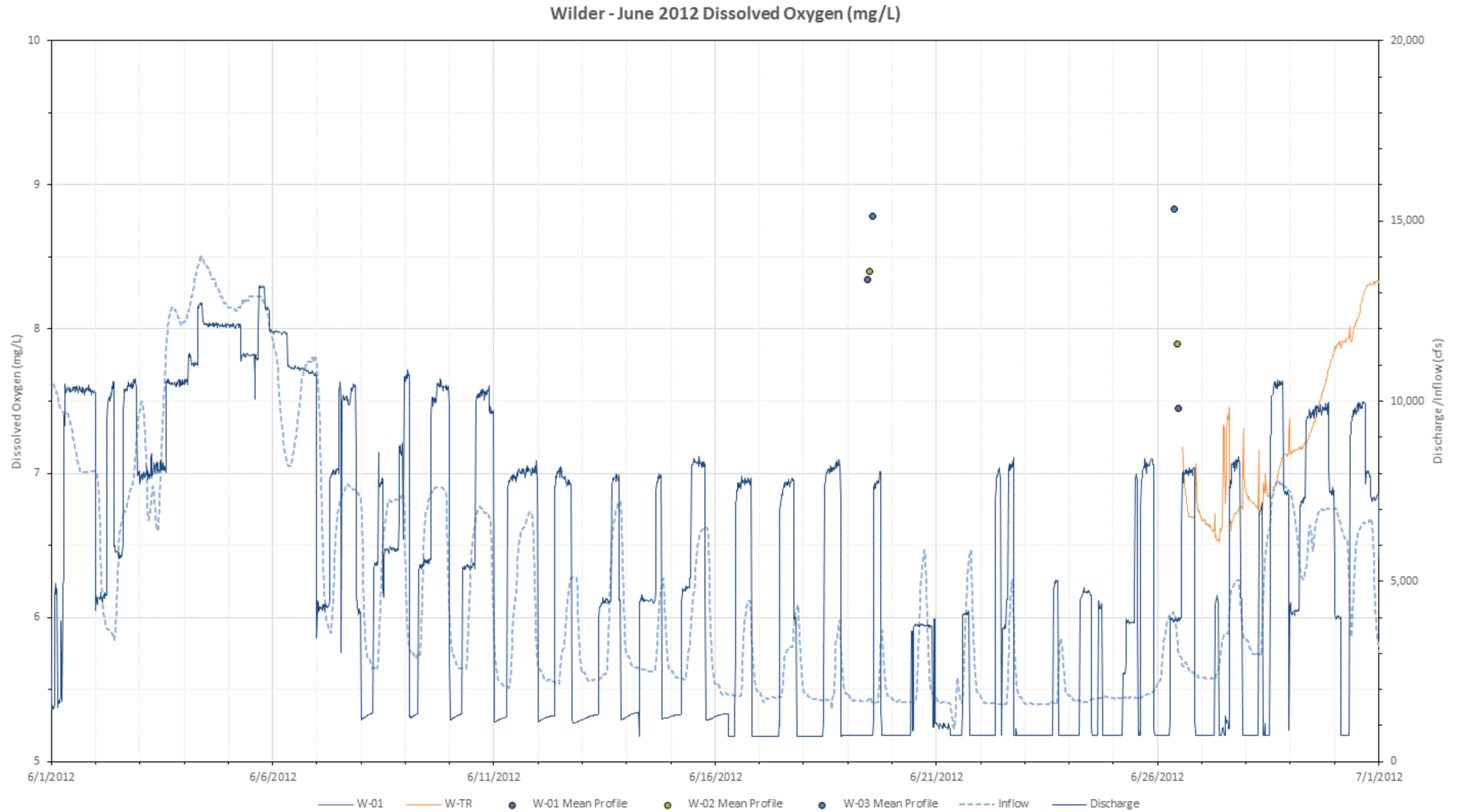
Figure L-13. 2012 June dissolved oxygen (mg/L) at all Wilder mainstem stations with inflow (USGS Gage No. 01138500) and Wilder project discharge.
