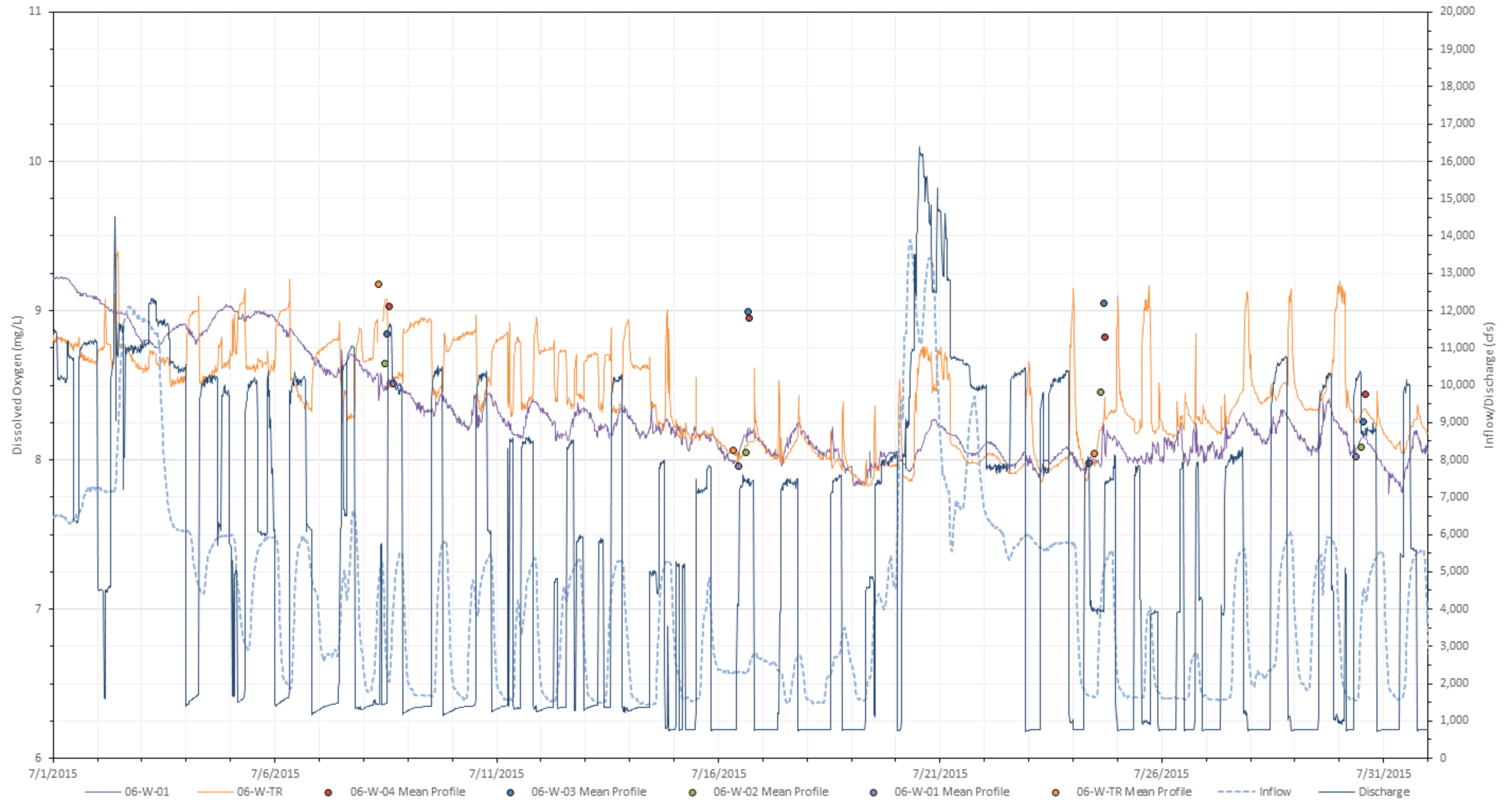
Figure F-25. 2015 July dissolved oxygen (mg/L) at all Wilder mainstem stations with inflow (USGS Gage No. 01138500) and Wilder project discharge.
