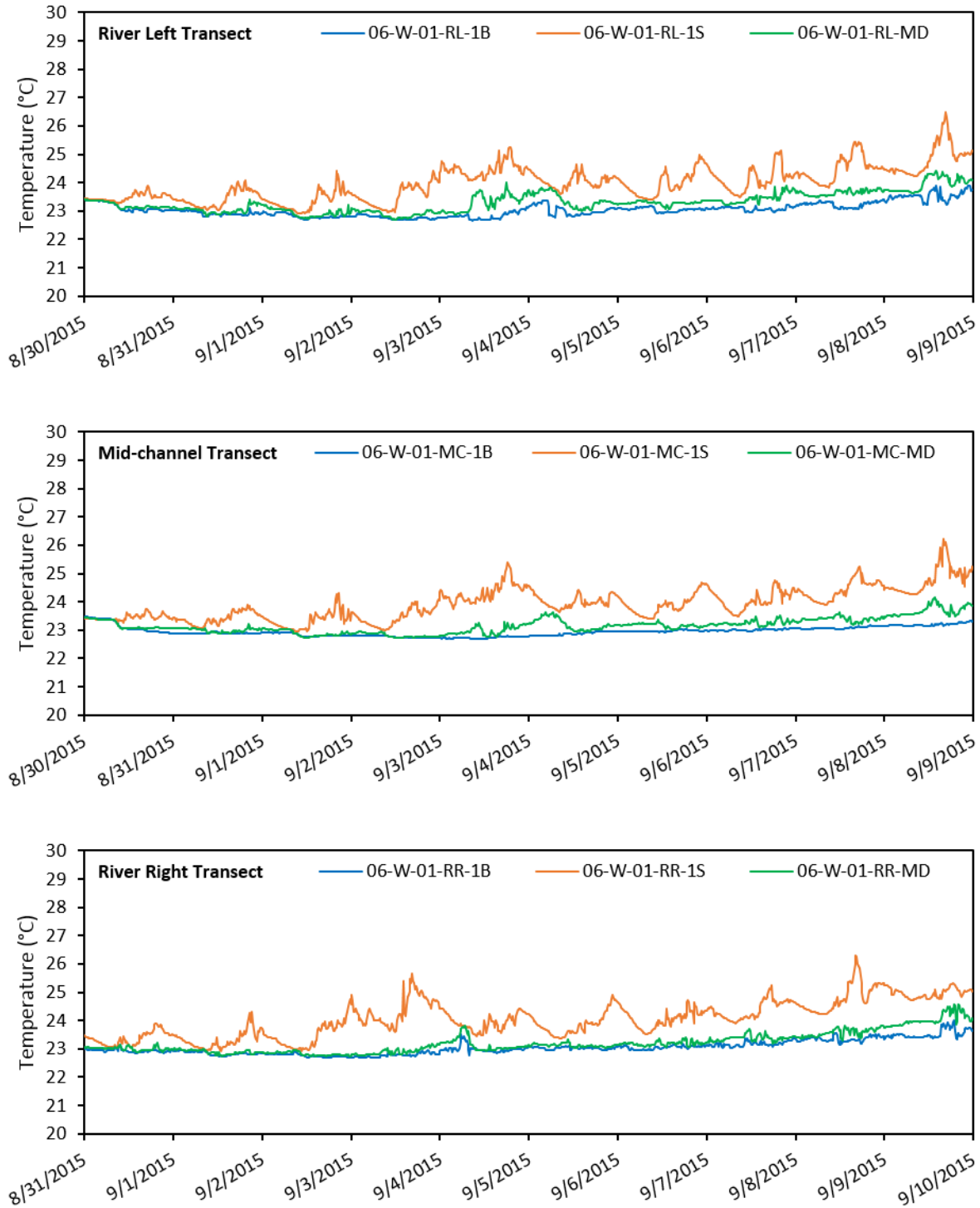
Figure I-4. Continuous water temperature collected at the Wilder forebay 06-W-01 water quality monitoring station during the high temperature low-flow monitoring period. Loggers were deployed at one meter below the surface (1S), mid-depth (MD), and one meter above the river bottom (1B).
