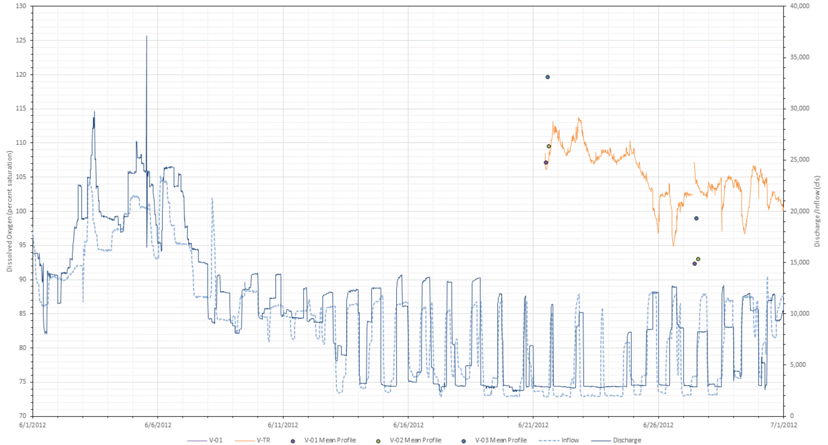
Figure L-33. 2012 June dissolved oxygen (percent saturation) at all mainstem Vernon stations with inflow (USGS Gage No. 01154500) and Vernon project discharge.
