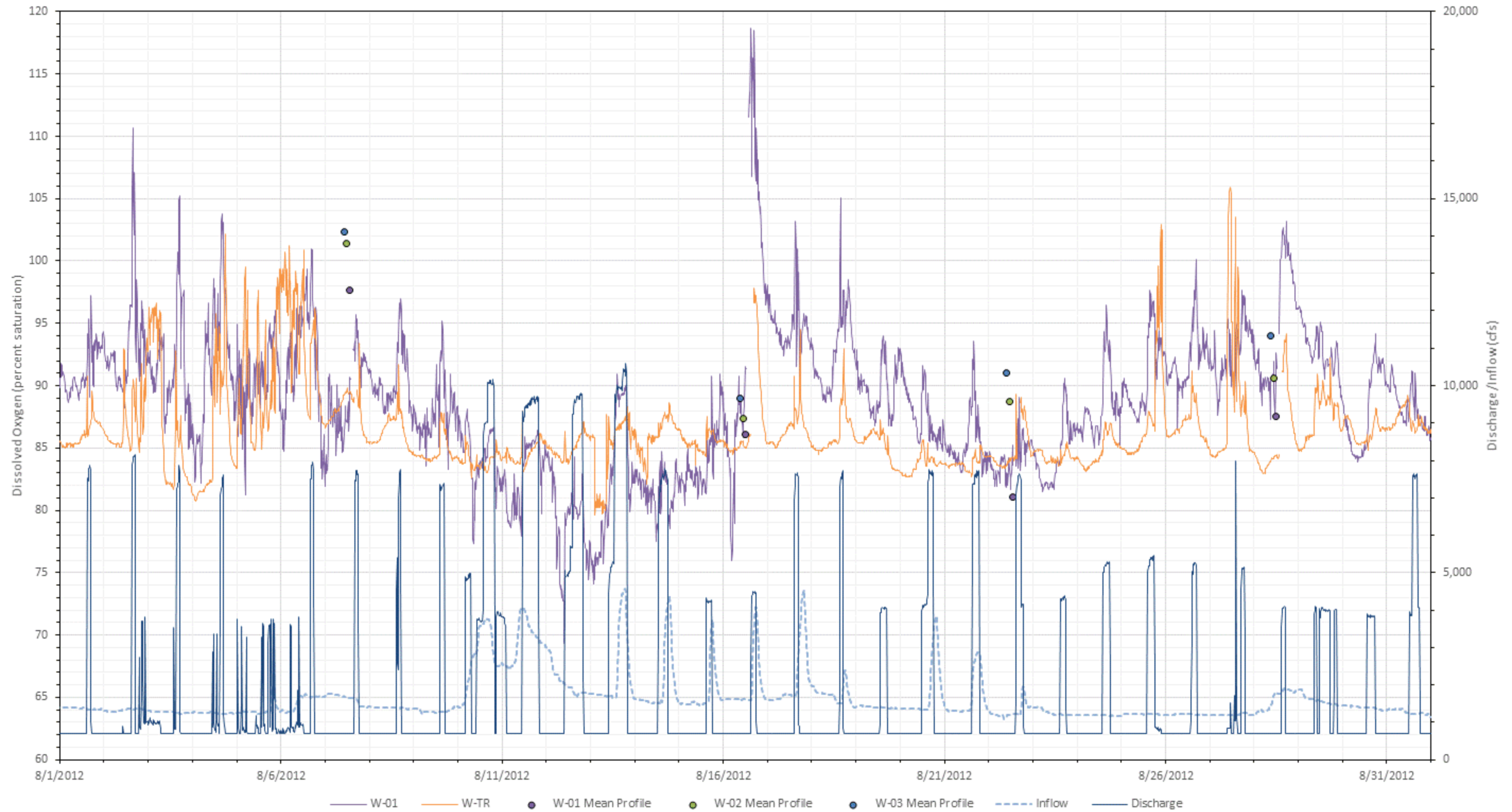
Figure L-27. 2012 August dissolved oxygen (percent saturation) at all Wilder mainstem stations with inflow (USGS Gage No. 01138500) and Wilder project discharge.
