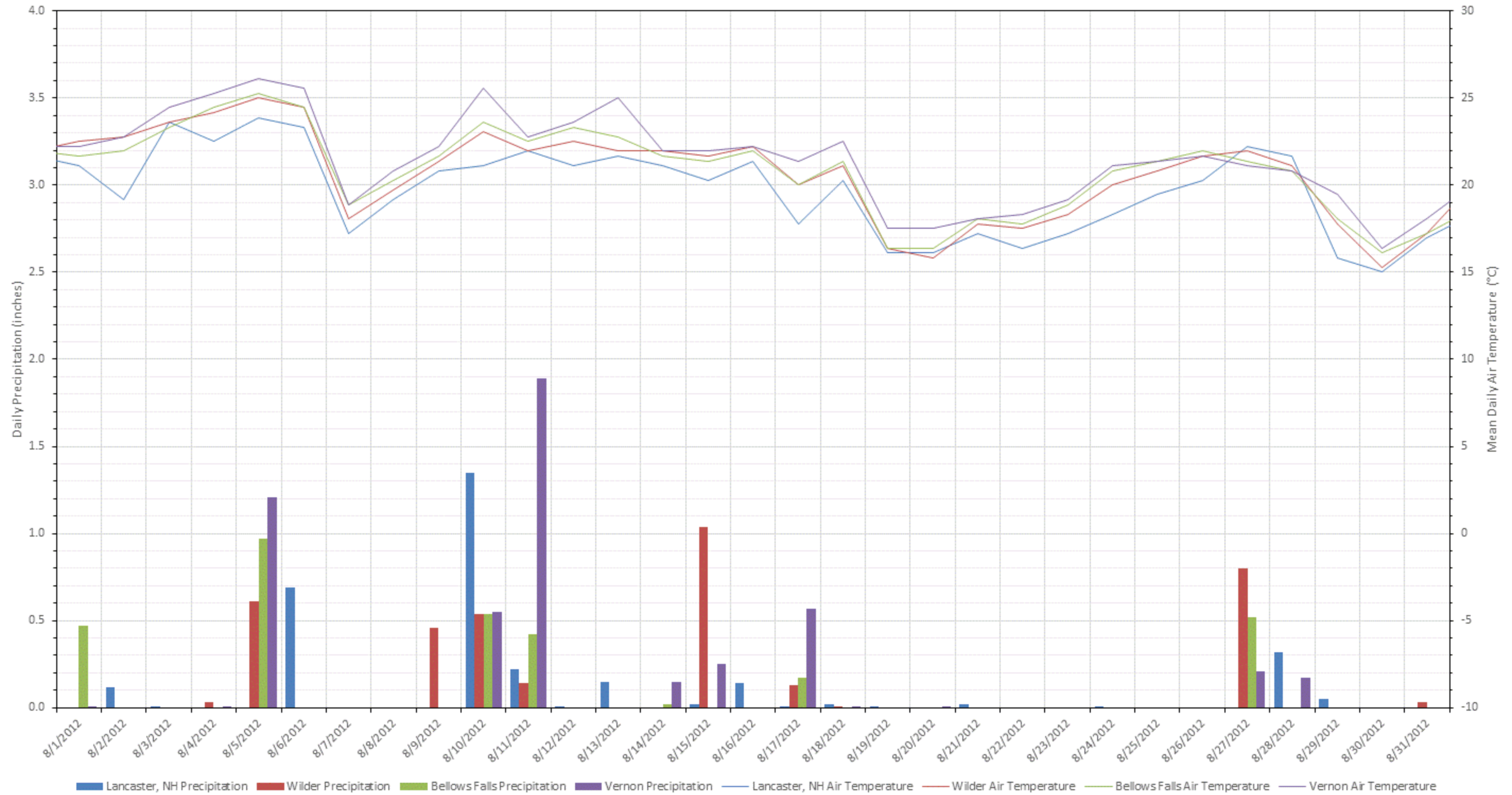
Figure M-3. 2012 August daily mean air temperature (°C) and daily precipitation (inches) for the study area.
