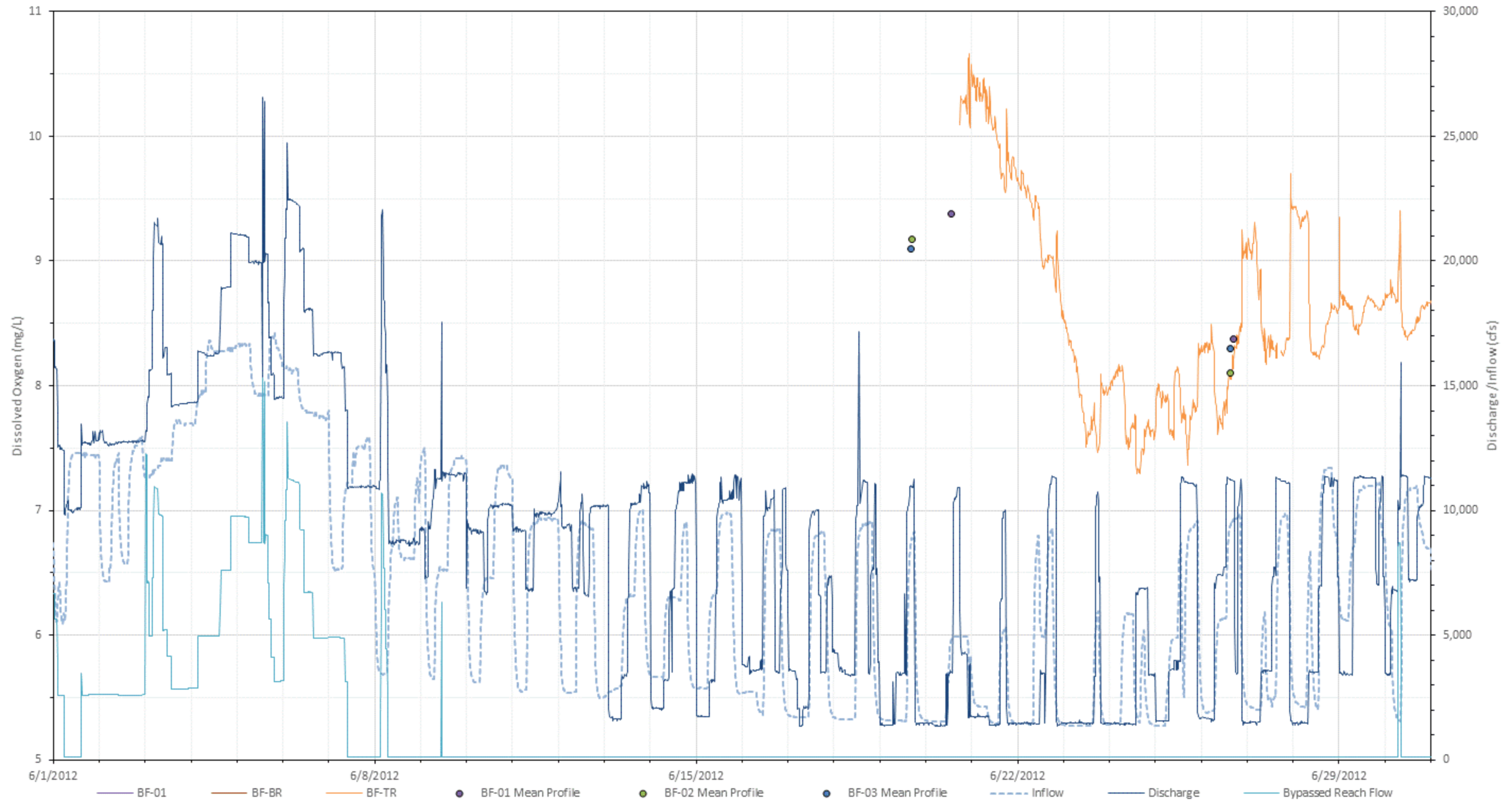
Figure L-17. 2012 June dissolved oxygen (mg/L) at all Bellows Falls stations with inflow (USGS Gage No. 01144500), bypassed reach flow, and Bellows Falls project discharge.
