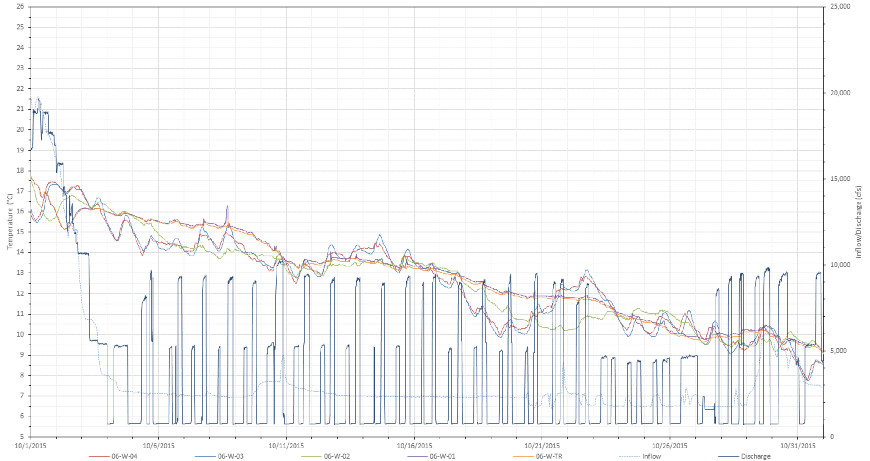
Figure F-6. 2015 October water temperatures at all Wilder stations with inflow (USGS Gage No. 01138500) and Wilder project discharge.
