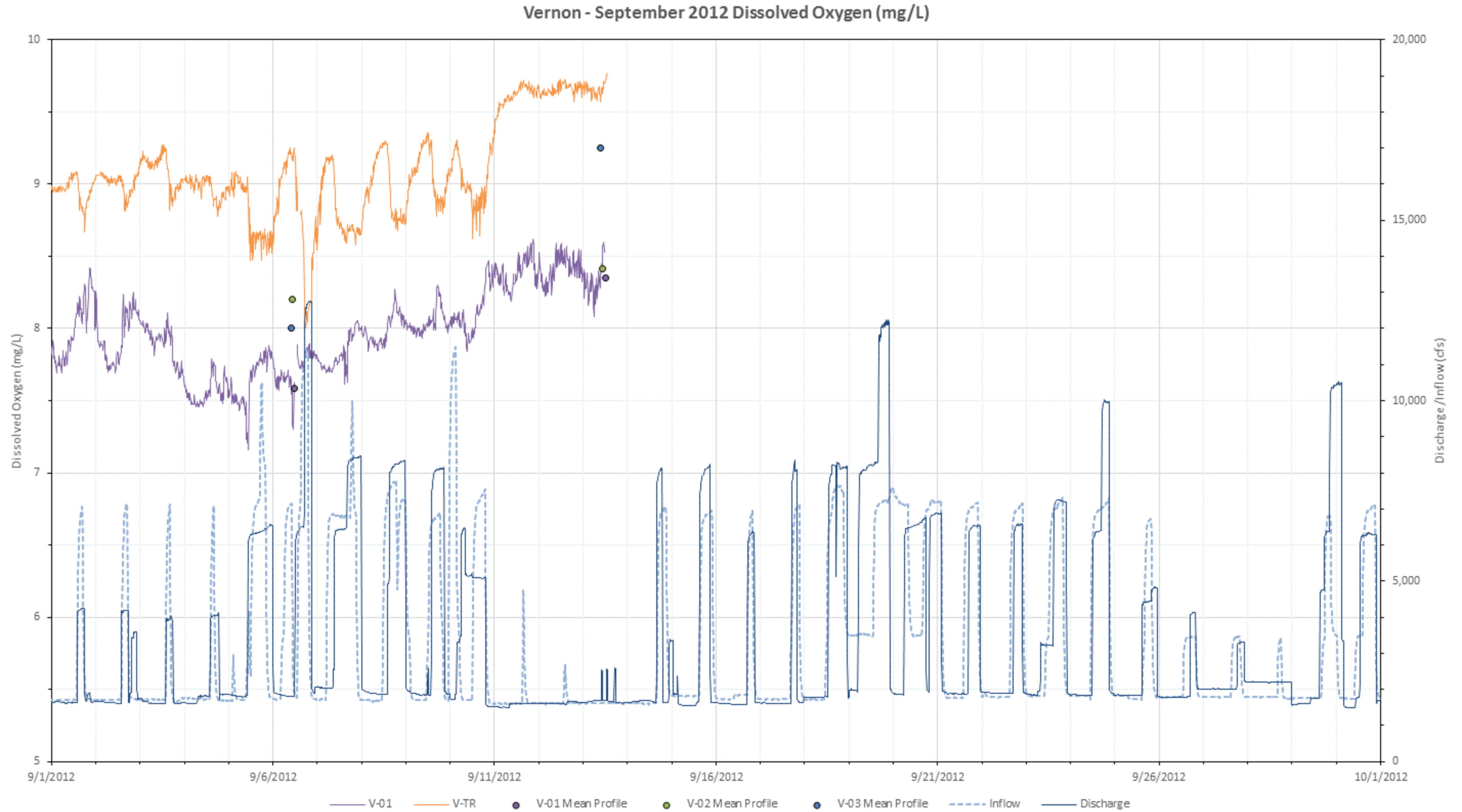
Figure L-24. 2012 September dissolved oxygen (mg/L) at all mainstem Vernon stations with inflow (USGS Gage No. 01154500) and Vernon project discharge.
