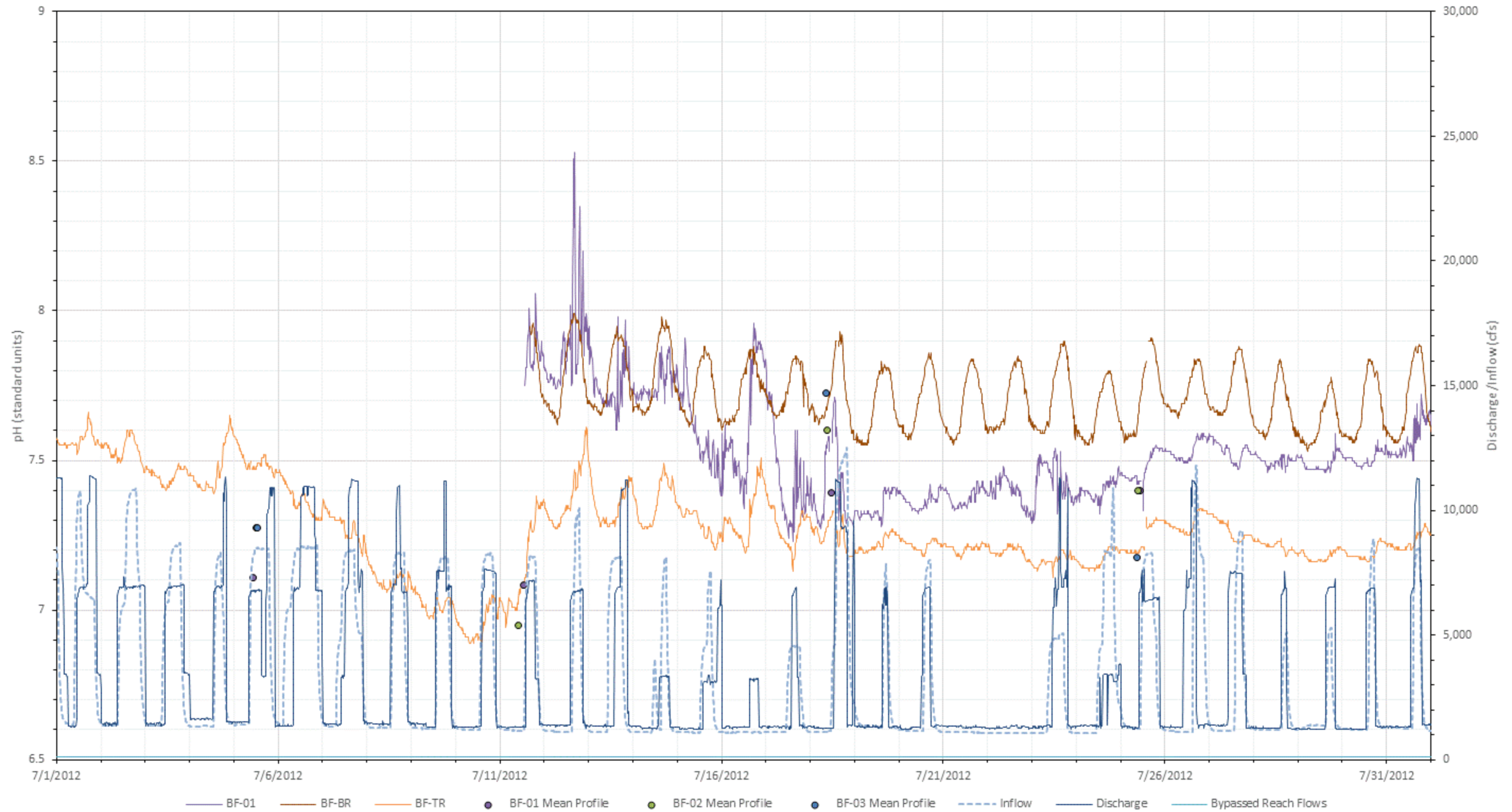
Bellows Falls - July 2012 pH (standard units)
