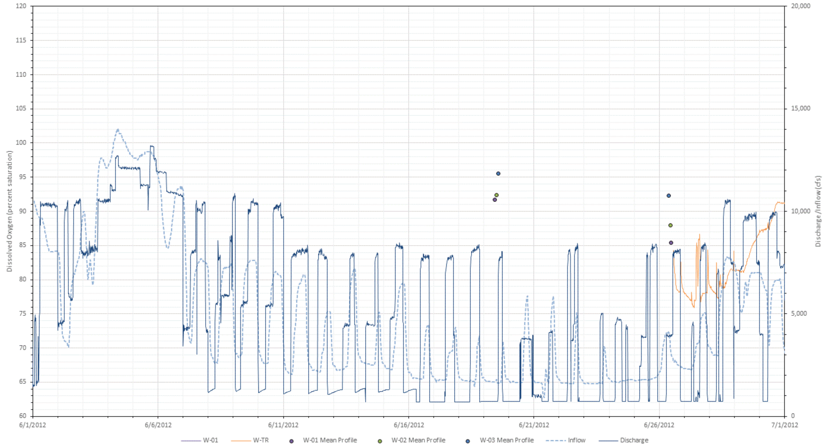
Figure L-25. 2012 June dissolved oxygen (percent saturation) at all Wilder mainstem stations with inflow (USGS Gage No. 01138500) and Wilder project discharge.
