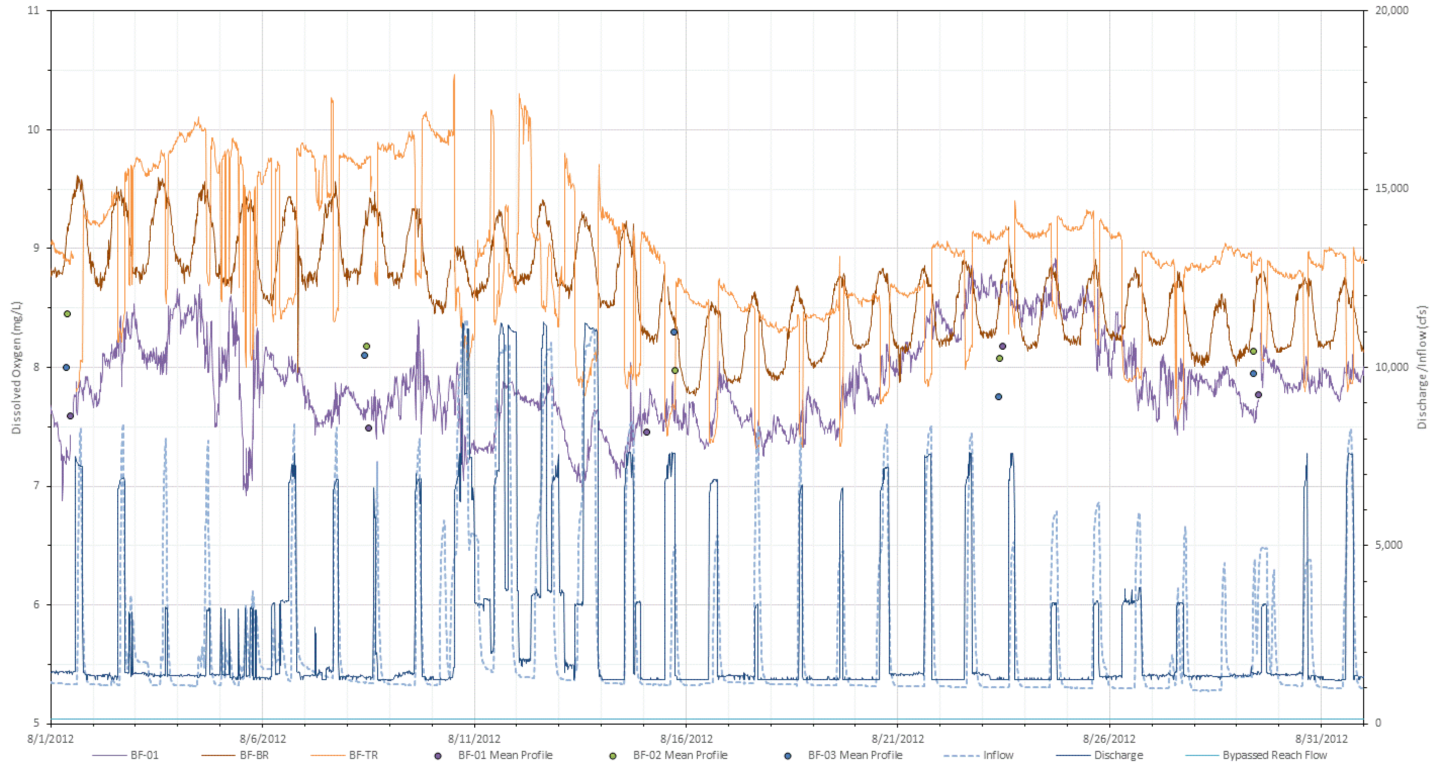
Figure L-19. 2012 August dissolved oxygen (mg/L) at all Bellows Falls stations with inflow (USGS Gage No. 01144500), bypassed reach flow, and Bellows Falls project discharge.
