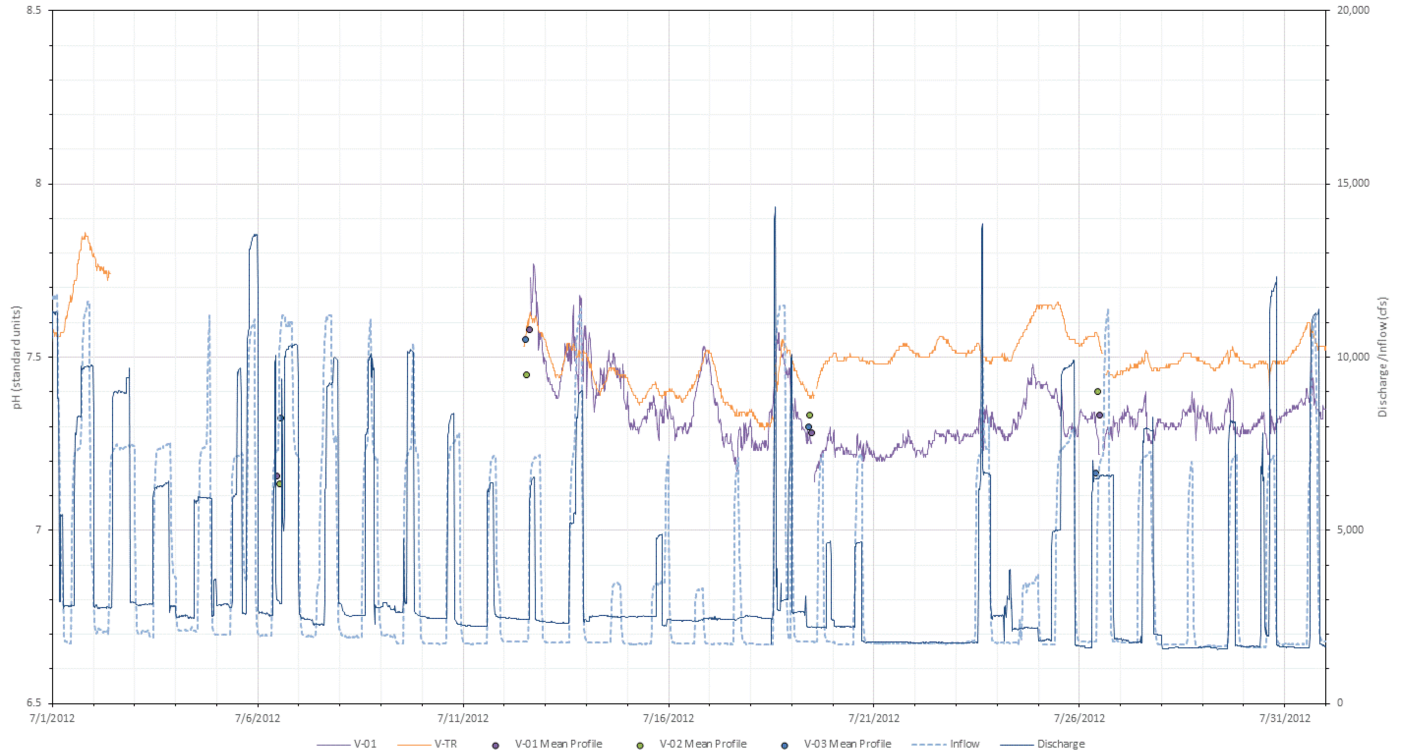
Figure L-46. 2012 July pH (standard units) at all mainstem Vernon stations with inflow (USGS Gage No. 01154500) and Vernon project discharge.
