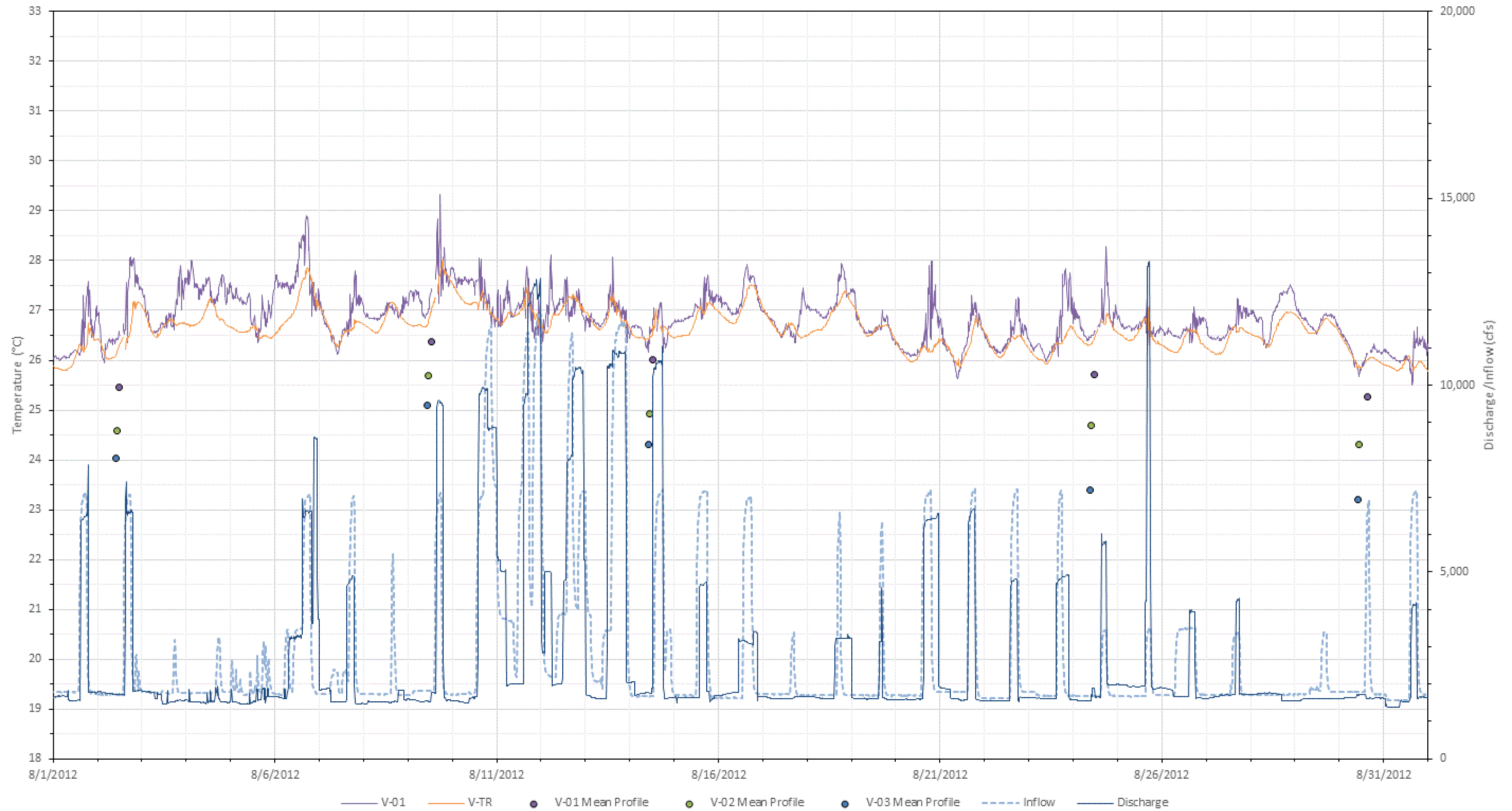
Figure L-11. 2012 August water temperatures at all mainstem Vernon stations with inflow (USGS Gage No. 01154500) and Vernon project discharge.
