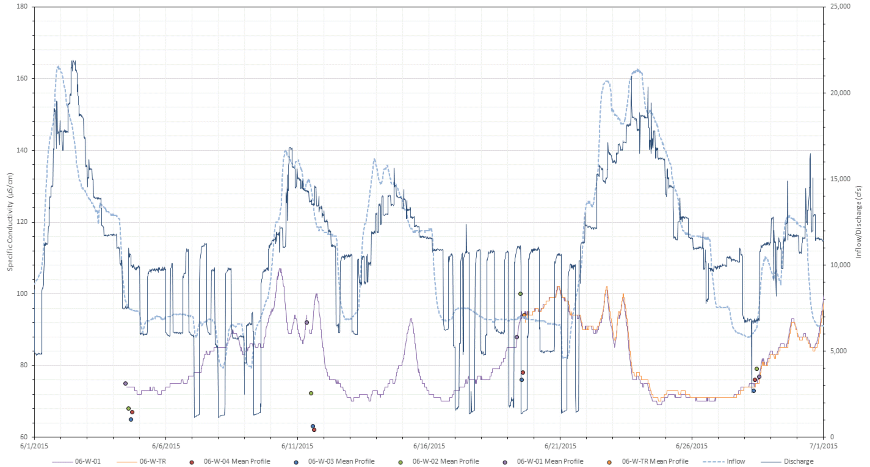
Wilder - June 2015 Specific Conductivity ( \mu\text{S}/\text{cm} )
