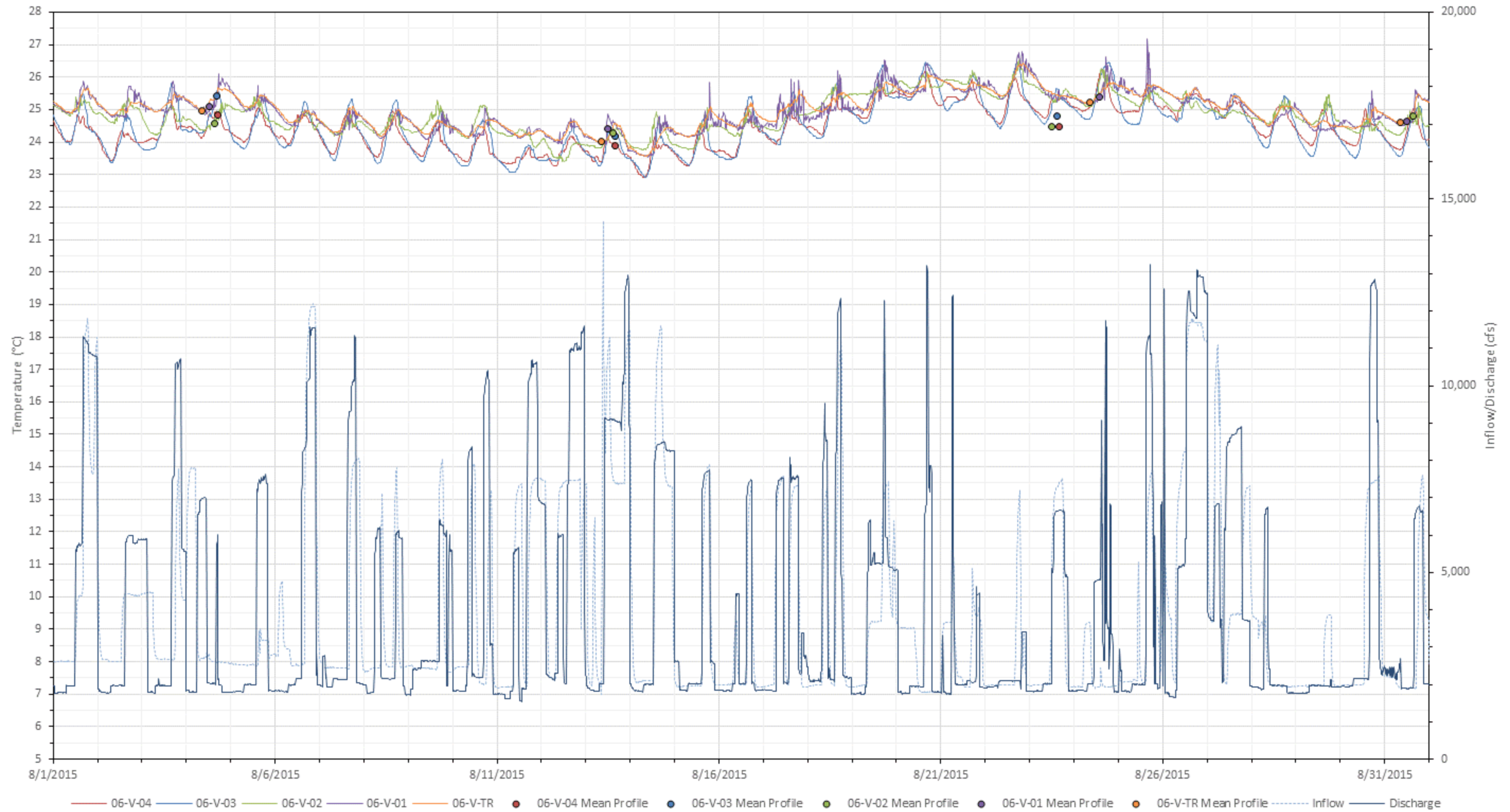
Figure F-20. 2015 August water temperatures at all mainstem Vernon stations with inflow (USGS Gage No. 01154500) and Vernon project discharge.
