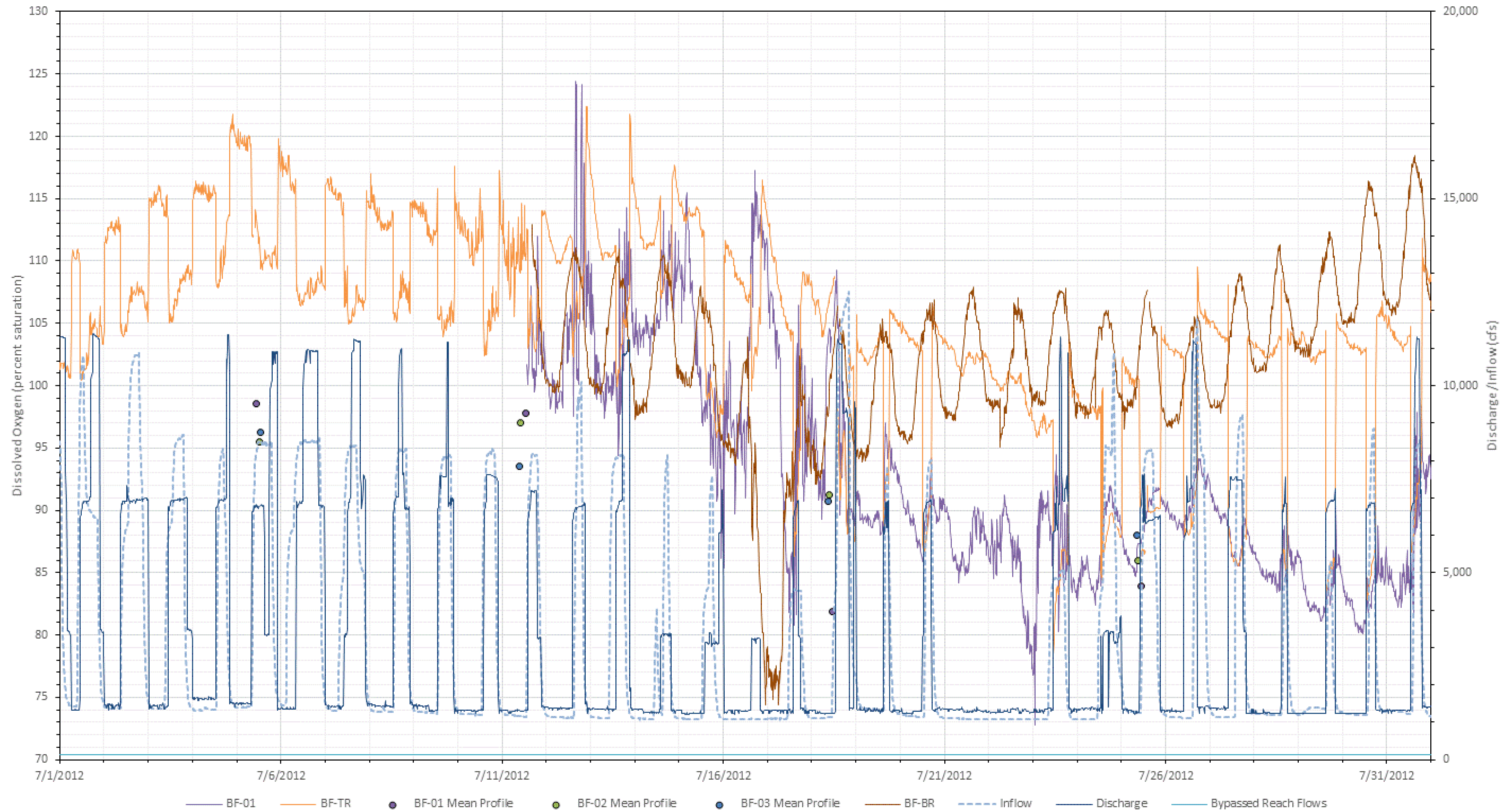
Figure L-30. 2012 July dissolved oxygen (percent saturation) at all Bellows Falls stations with inflow (USGS Gage No. 01144500), bypassed reach flow, and Bellows Falls project discharge.
