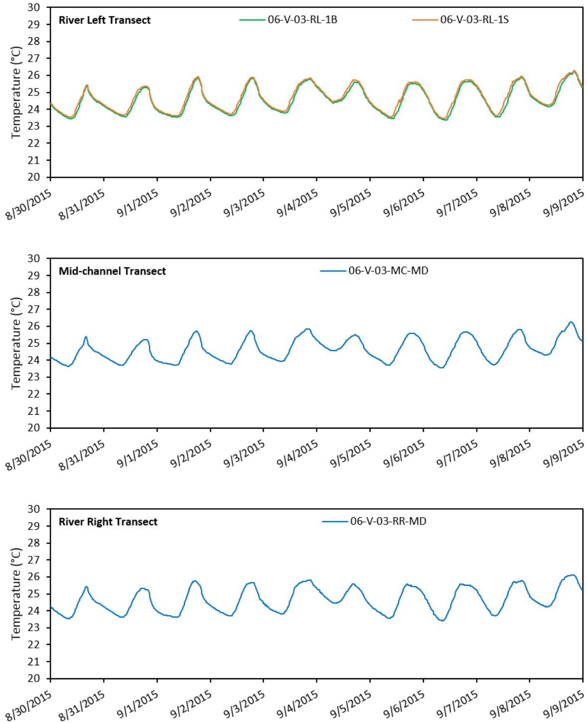
Figure I-10. Continuous water temperature collected at the Vernon 06-V-03 water quality monitoring station during the high temperature low flow monitoring period. Loggers were deployed at one meter below the surface (1S), mid-depth (MD), and one meter above the river bottom (1B).
