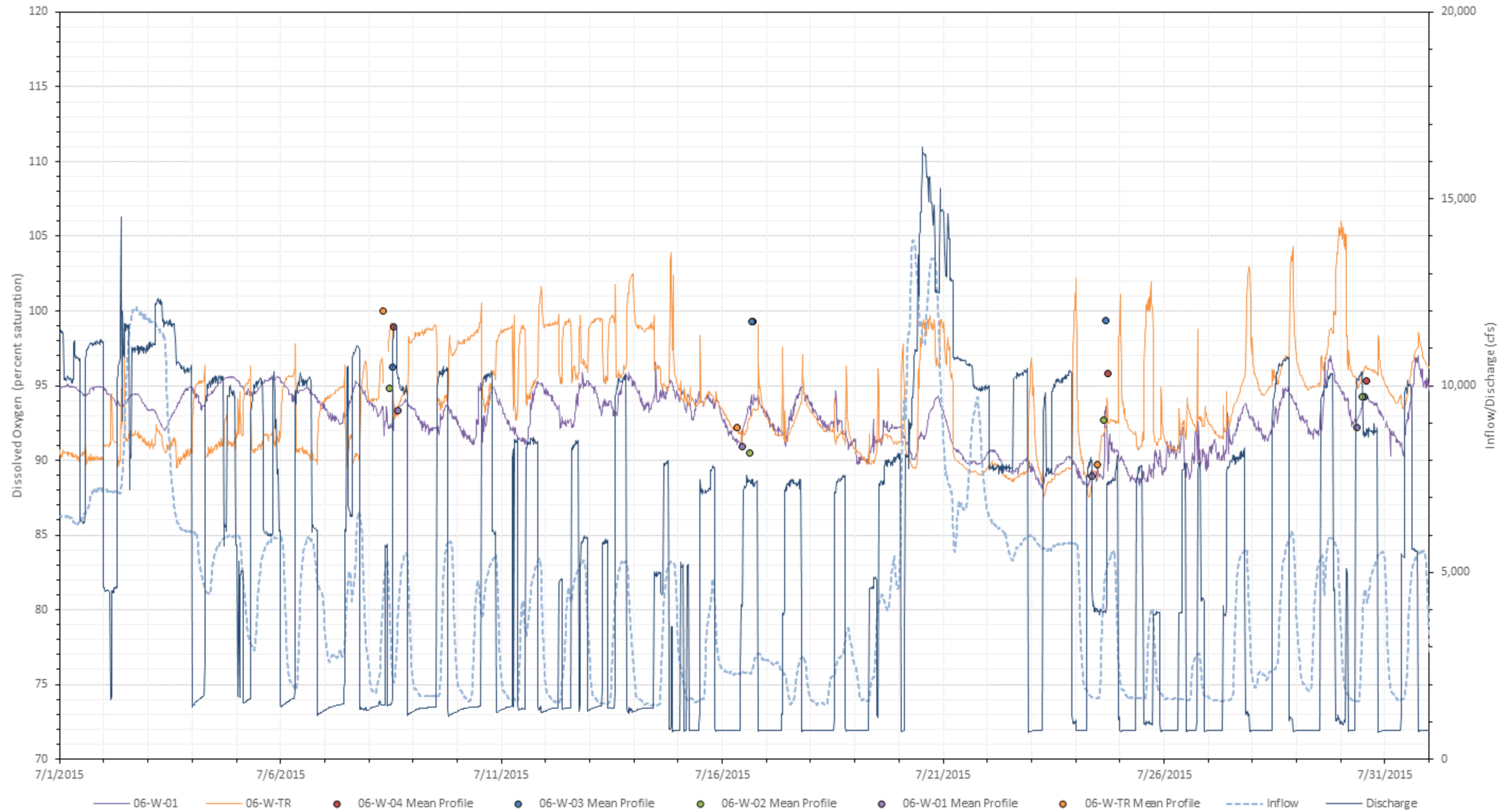
Figure F-37. 2015 July dissolved oxygen (percent saturation) at all Wilder mainstem stations with inflow (USGS Gage No. 01138500) and Wilder project discharge.
