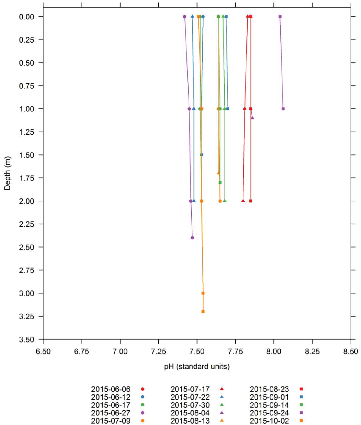
Figure H-65. Vertical profiles of pH (standard units) collected at the Vernon upstream 06-V-04 water quality monitoring station.
