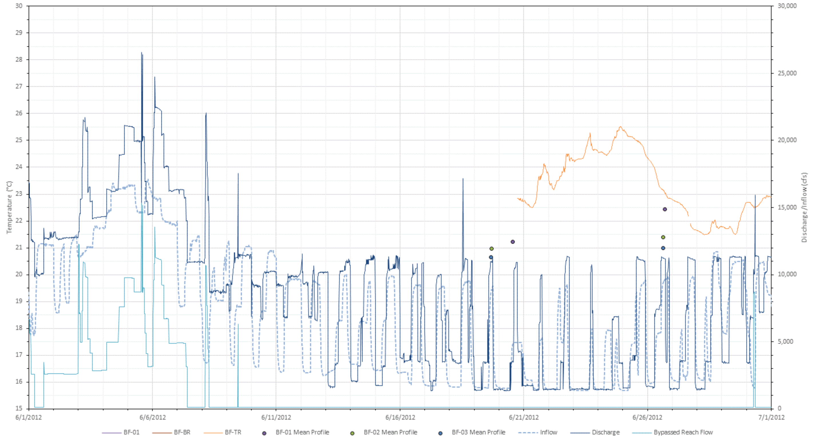
Figure L-5. 2012 June water temperatures at all Bellows Falls stations with inflow (USGS Gage No. 01144500), bypassed reach flow, and Bellows Falls project discharge.
