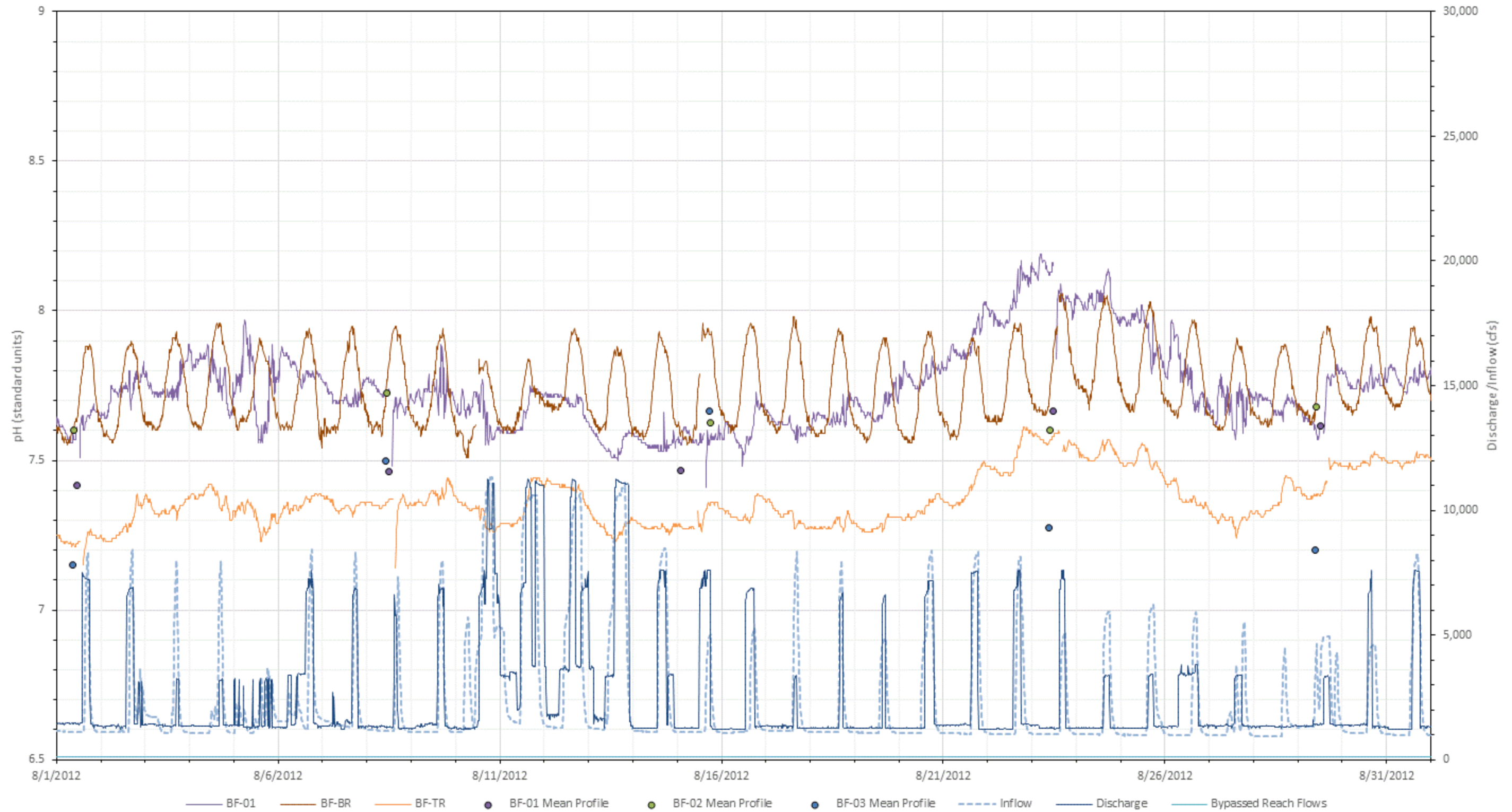
Figure L-43. 2012 August pH (standard units) at all Bellows Falls stations with inflow (USGS Gage No. 01144500), bypassed reach flow, and Bellows Falls project discharge.
