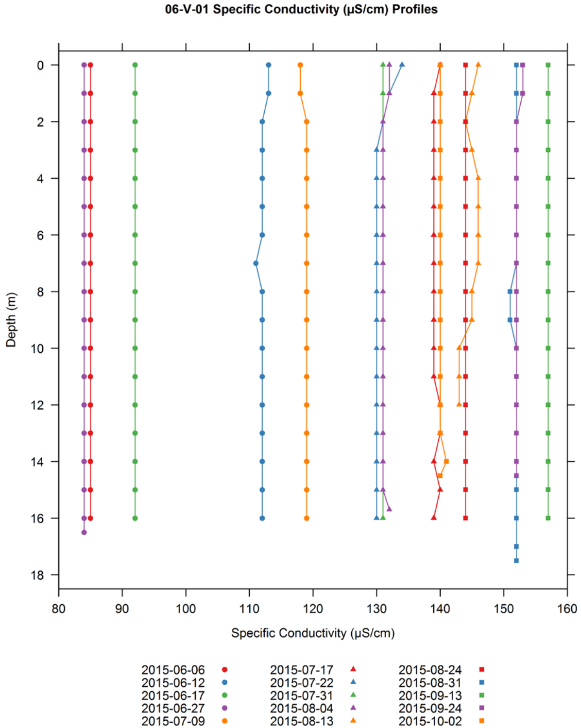
Figure H-82. Vertical profiles of specific conductivity ( \mu\text{S}/\text{cm} ) collected at the Vernon forebay 06-V-01 water quality monitoring station.
