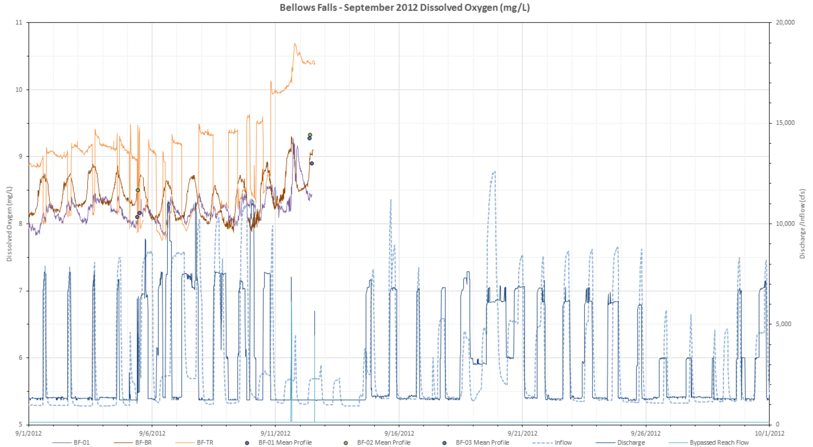
Figure L-20. 2012 September dissolved oxygen (mg/L) at all Bellows Falls stations with inflow (USGS Gage No. 01144500), bypassed reach flow, and Bellows Falls project discharge.
