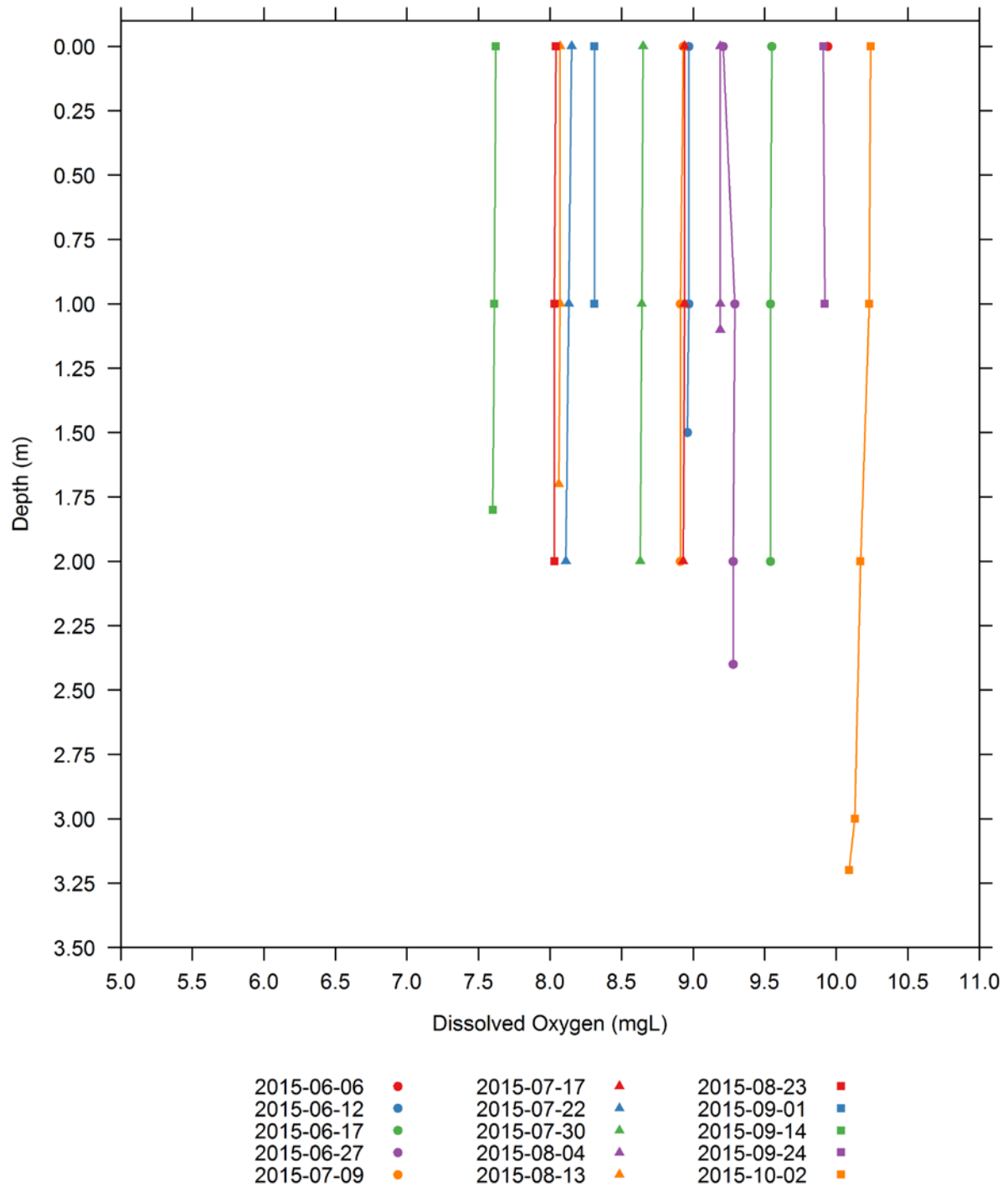
Figure H-62. Vertical profiles of dissolved oxygen (mg/L) collected at the Vernon upstream 06-V-04 water quality monitoring station.
