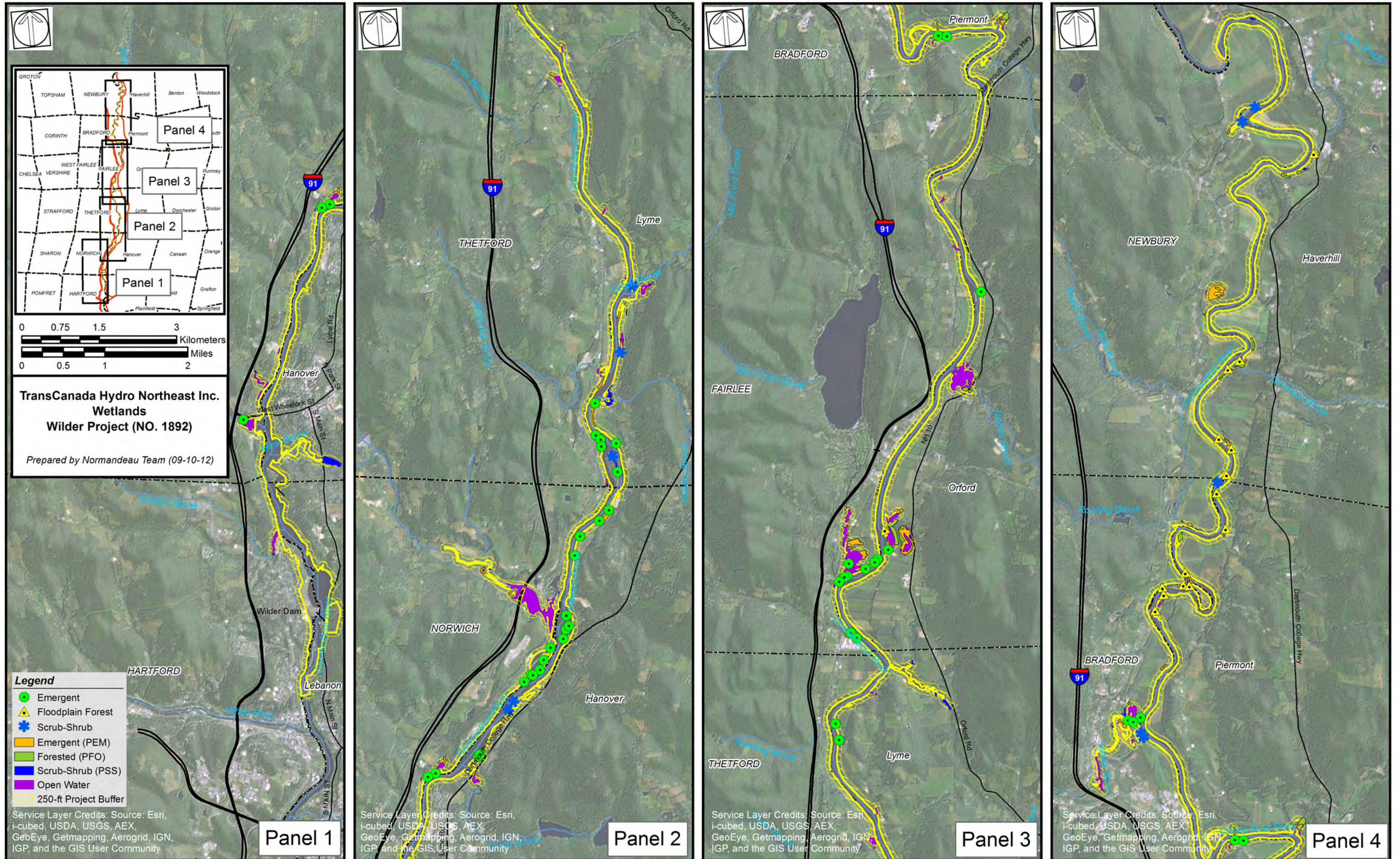
Figure 3.8-1. Wetlands maps.
