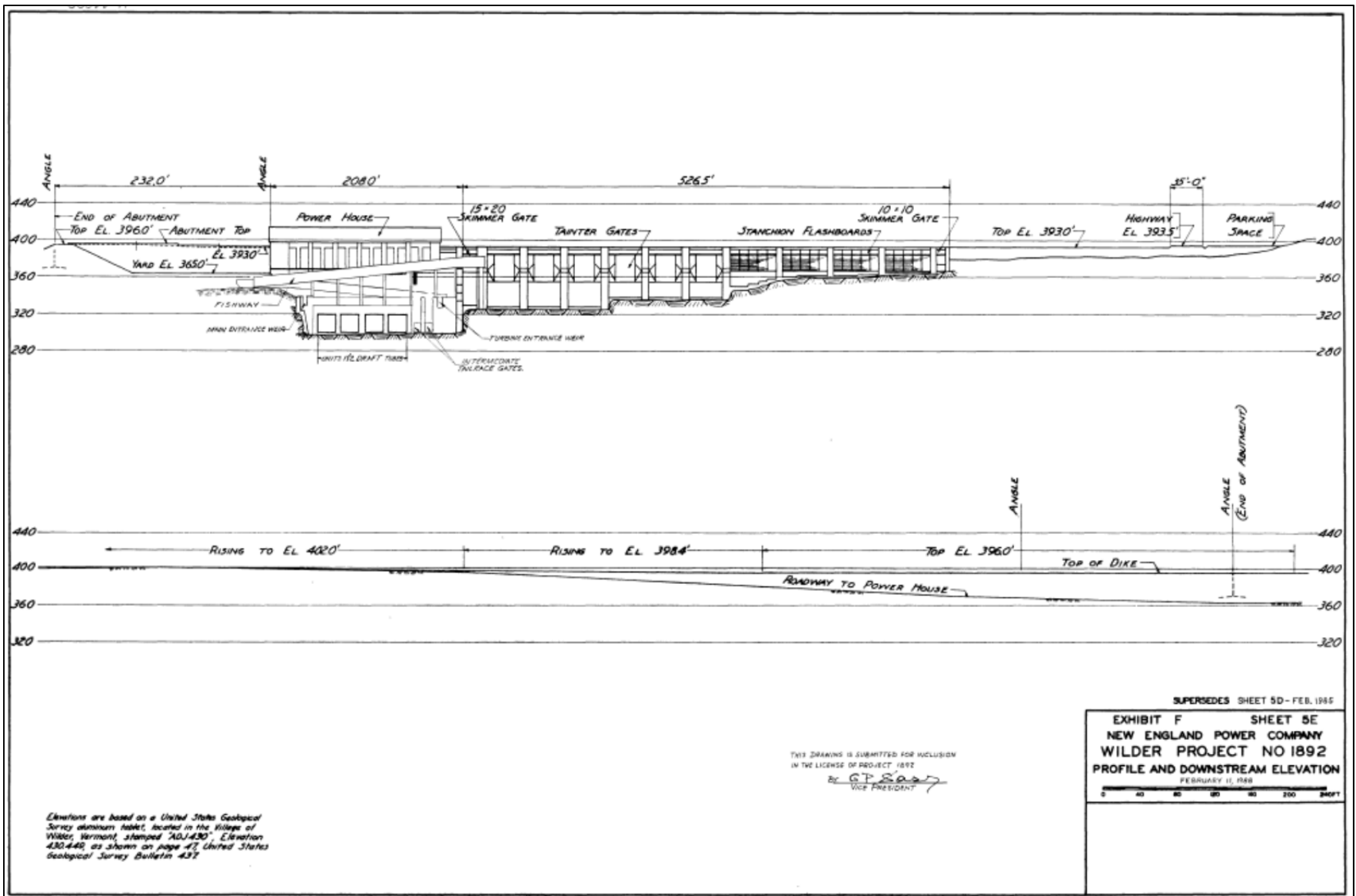
Figure 2.3-2. Spillway profile.
