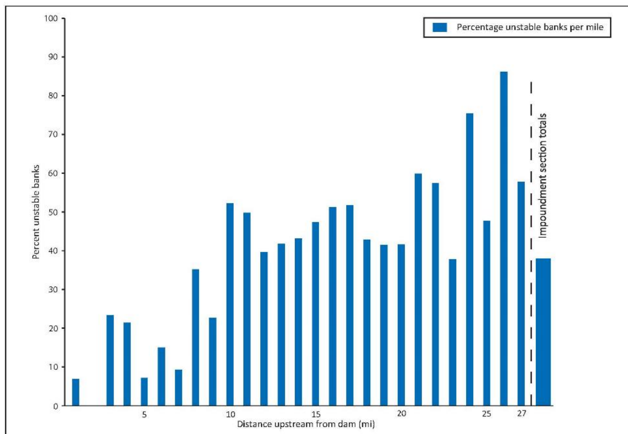
Figure 3.3-16. Variation in amounts of erosion with distance from Vernon dam.
