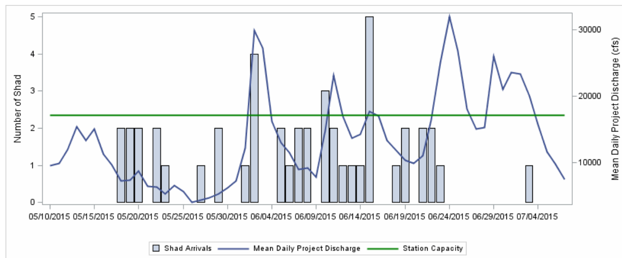
Figure 3.5-17. Distribution of forebay entry dates for radio-tagged adult American Shad approaching the Vernon dam during their downstream migration relative to mean daily project discharge (cfs), 2015.
