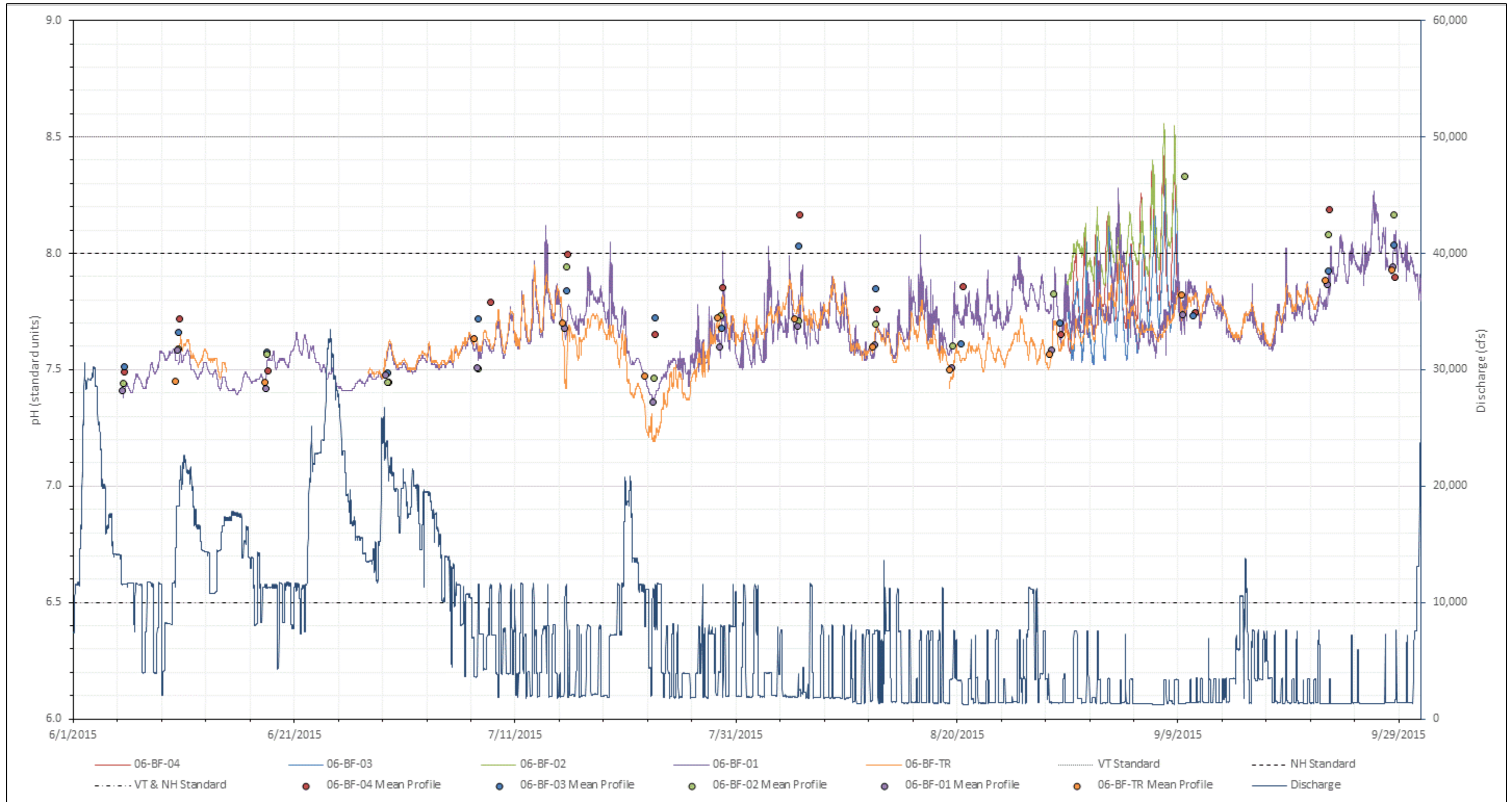
Figure 3.4-33. 2015 pH measured in the Bellows Falls forebay, bypassed reach, and tailrace, and at all stations during a 10-day, high-temperature, low-flow period with Bellows Falls discharge.
