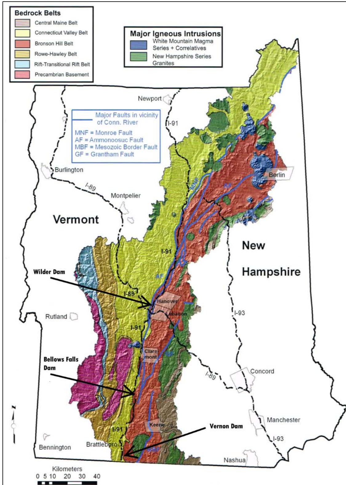
Figure 3.3-1. Bedrock geology in the Project areas.
