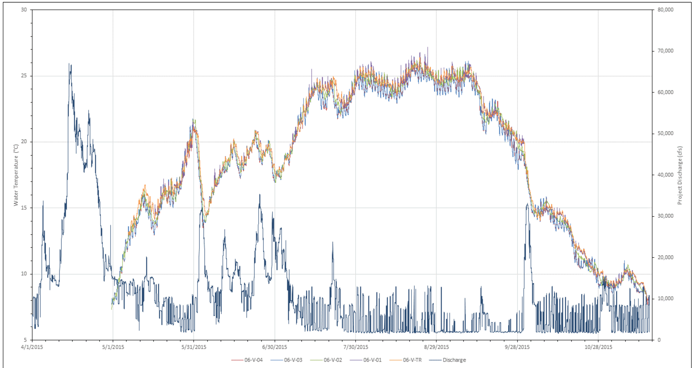
Figure 3.4-35. Vernon continuous water temperatures observed during spring, summer, and fall 2015 with Vernon discharge.
