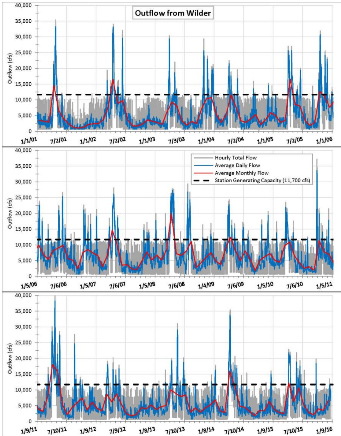
Figure 3.4-17. Hourly, average daily, and average monthly outflow from the Wilder Project (January 1, 2001–December 31, 2015).
