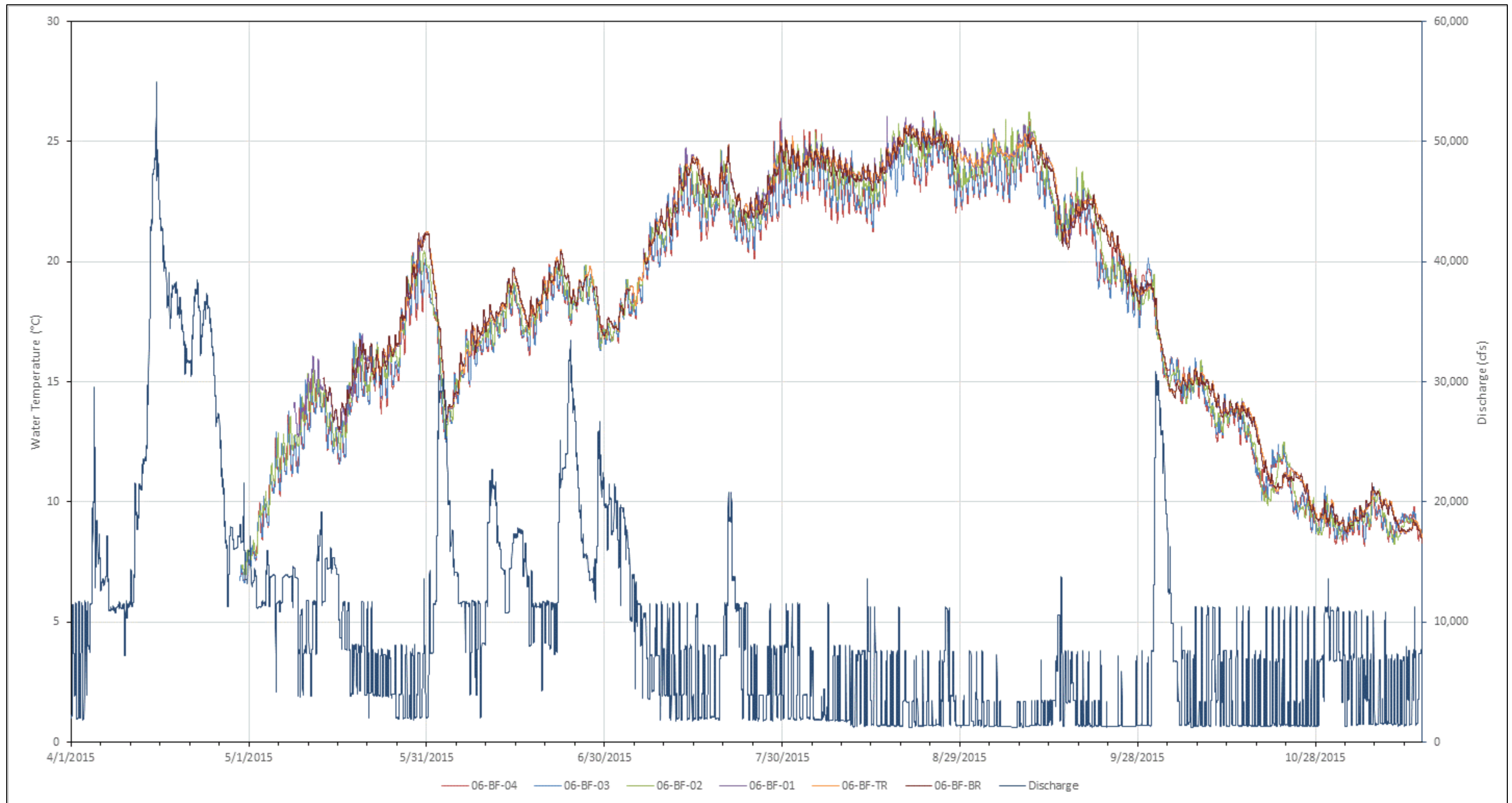
Figure 3.4-30. Bellows Falls continuous water temperatures observed during spring, summer, and fall 2015 with Bellows Falls discharge.
