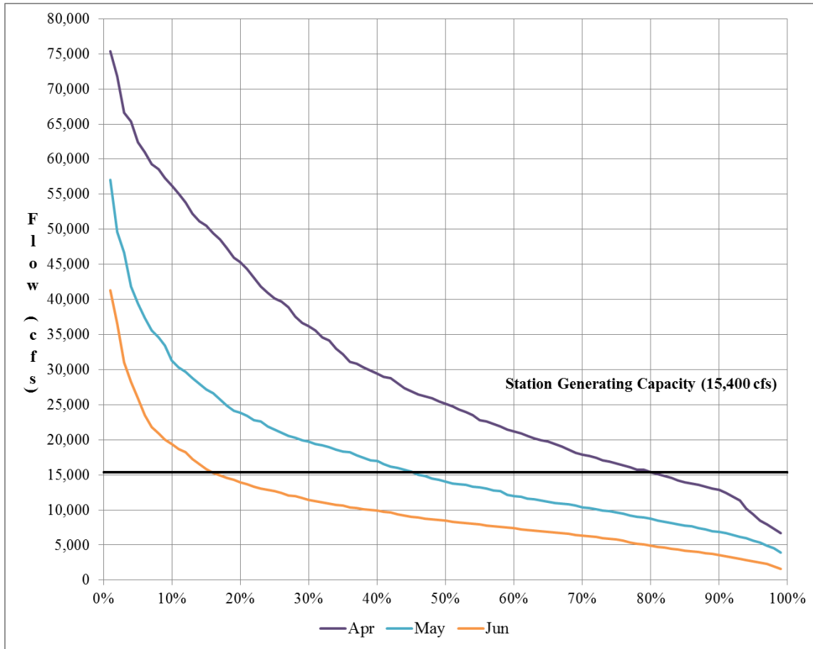
Figure 3.4-11. Vernon flow exceedance curves, April–June (based on flow data from January 1, 1979 to December 31, 2015).
