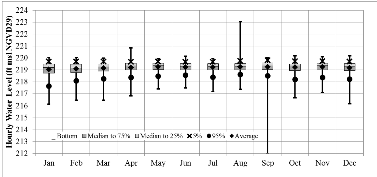
Figure 3.4-20. Vernon hourly impoundment elevations January 1, 2001–December 31, 2015.
