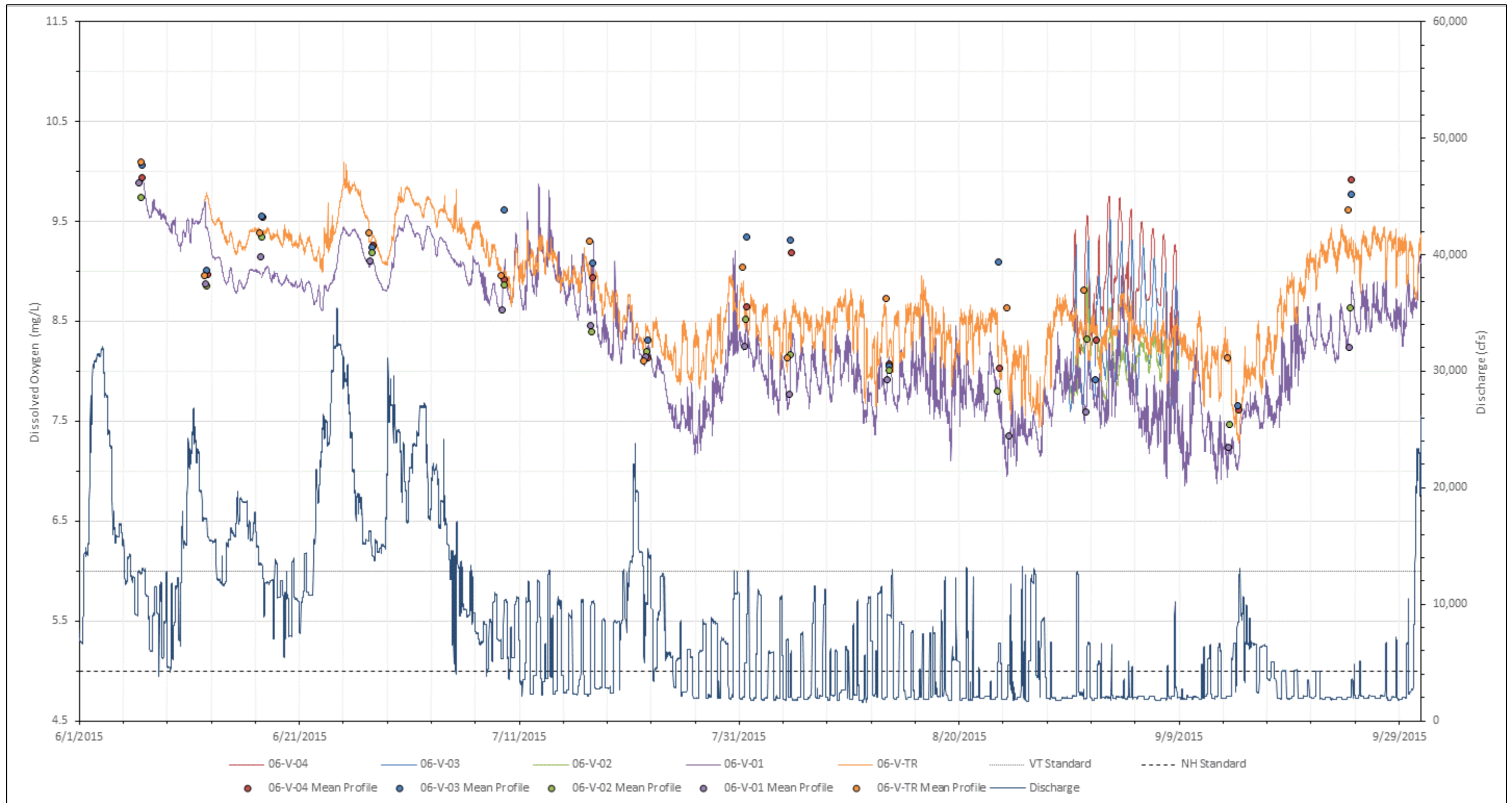
Figure 3.4-36. 2015 DO concentrations continuously measured in the Vernon forebay and tailrace, and at all stations during a 10-day, high-temperature, low-flow period with Vernon discharge.
