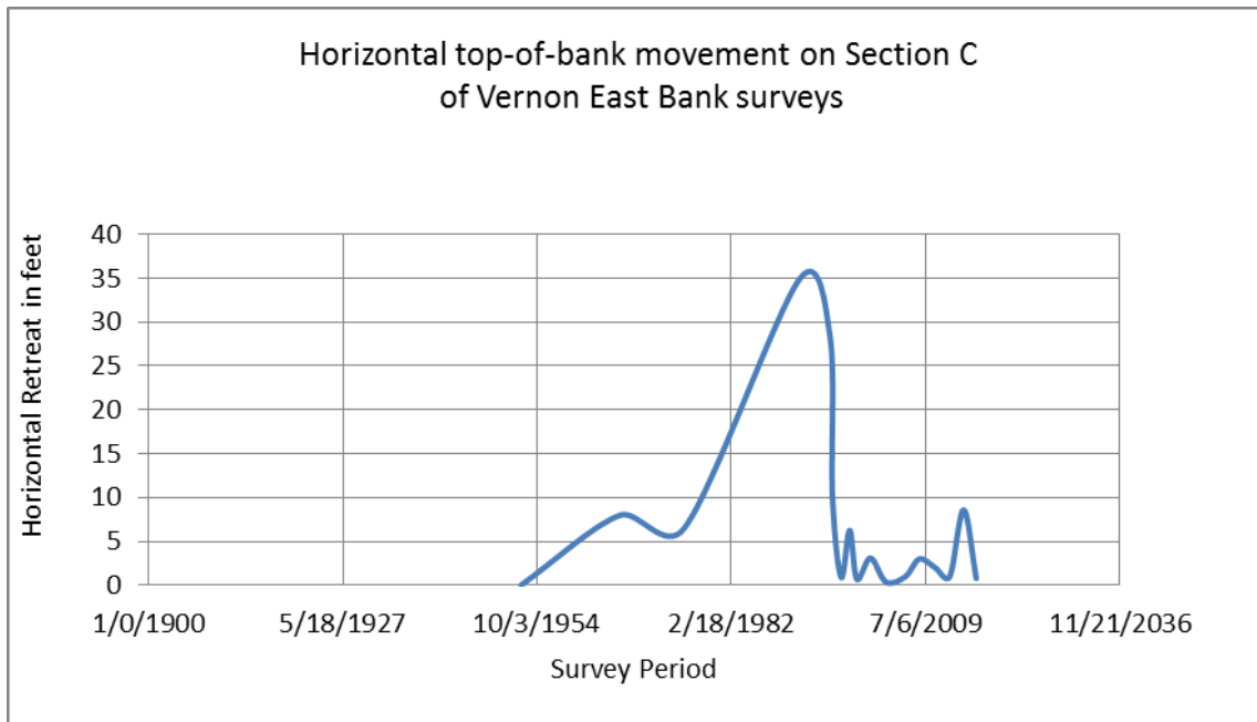
Figure 3.3-18. Vernon East Bank historical top-of-bank movement.
