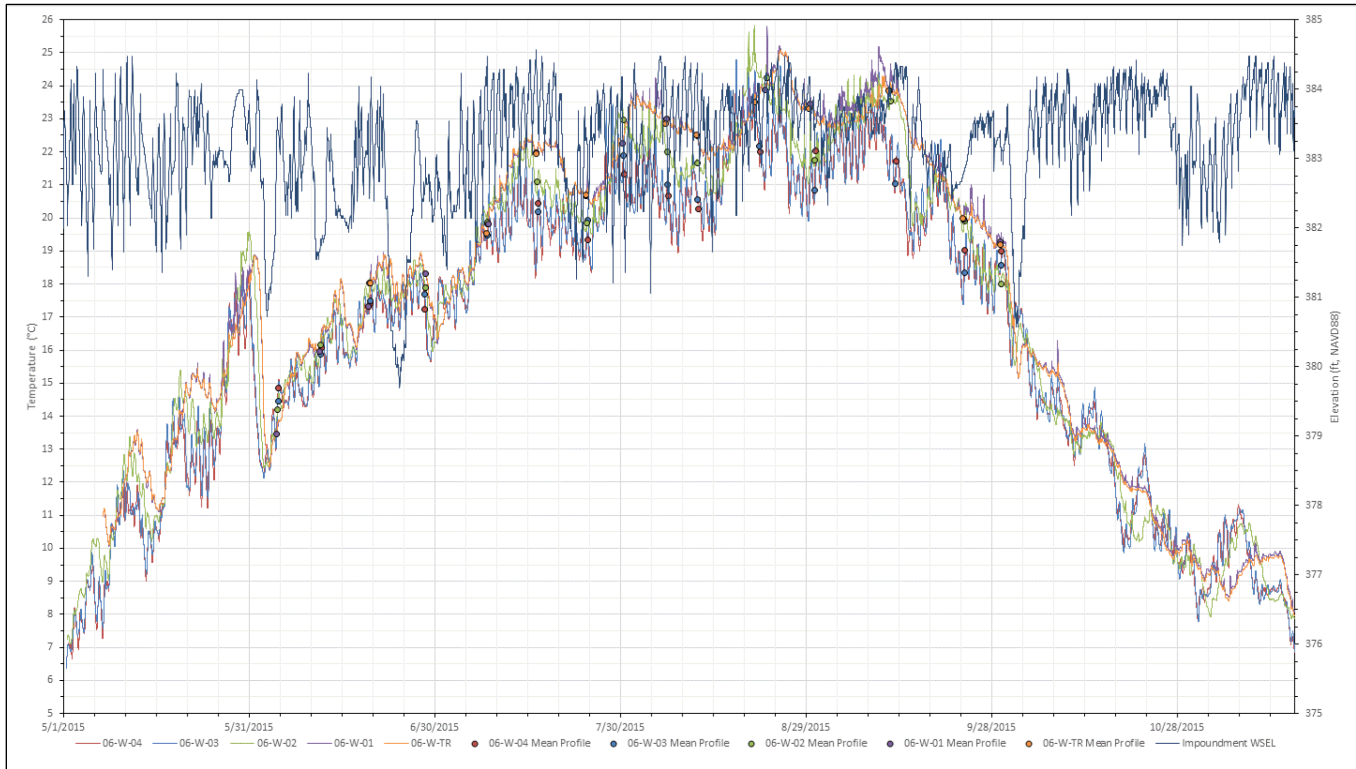
Figure 3.4-39. Wilder continuous water temperatures observed during spring, summer, and fall 2015 with Wilder impoundment water surface elevations.
