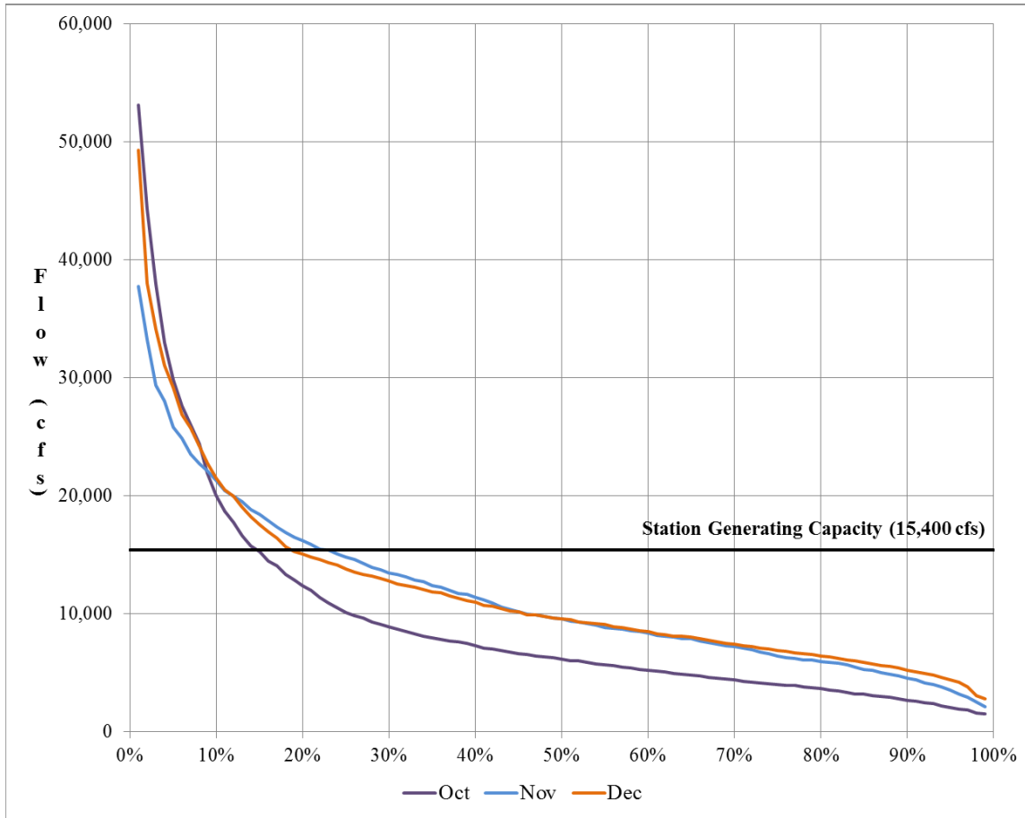
Figure 3.4-13. Vernon flow exceedance curves, October–December (based on flow data from January 1, 1979 to December 31, 2015).
