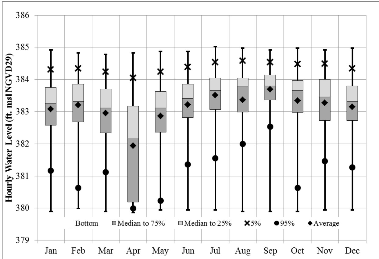
Figure 3.4-16. Wilder hourly impoundment water surface elevations January 1, 2001–December 31, 2015.
