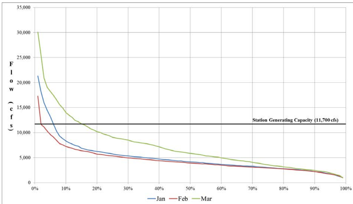
Figure 3.4-2. Wilder flow exceedance curves, January–March (based on flow data from January 1, 1979 to December 31, 2015).
