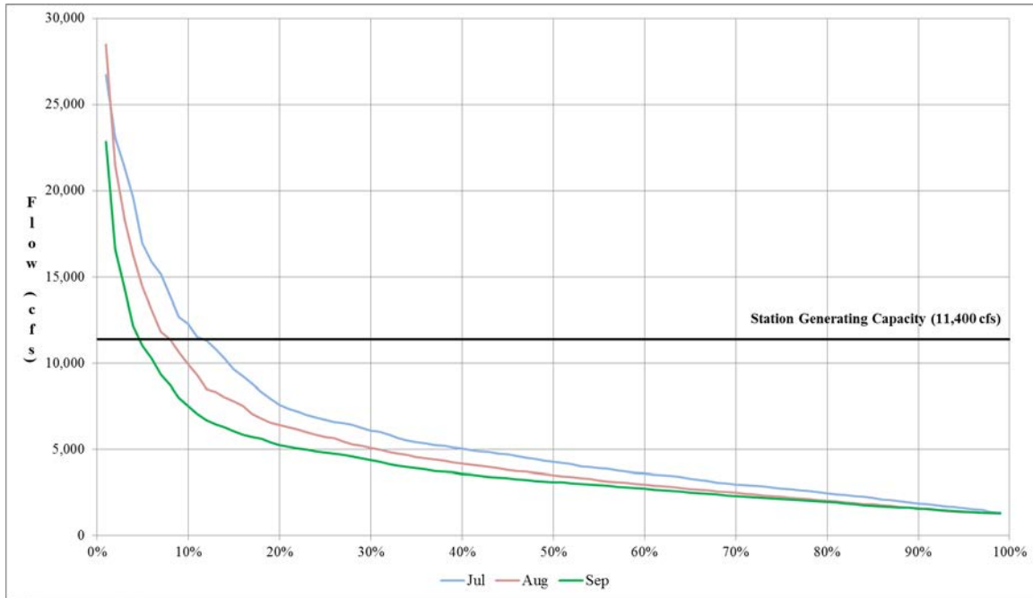
Figure 3.4-8. Bellows Falls flow exceedance curves, July–September (based on flow data from January 1, 1979 to December 31, 2015).
