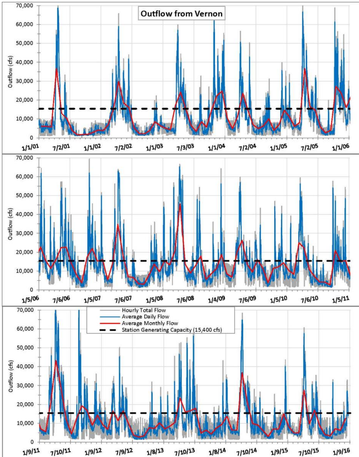
Figure 3.4-21. Hourly, average daily, and average monthly outflow from the Vernon Project (January 1, 2001–December 31, 2015).
