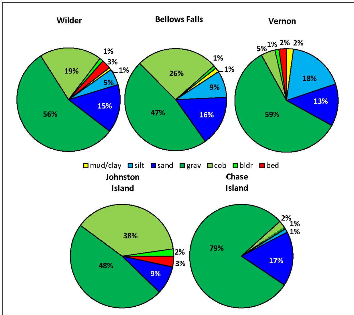
Figure 3.5-4. Percentage by length of dominant substrate types along 1D transects in the riverine reaches, and by area in the 2D study sites (Johnson and Chase Islands) in the Wilder riverine reach.
