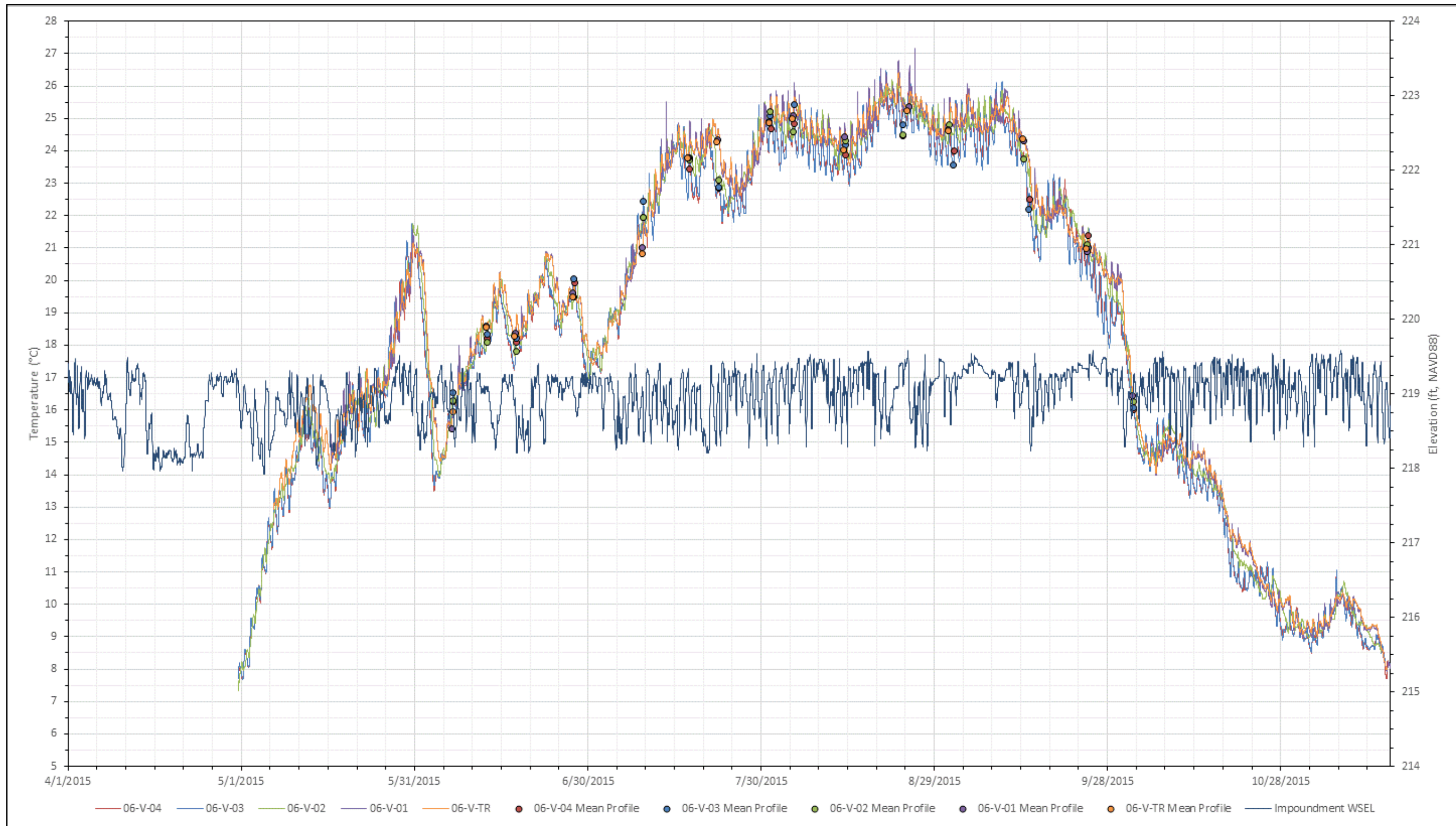
Figure 3.4-41. Vernon continuous water temperatures observed during spring, summer, and fall 2015 with Vernon impoundment water surface elevations.
