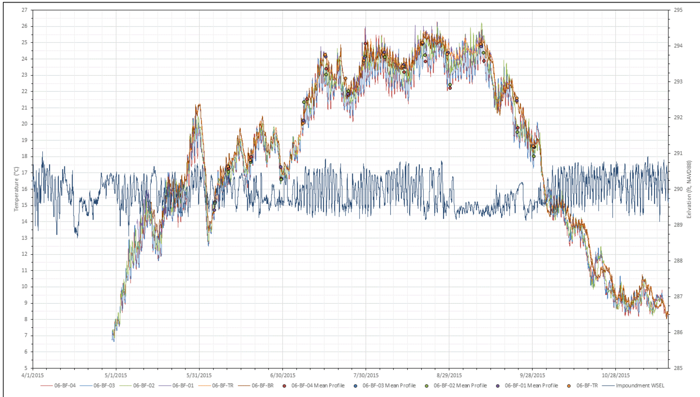
Figure 3.4-40. Bellows Falls continuous water temperatures observed during spring, summer, and fall 2015 with Bellows Falls impoundment water surface elevations.
