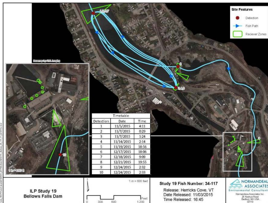
Figure 3.5-15. Example of eel wandering pattern prior to passage via the spillway at Bellows Falls, 2015.
