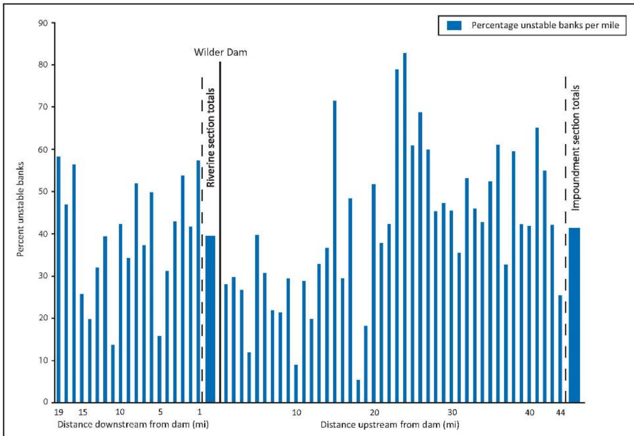
Figure 3.3-12. Variation in amounts of erosion with distance from Wilder dam.
