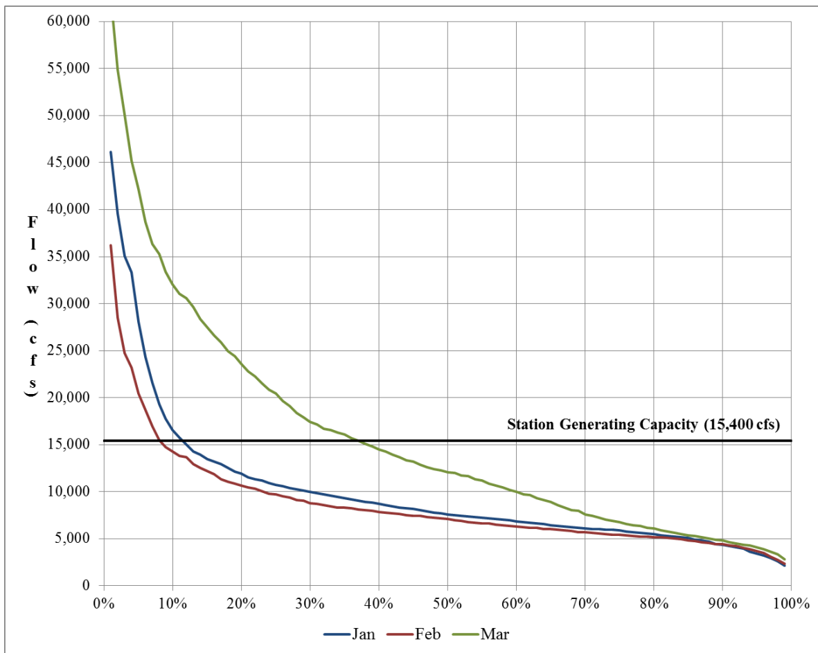
Figure 3.4-10. Vernon flow exceedance curves, January–March (based on flow data from January 1, 1979 to December 31, 2015).
