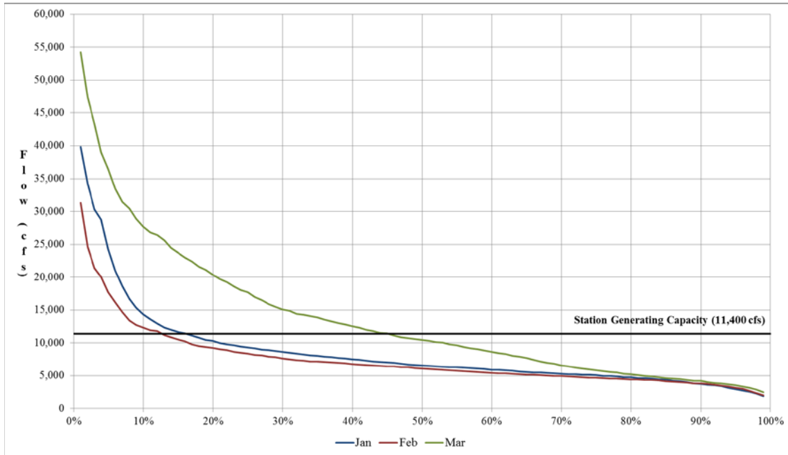
Figure 3.4-6. Bellows Falls flow exceedance curves, January–March (based on flow data from January 1, 1979 to December 31, 2015).
