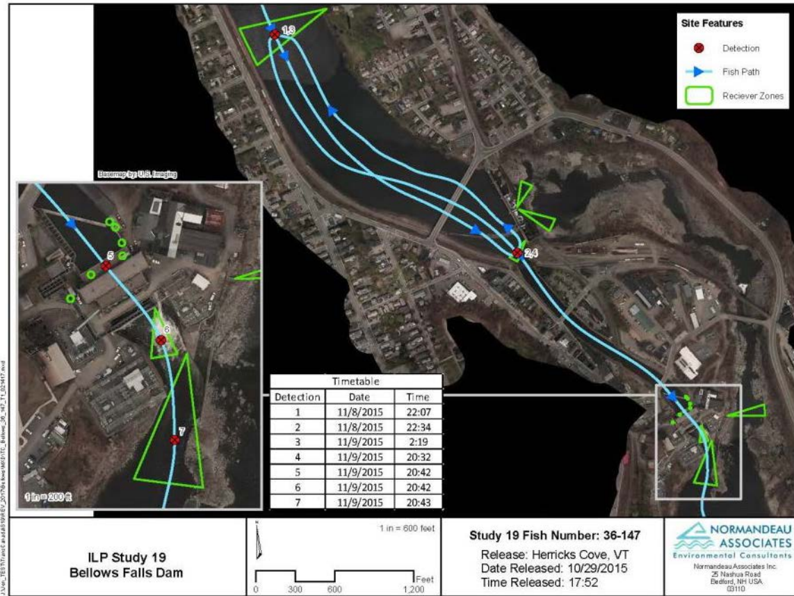
Figure 3.5-14. Example of eel wandering pattern prior to passage at Bellows Falls, 2015.
