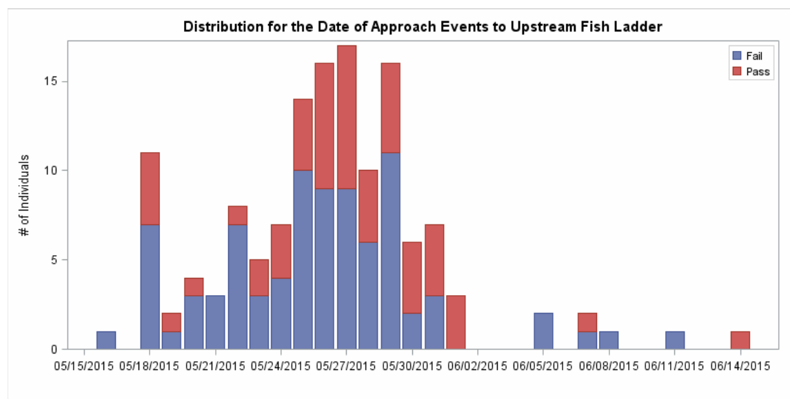
Figure 3.5-10. Distribution of the observed initiation dates for fish ladder approach events resulting in successful and unsuccessful American Shad upstream forays at Vernon, 2015.
