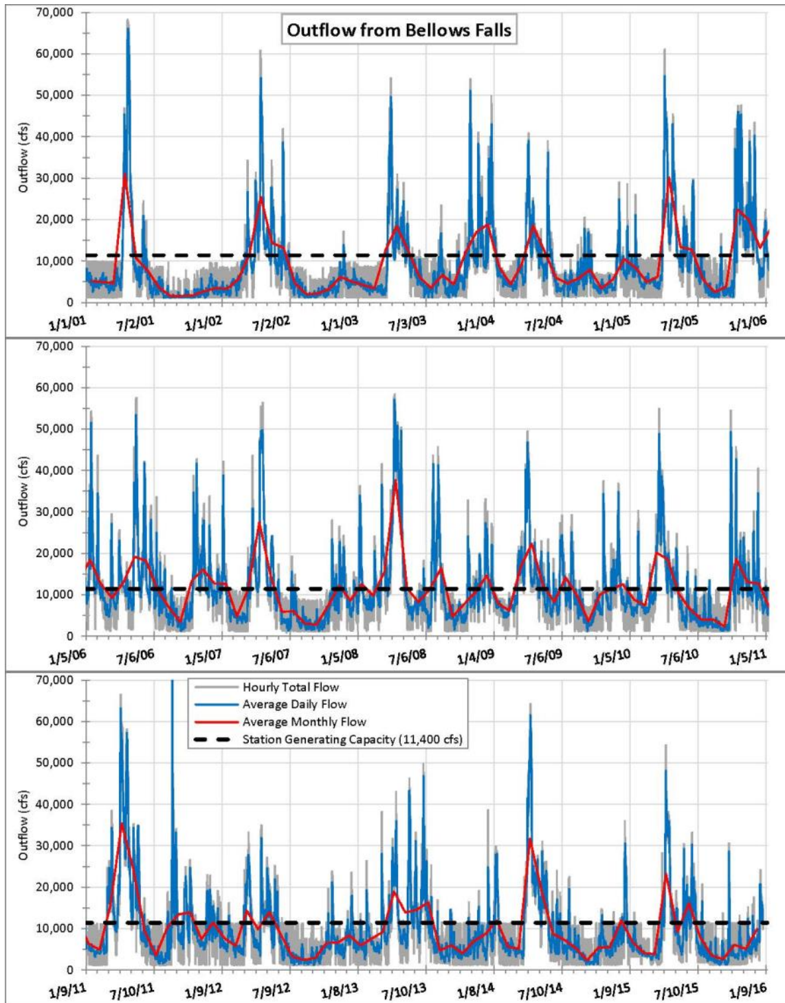
Figure 3.4-19. Hourly, average daily, and average monthly outflow from the Bellows Falls Project (January 1, 2001–December 31, 2015).
