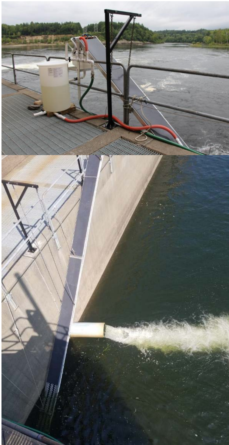
Source: ILP Study 18, American Eel Upstream Passage Assessment, Report Supplement Figure 3.5-9. Temporary eel trap and ramp, Vernon, 2016.
