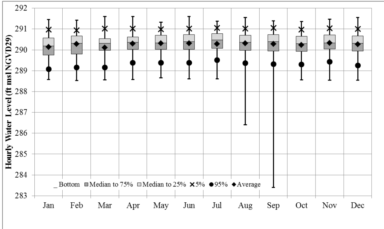
Figure 3.4-18. Bellows Falls hourly impoundment water surface elevations January 1, 2001–December 31, 2015.
