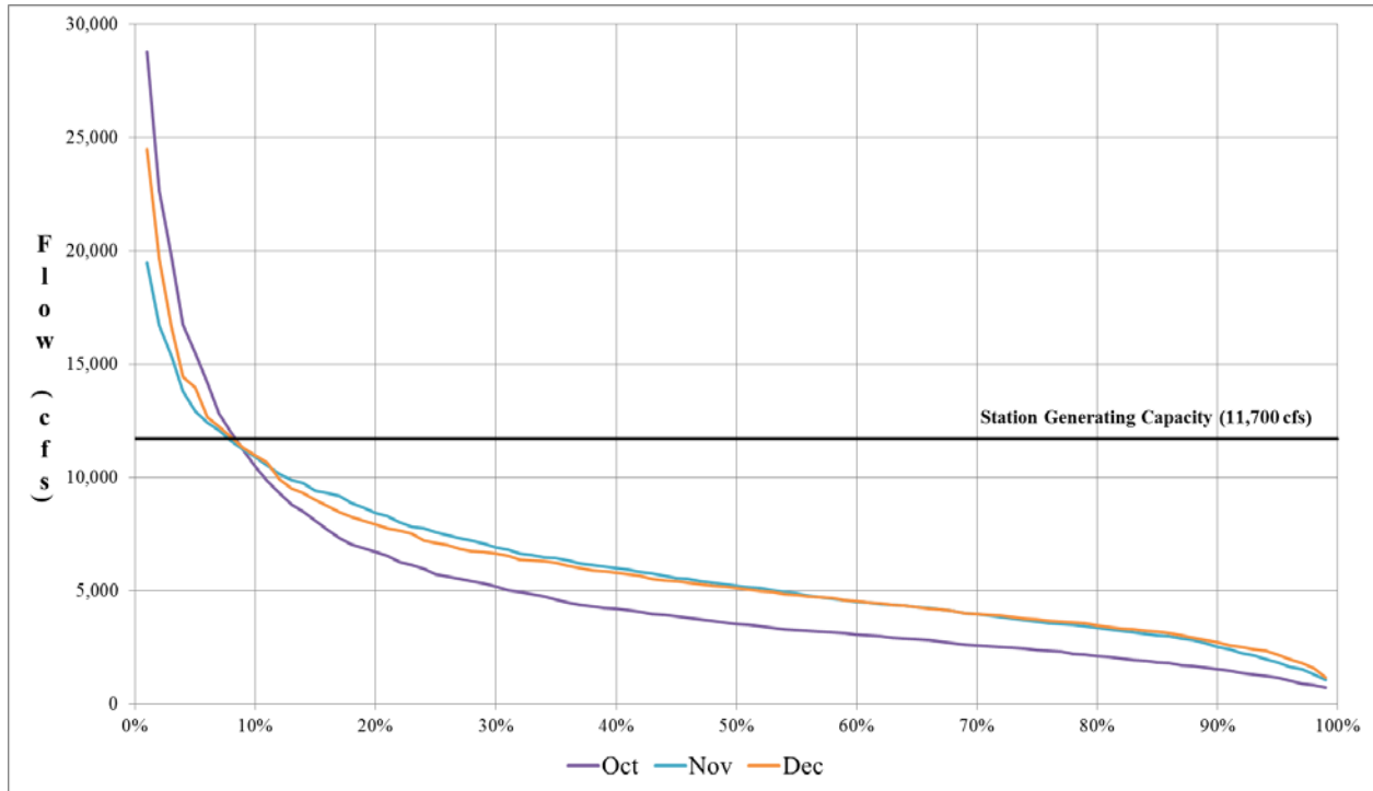
Figure 3.4-5. Wilder flow exceedance curves, October–December (based on flow data from January 1, 197, to December 31, 2015).
