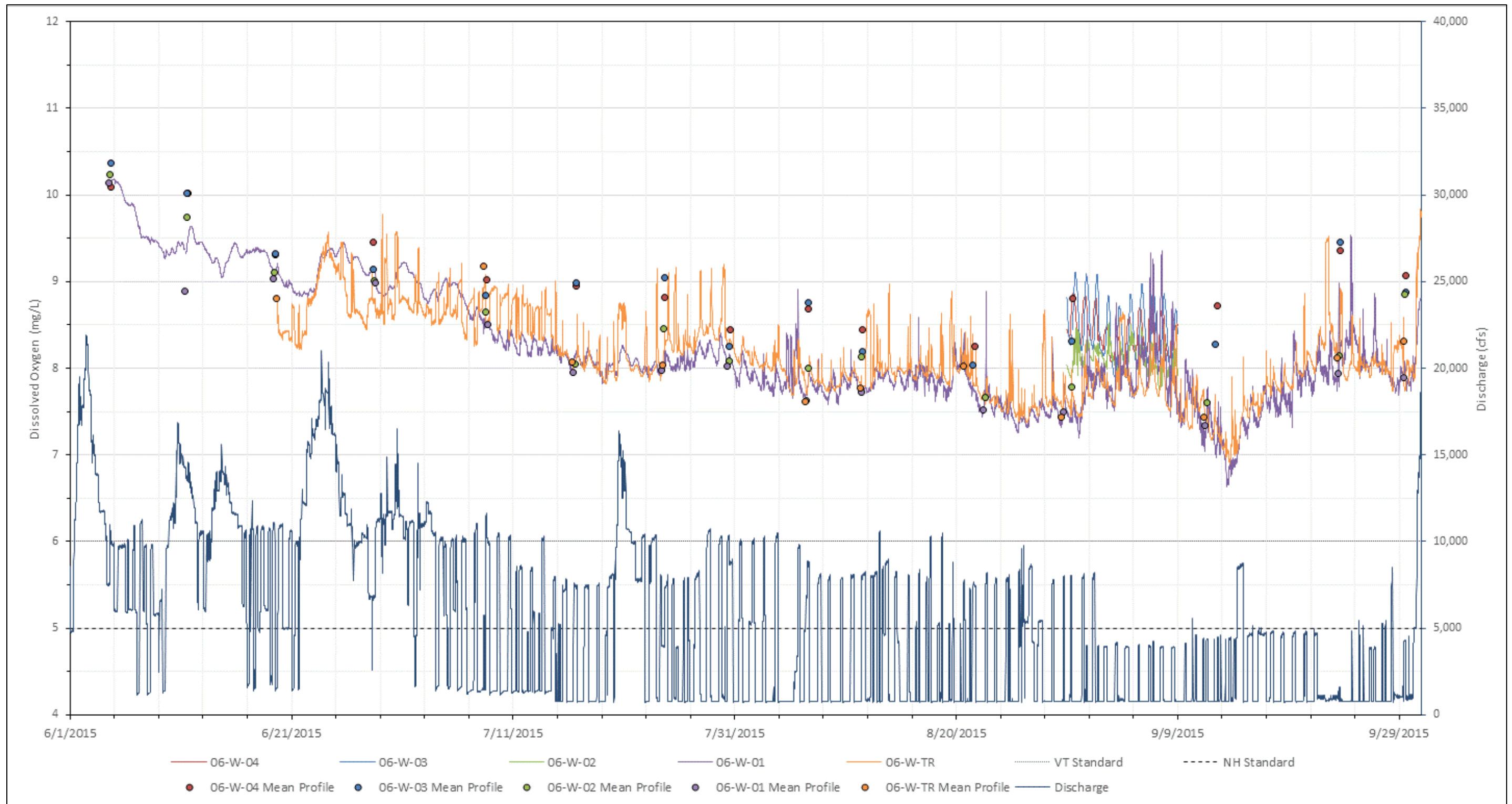
Figure 3.4-27. 2015 DO concentrations continuously measured in the Wilder forebay and tailrace, and at all stations during a 10-day, high-temperature, low-flow period with Wilder discharge.
