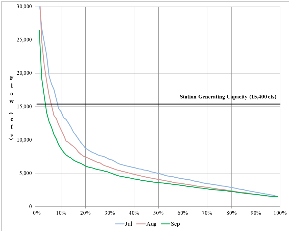
Figure 3.4-12. Vernon flow exceedance curves, July–September (based on flow data from January 1, 1979 to December 31, 2015).
