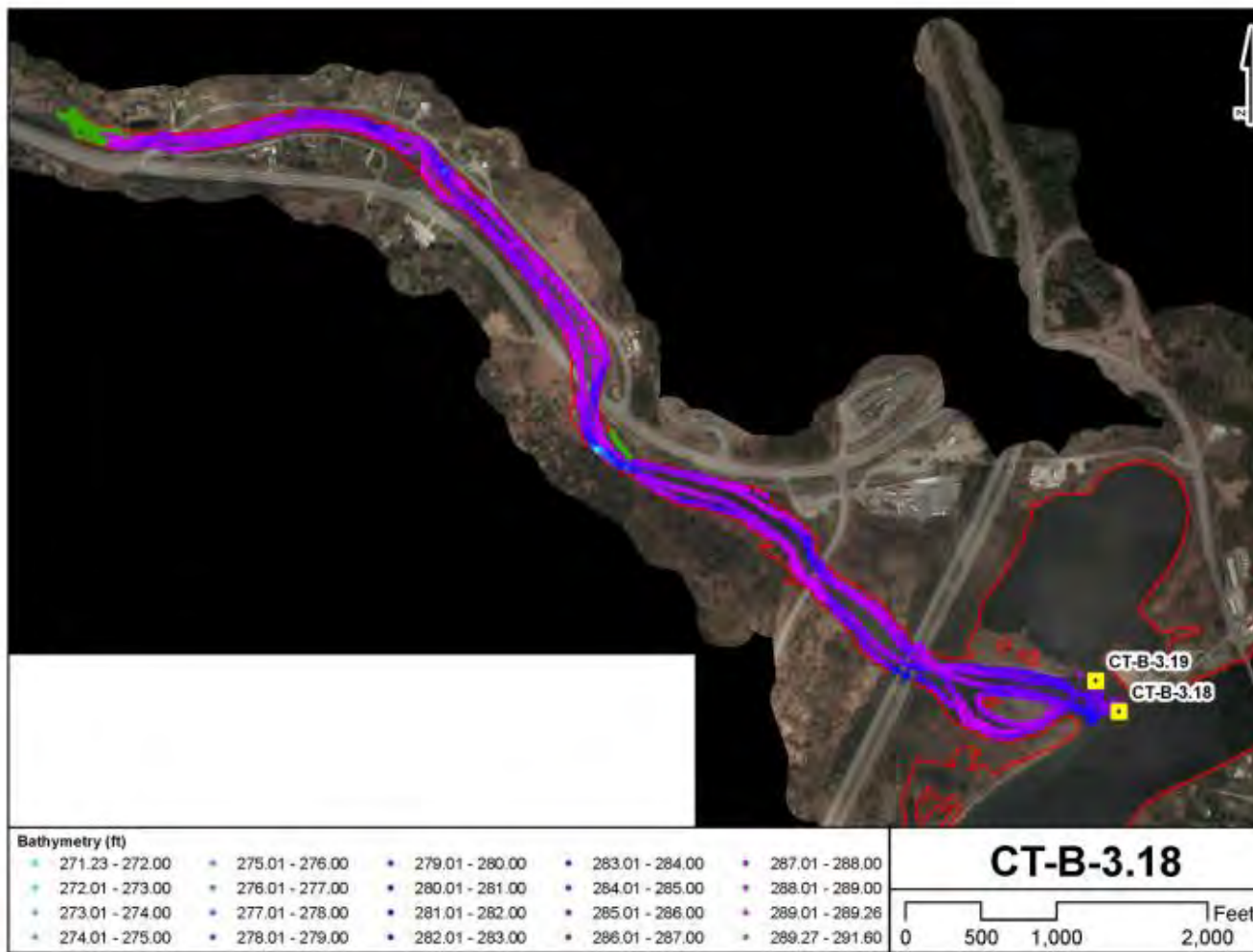
Figure C-15. Plan view of available bathymetry data at tributary site CT-B-3.18 (Black River, Stream Order 5). Color scale is relative to the low water elevation of 289.27' as recorded at level logger station 43 (green = dry, blue-pink = deeper-shallower).
