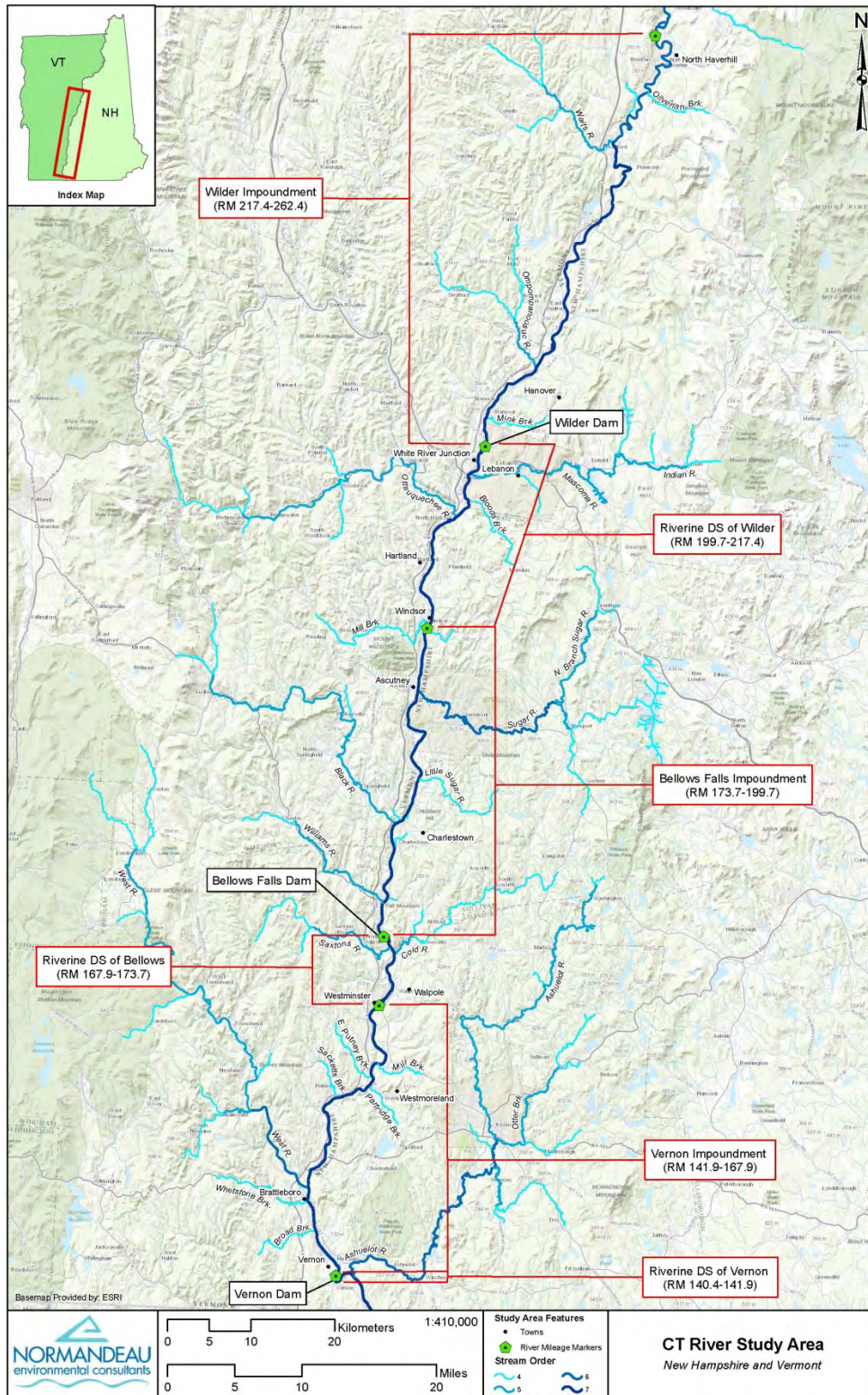
Figure 4-1. TransCanada Wilder, Bellows Falls, and Vernon hydroelectric projects study area.
