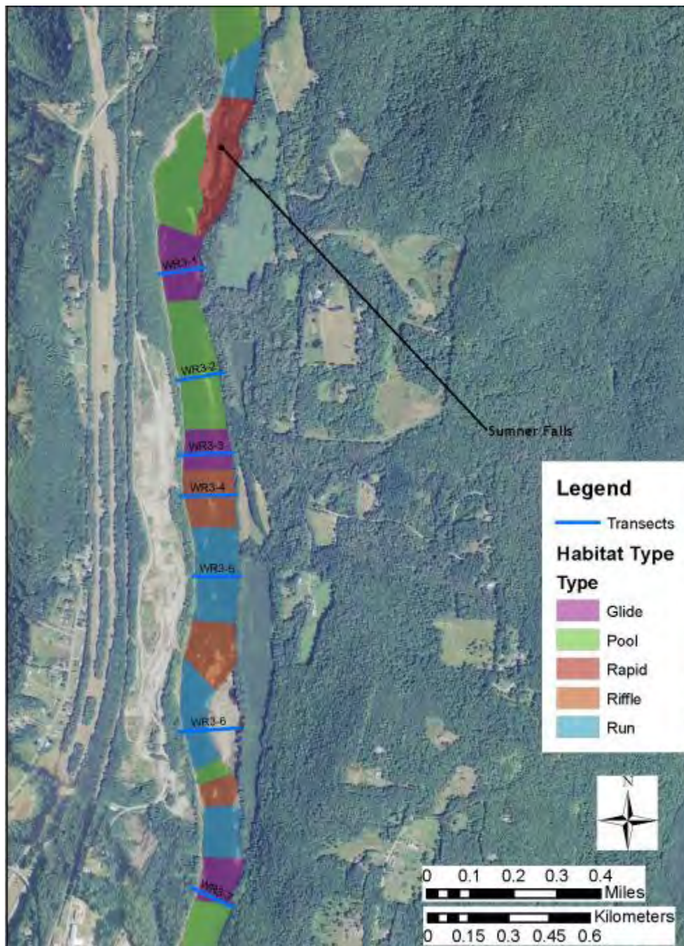
Figure 4-4. Mesohabitat types and proposed transect locations in upper portion of Wilder reach 3 - Ottauquechee River to Chase Island.
