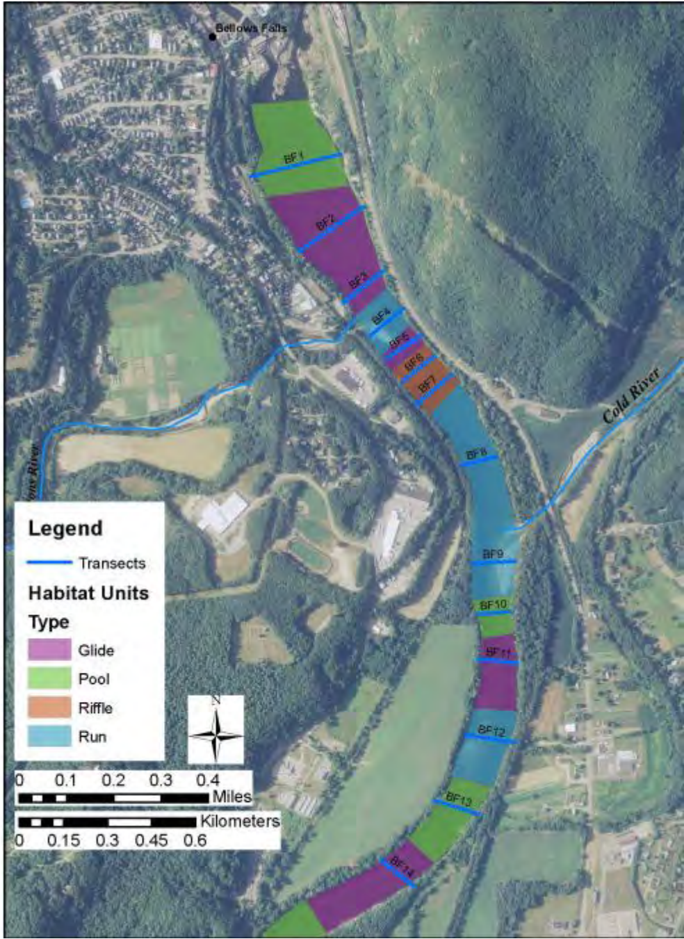
Figure 4-7. Mesohabitat types and proposed transect locations in the upper portion of the Bellows Falls reach.
