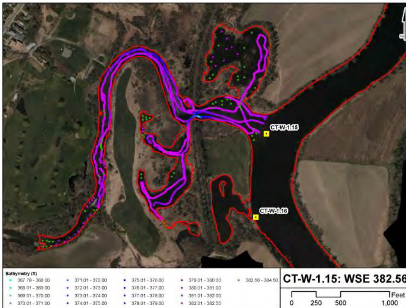
Figure C-3. Plan view of available bathymetry data at tributary site CT-W-1.15 (Waits River, Stream Order 5). Color scale is relative to the low water elevation of 382.56' as recorded at level logger station 5 (green = dry, blue-pink = deeper-shallower).
