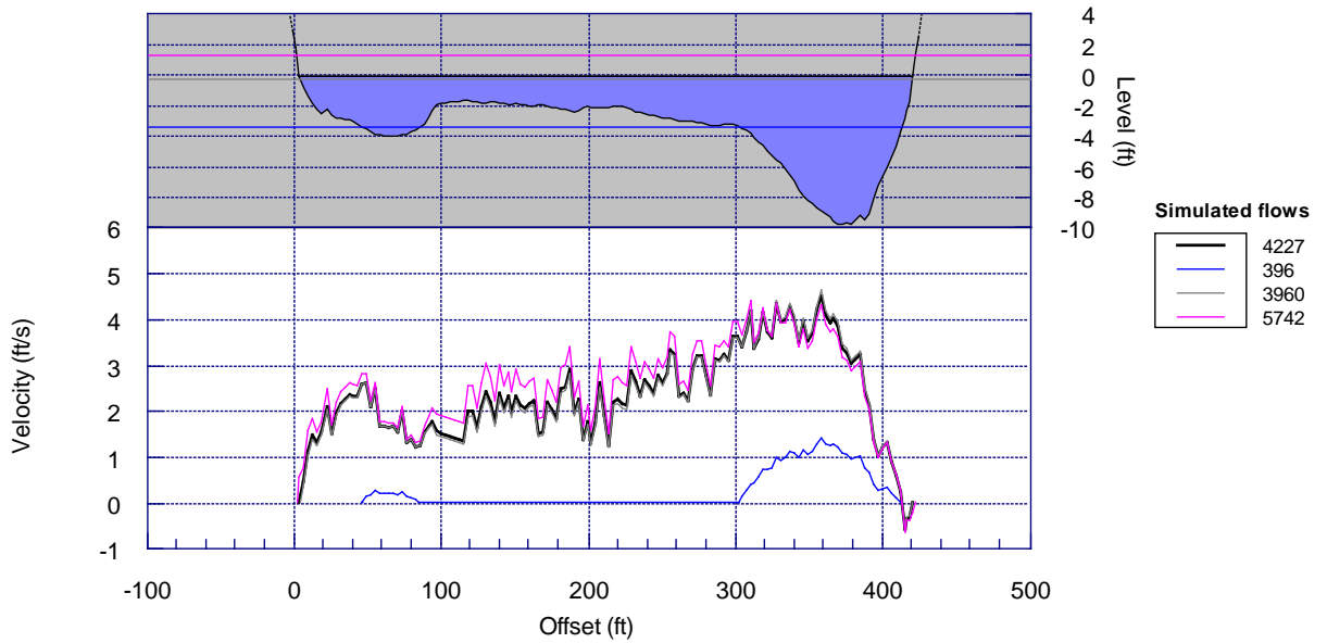
Cross-section: VR8 RC Run: Manning Ns applied IFG4 method
