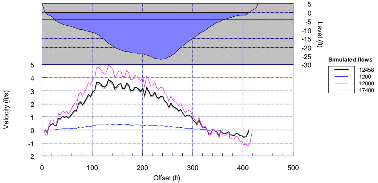
Cross-section: VR3 Pool: Manning Ns applied IFG4 method
