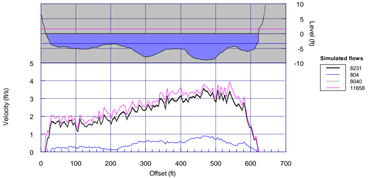
Cross-section: VR9 LC Glide: Manning Ns applied IFG4 method
