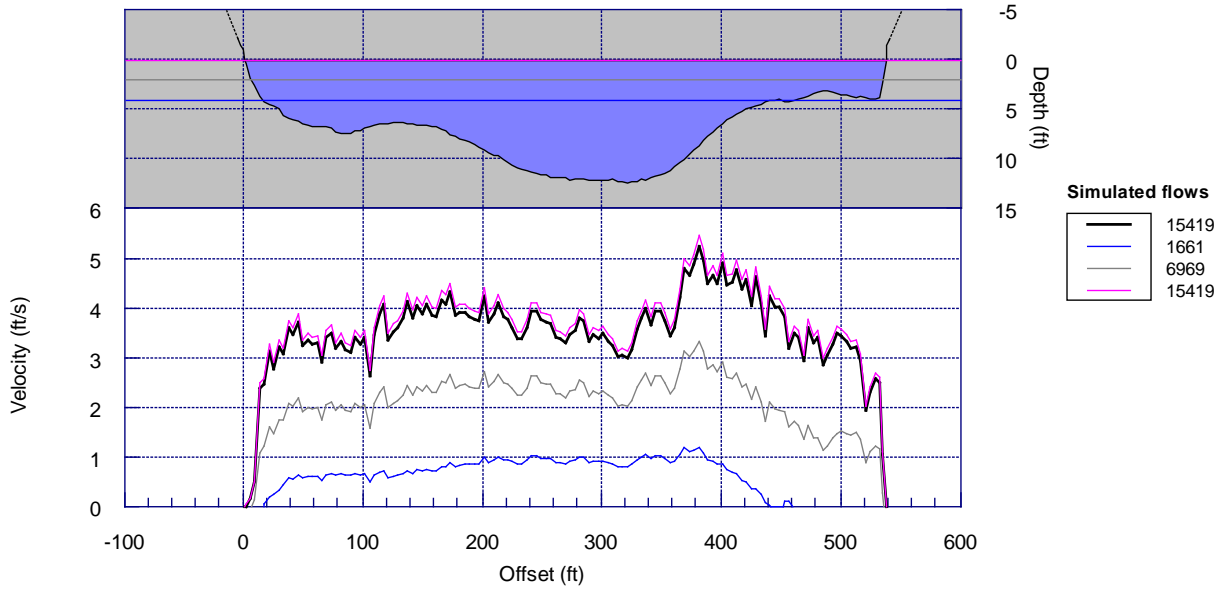
Cross-section: WR3-1 Glide: Manning Ns applied IFG4 method
