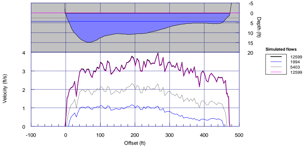
Cross-section: BF15 Pool: Manning Ns applied IFG4 method
