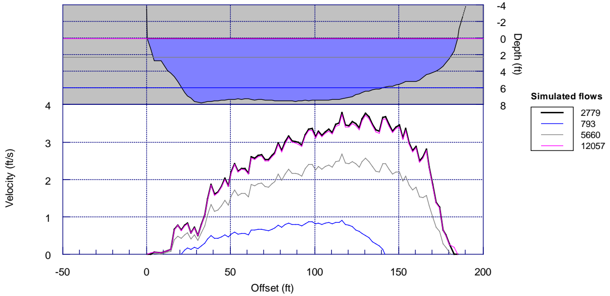
Cross-section: WR1-5 RC Run: Manning Ns applied IFG4 method
