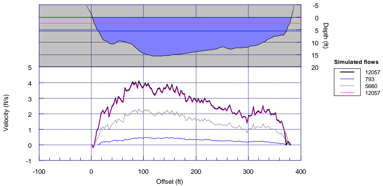
Cross-section: WR1-9 Pool: Manning Ns applied IFG4 method
