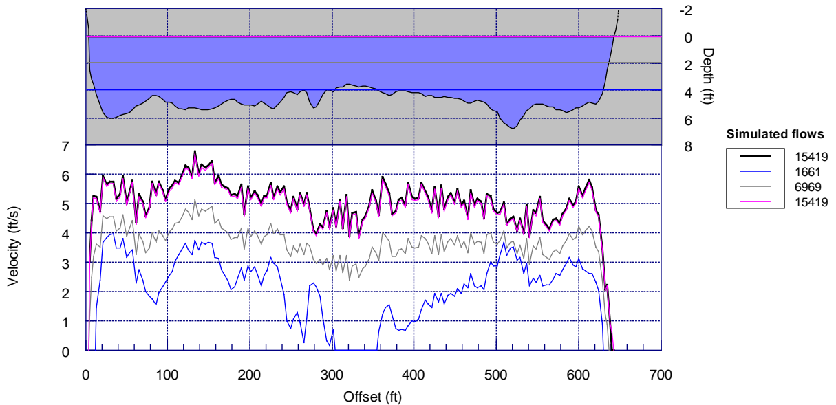
Cross-section: WR3-4 Riffle: Manning Ns applied IFG4 method
