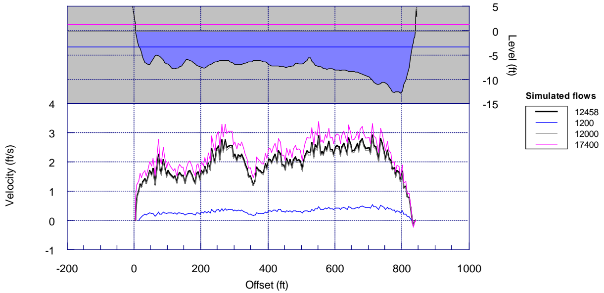
Cross-section: VR10 Pool: Manning Ns applied IFG4 method
