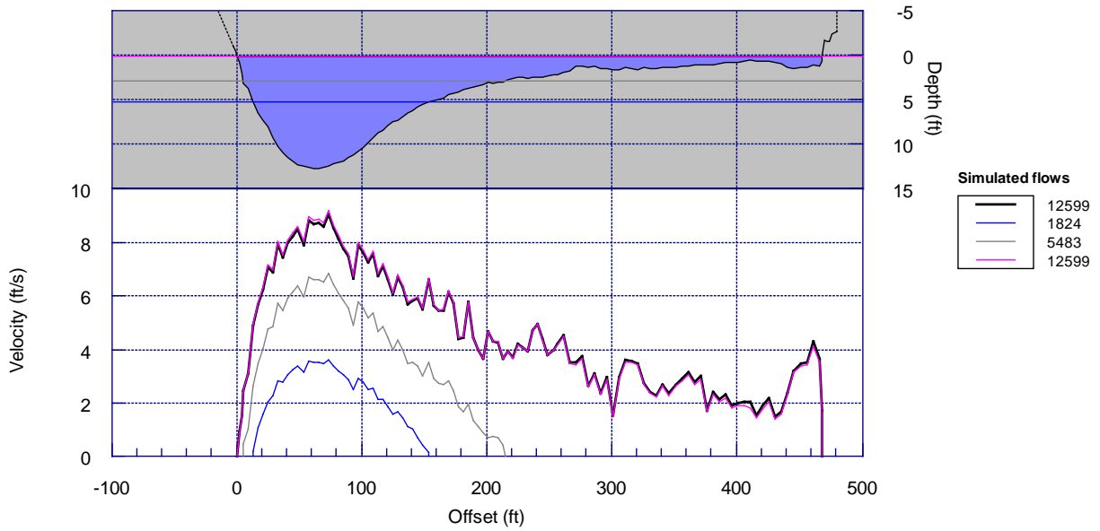
Cross-section: BF9 Run: Manning Ns applied IFG4 method
