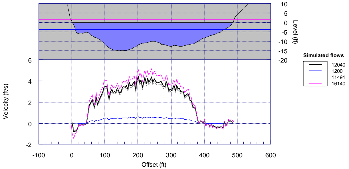
Cross-section: VR2 Run: Manning Ns applied IFG4 method
