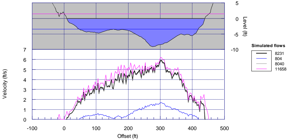
Cross-section: VR6 LC Run: Manning Ns applied IFG4 method
