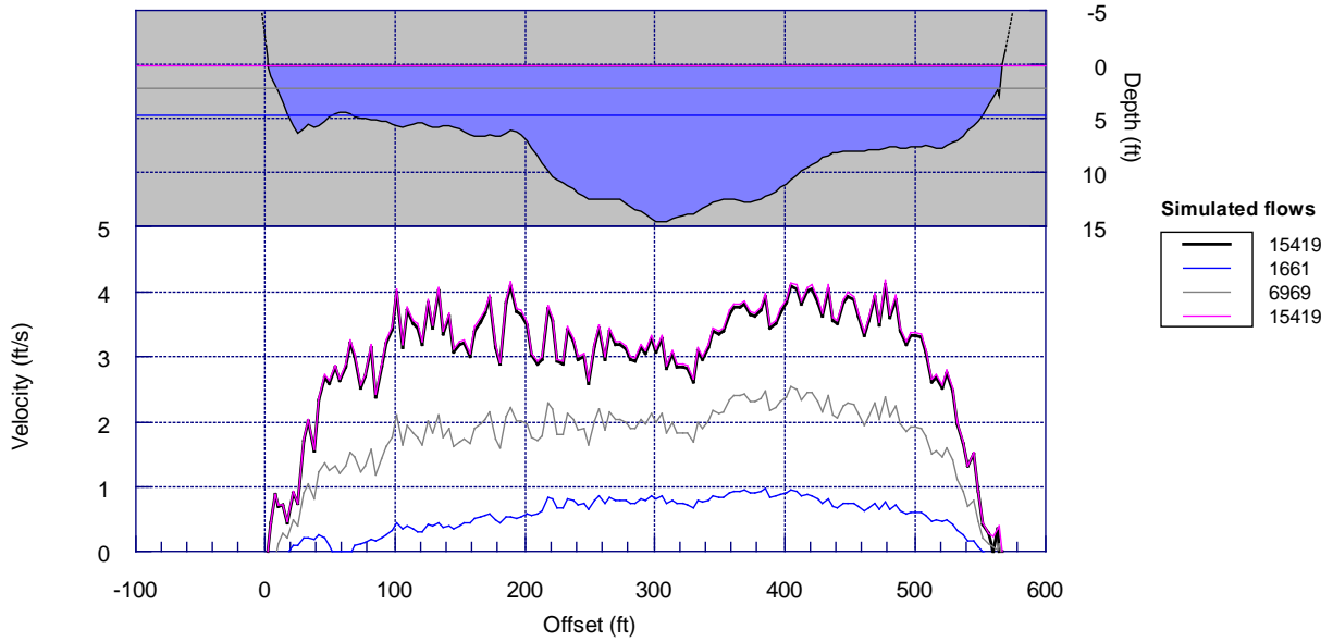
Cross-section: WR3-5 Run: Manning Ns applied IFG4 method
