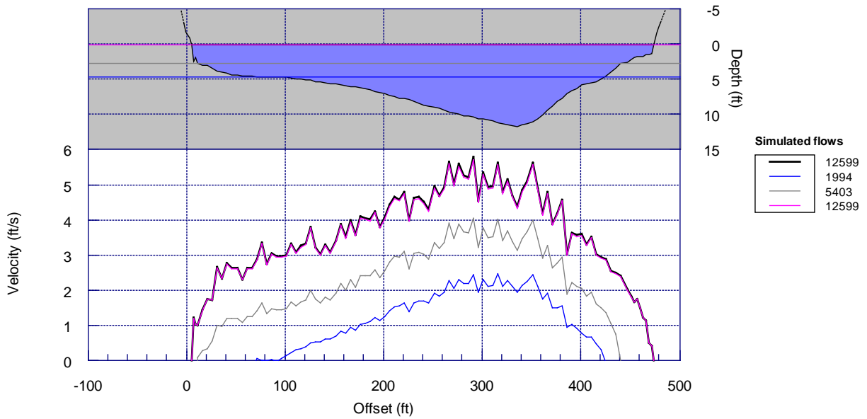
Cross-section: BF14 Glide: Manning Ns applied IFG4 method
