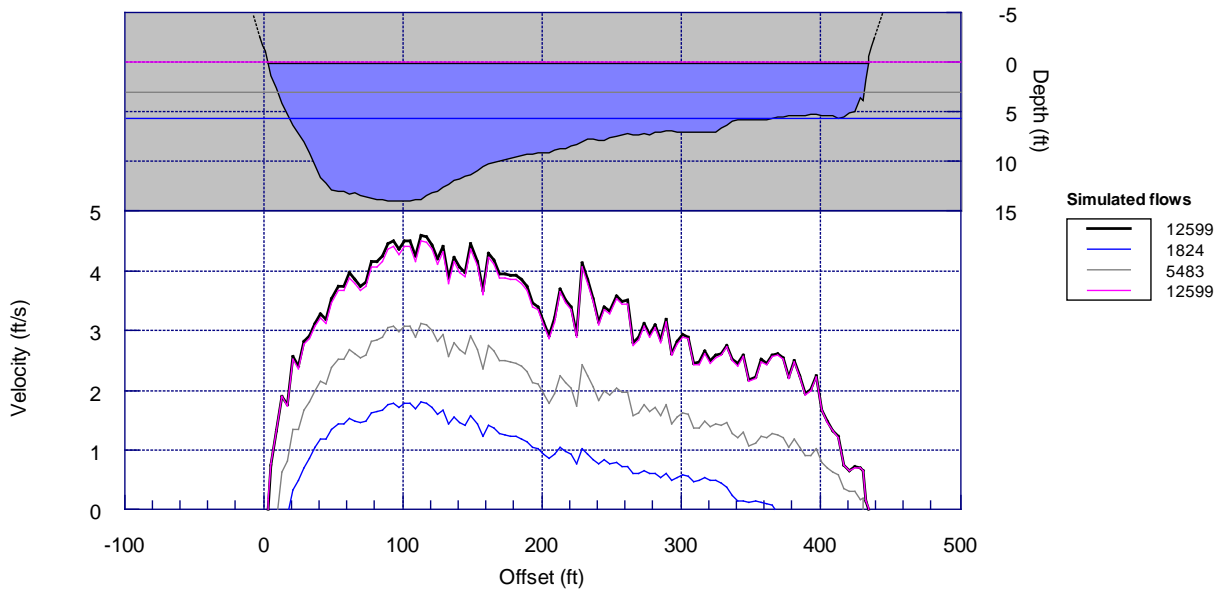
Cross-section: BF8 Run: Manning Ns applied IFG4 method
