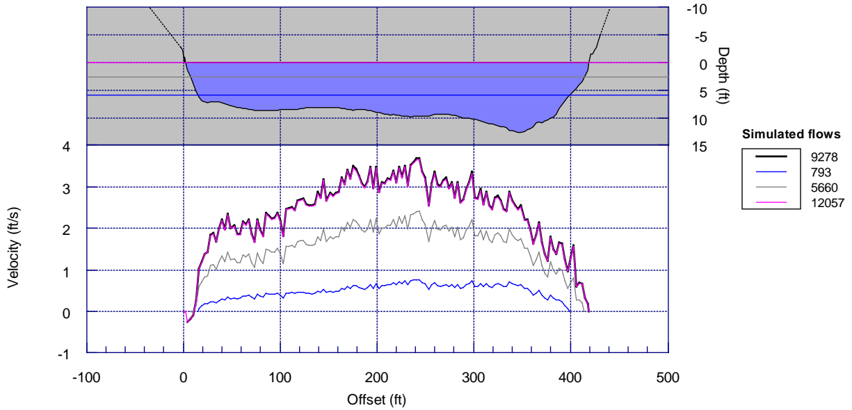
Cross-section: WR1-5 LC Glide: Manning Ns applied IFG4 method
