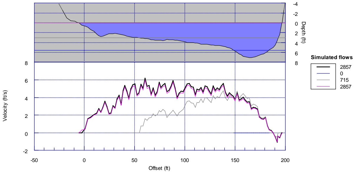
Cross-section: WR3-3 SC Riffle: Manning Ns applied IFG4 method
