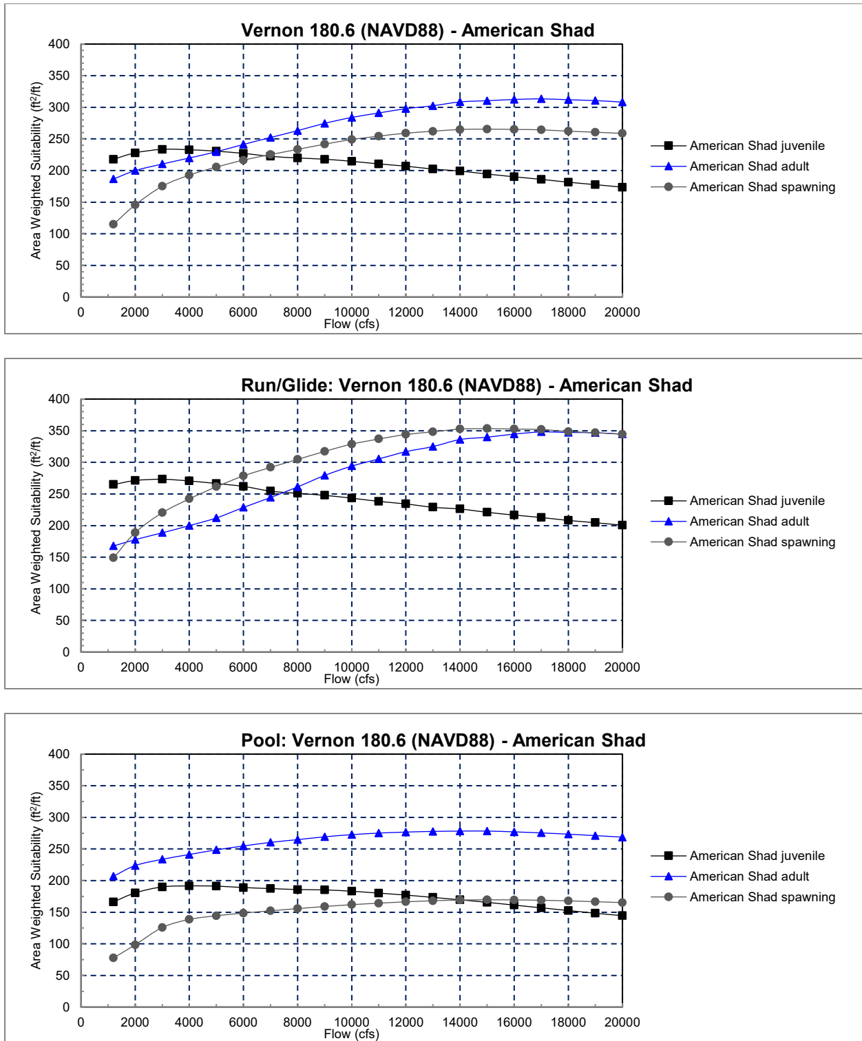
Figure 5.4-40. American Shad AWS for Vernon reach, and by habitat groups run/glide and pool at Turners Falls dam WSE of 180.6 ft (NAVD88).
