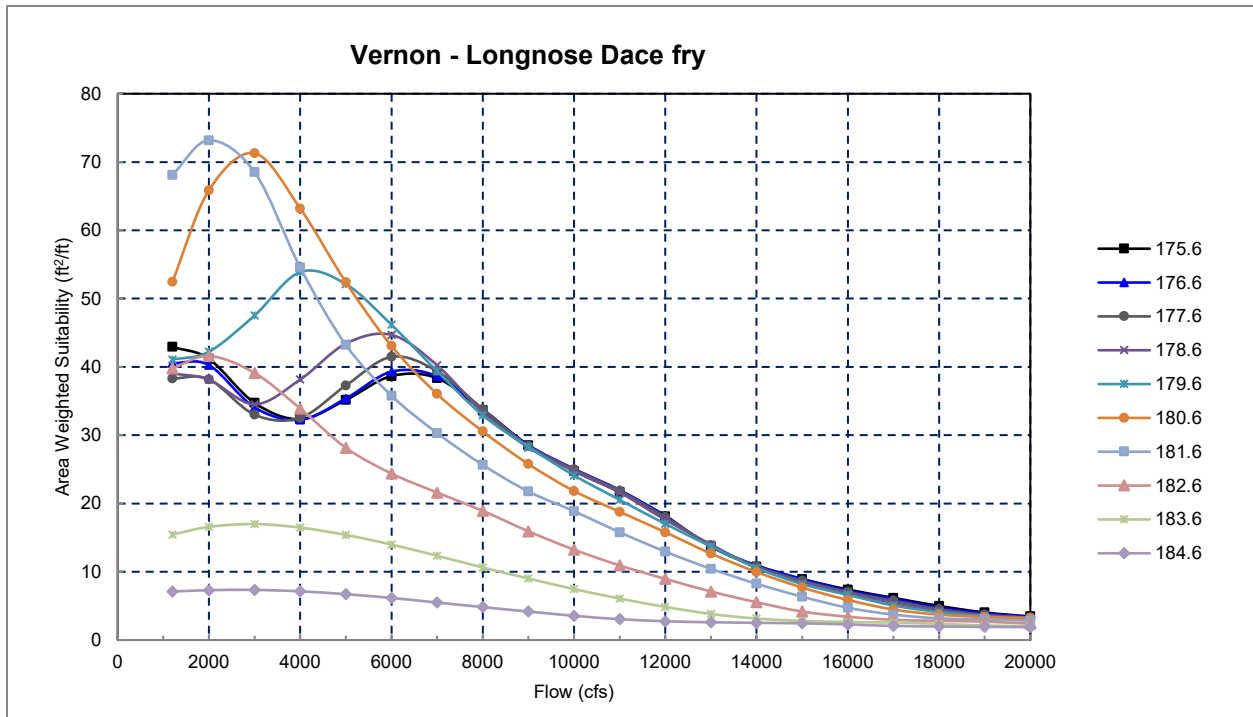
Figure 6.3.2-7. AWS curves for Longnose Dace fry at 10 Turners Falls elevations (ft NAVD88) in the Vernon riverine reach.
