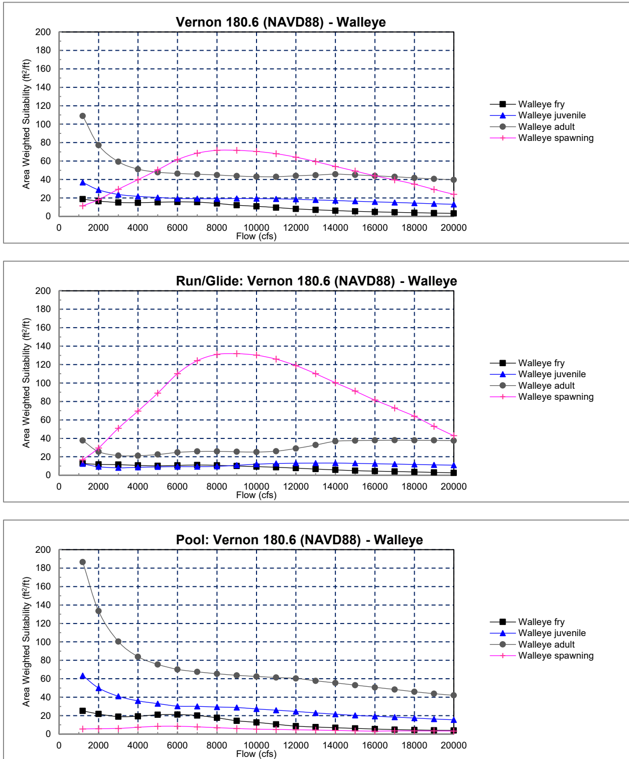
Figure 5.4-41. Walleye AWS for Vernon reach, and by habitat groups run/glide and pool at Turners Falls dam WSE of 180.6 ft (NAVD88).
