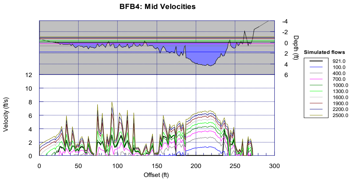
Figure 5.5-10. Measured middle flow velocities (black line) and simulated velocities for transect BFB4 in the Bellows Falls bypassed reach.
