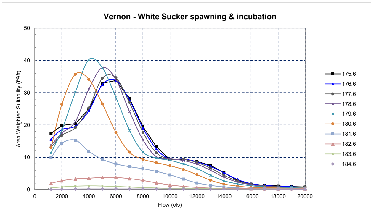
Figure 6.3.2-8. AWS curves for White Sucker spawning at 10 Turners Falls elevations (ft NAVD88) in the Vernon riverine reach.
