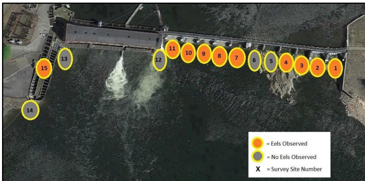
Figure 3.6-12. Vernon nighttime visual survey sites, 2017.
