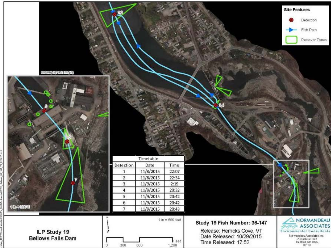
Figure 3.6-23. Example of eel wandering pattern prior to passage at Bellows Falls, 2015.
