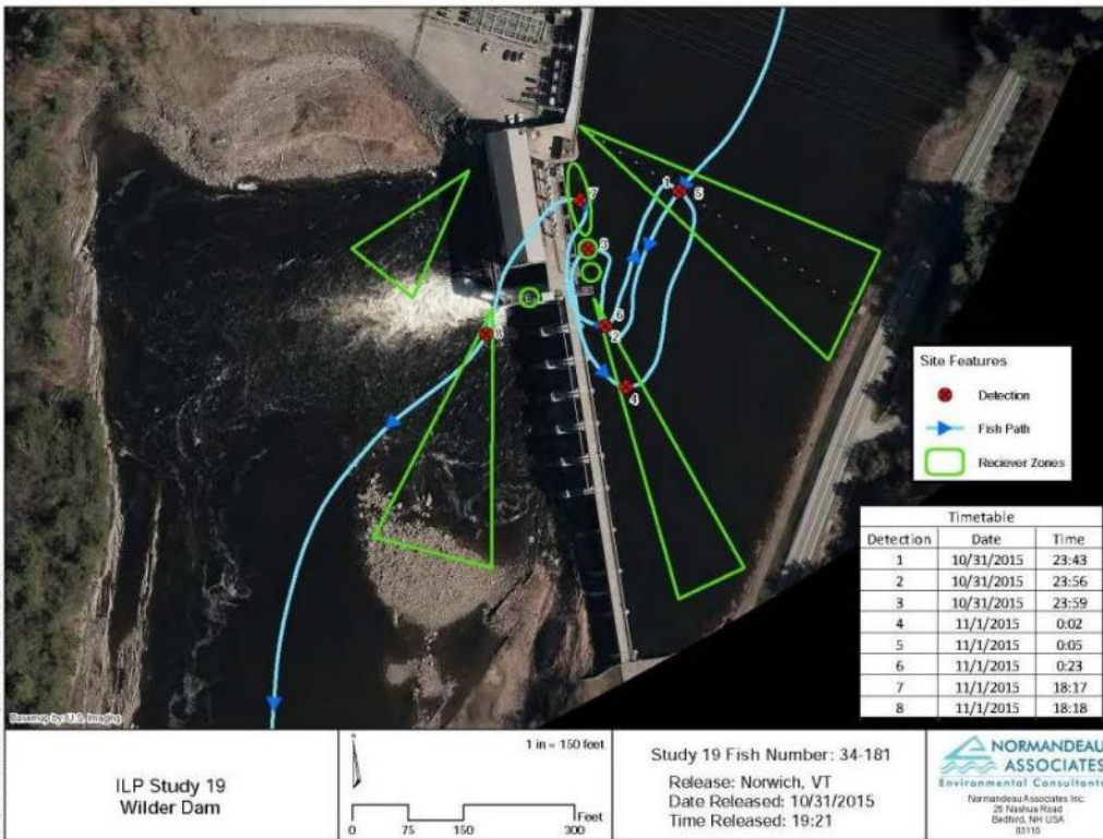
Figure 3.6-22. Example of eel wandering pattern prior to passage at Wilder, 2015.
