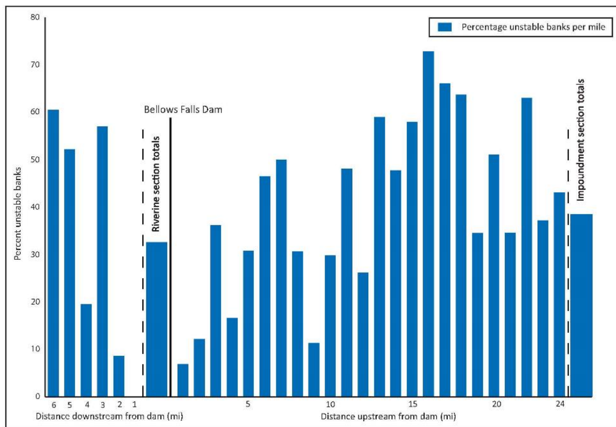
Figure 3.4-14. Variation in amounts of erosion with distance from Bellows Falls dam.
