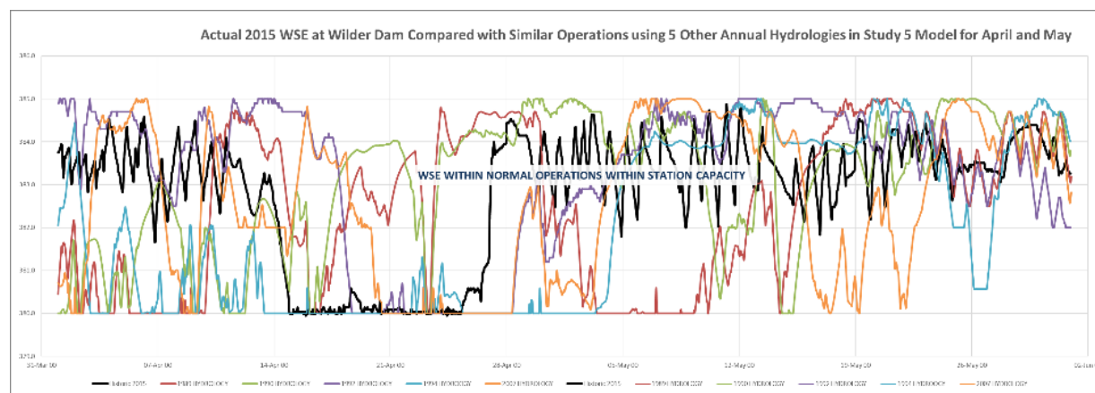
Figure 3.6-8. Comparison of 2015 actual and Study 5 modeled water surface elevations at Wilder dam.
